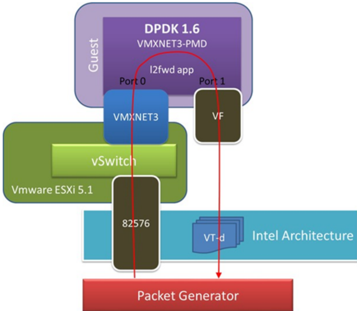
Fig. 17.2: VMXNET3 with a Native NIC Connected to a vSwitch
