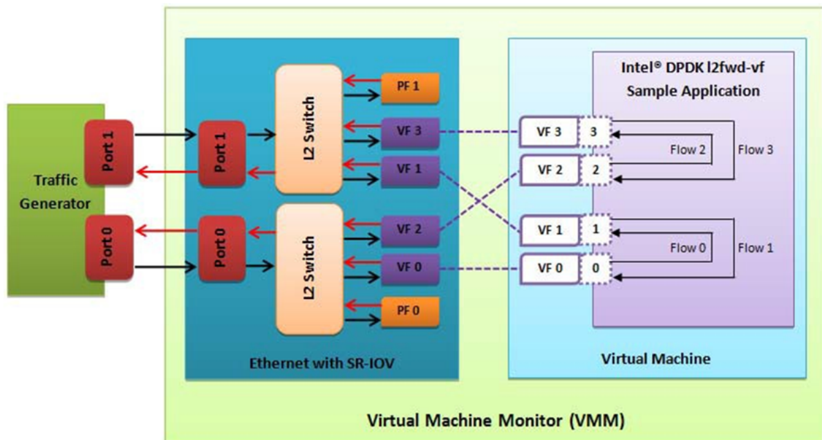
Fig. 10.2: Performance Benchmark Setup
