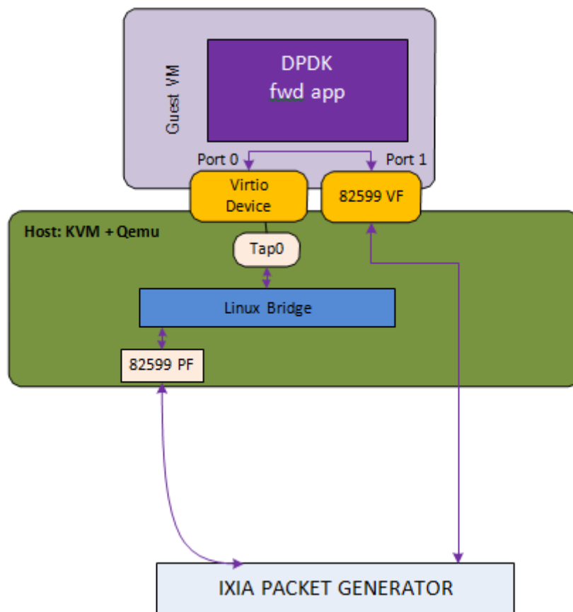
Fig. 15.3: Host2VM Communication Example Using qemu vhost Back End
