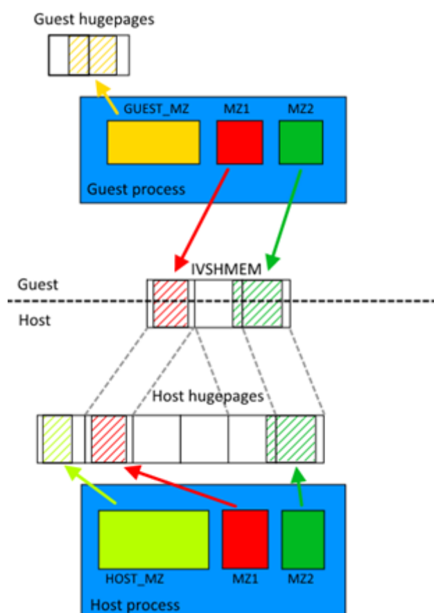
Fig. 9.1: Typical Ivshmem use case
