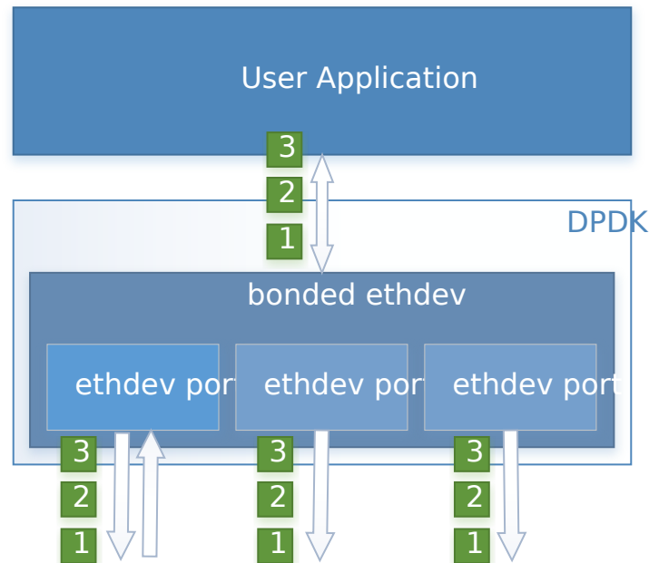
Fig. 10.5: Broadcast (Mode 3)
