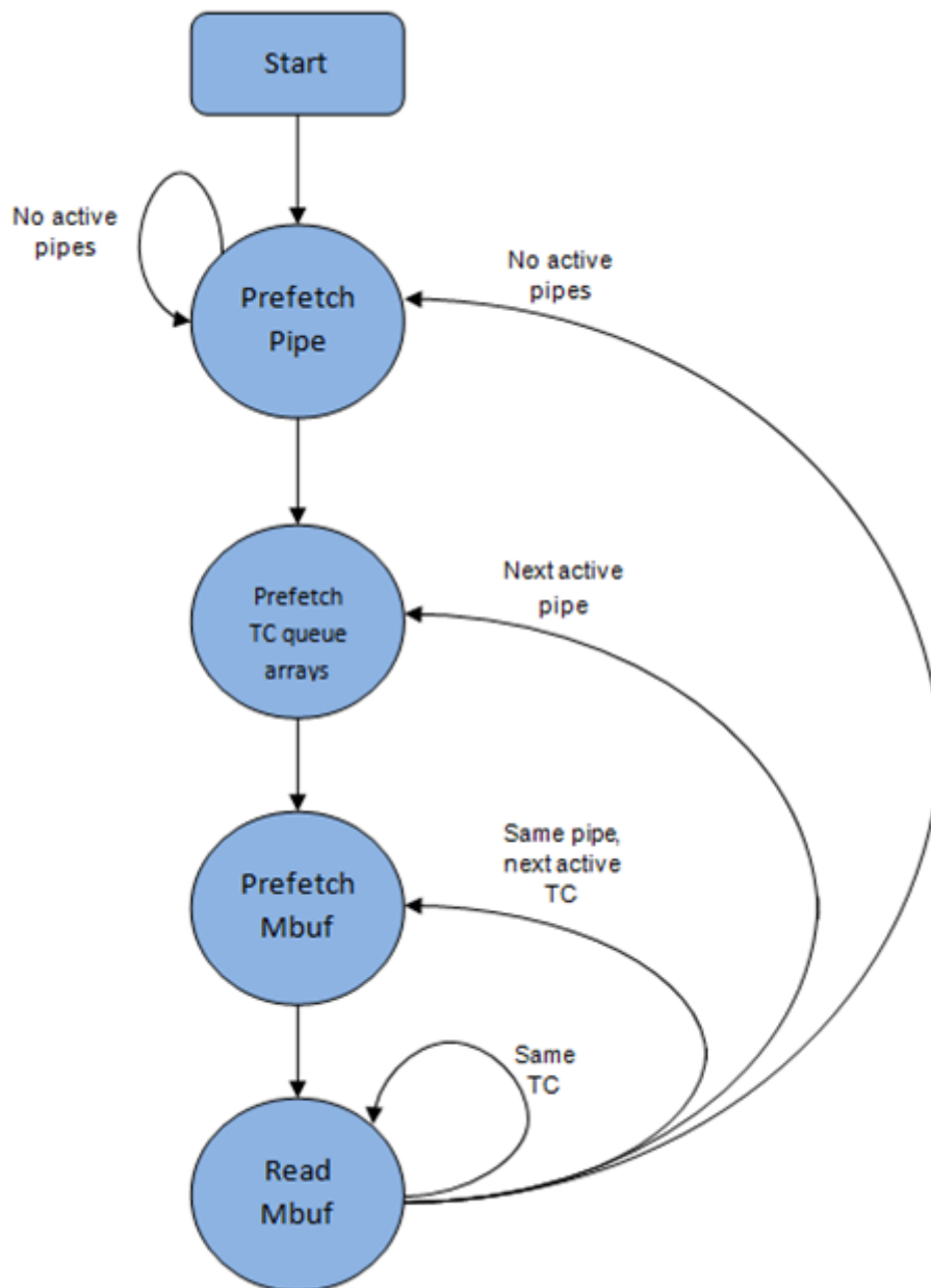
Fig. 21.6: Pipe Prefetch State Machine for the Hierarchical Scheduler Dequeue Operation
