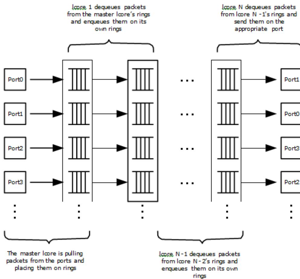
Fig. 27.1: Pipeline Overview
