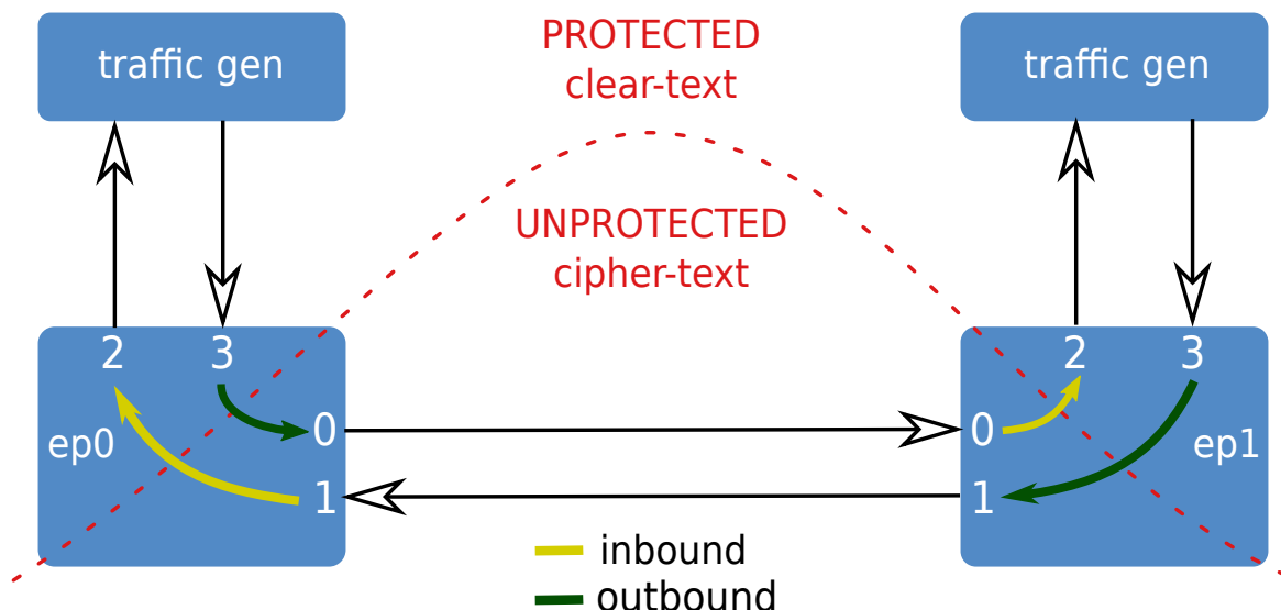
Fig. 41.1: IPsec Inbound/Outbound traffic
