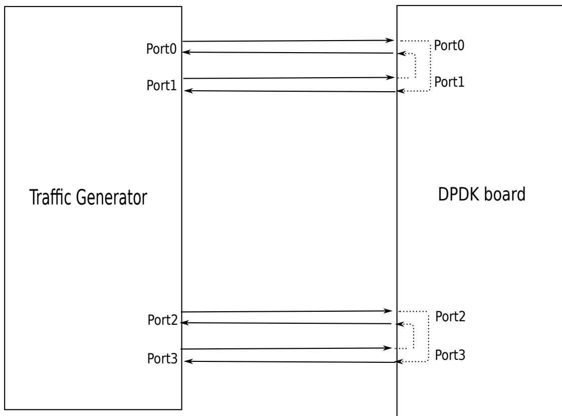
Fig. 35.1: Performance Benchmarking Setup (Basic Environment)
