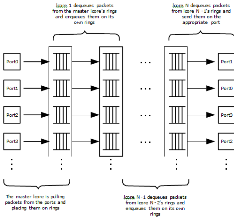
Fig. 27.1: Pipeline Overview
