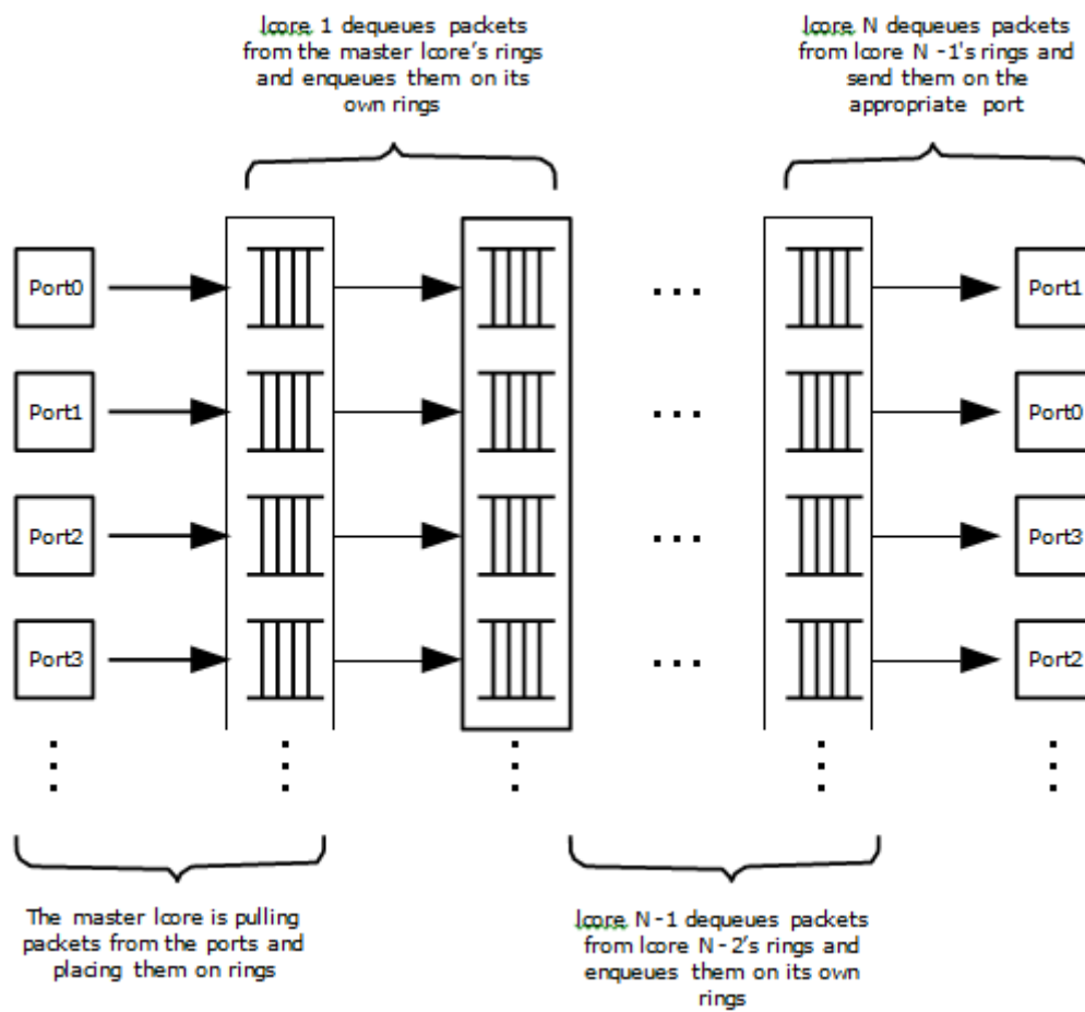
Fig. 28.1: Pipeline Overview
