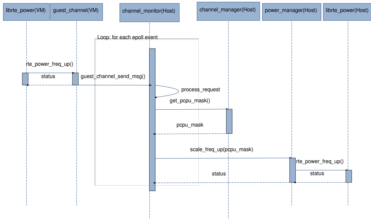
Fig. 37.2: VM request to scale frequency
