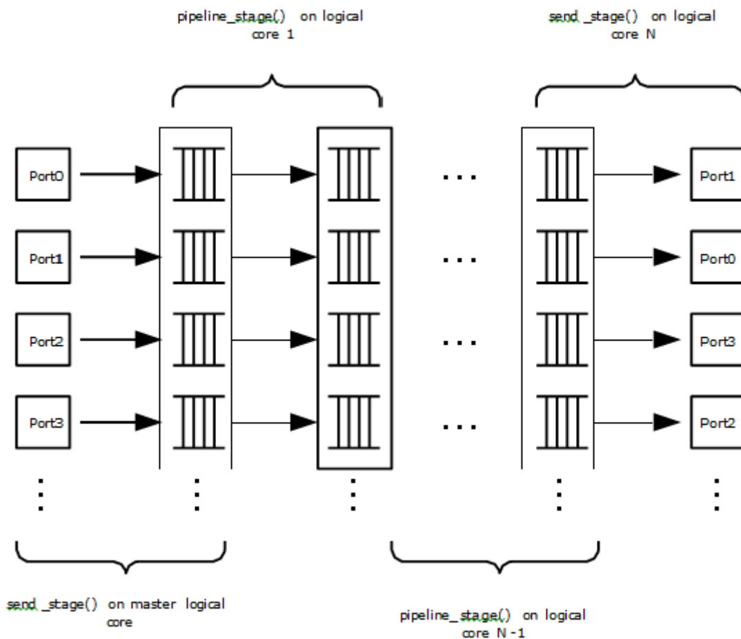
Fig. 28.3: Threads and Pipelines
