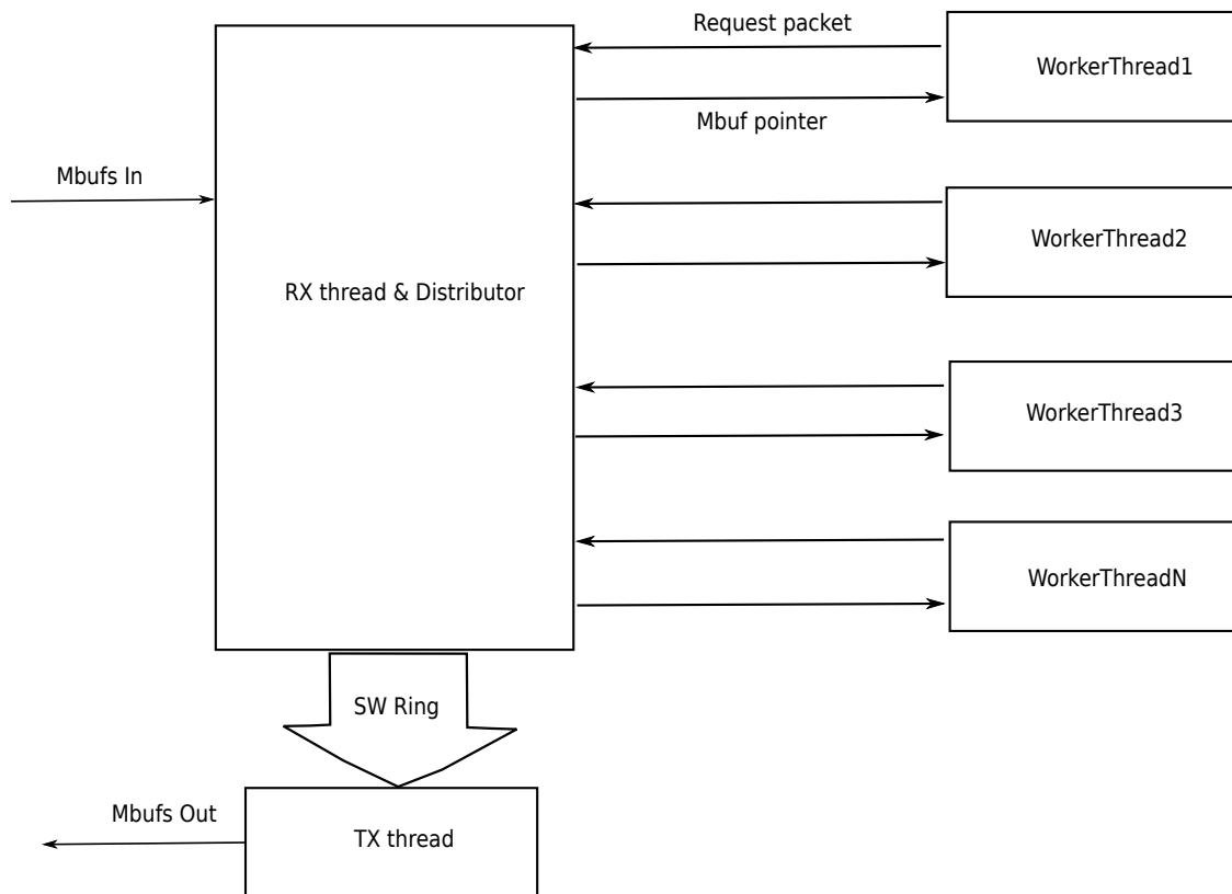
Fig. 36.2: Distributor Sample Application Layout
