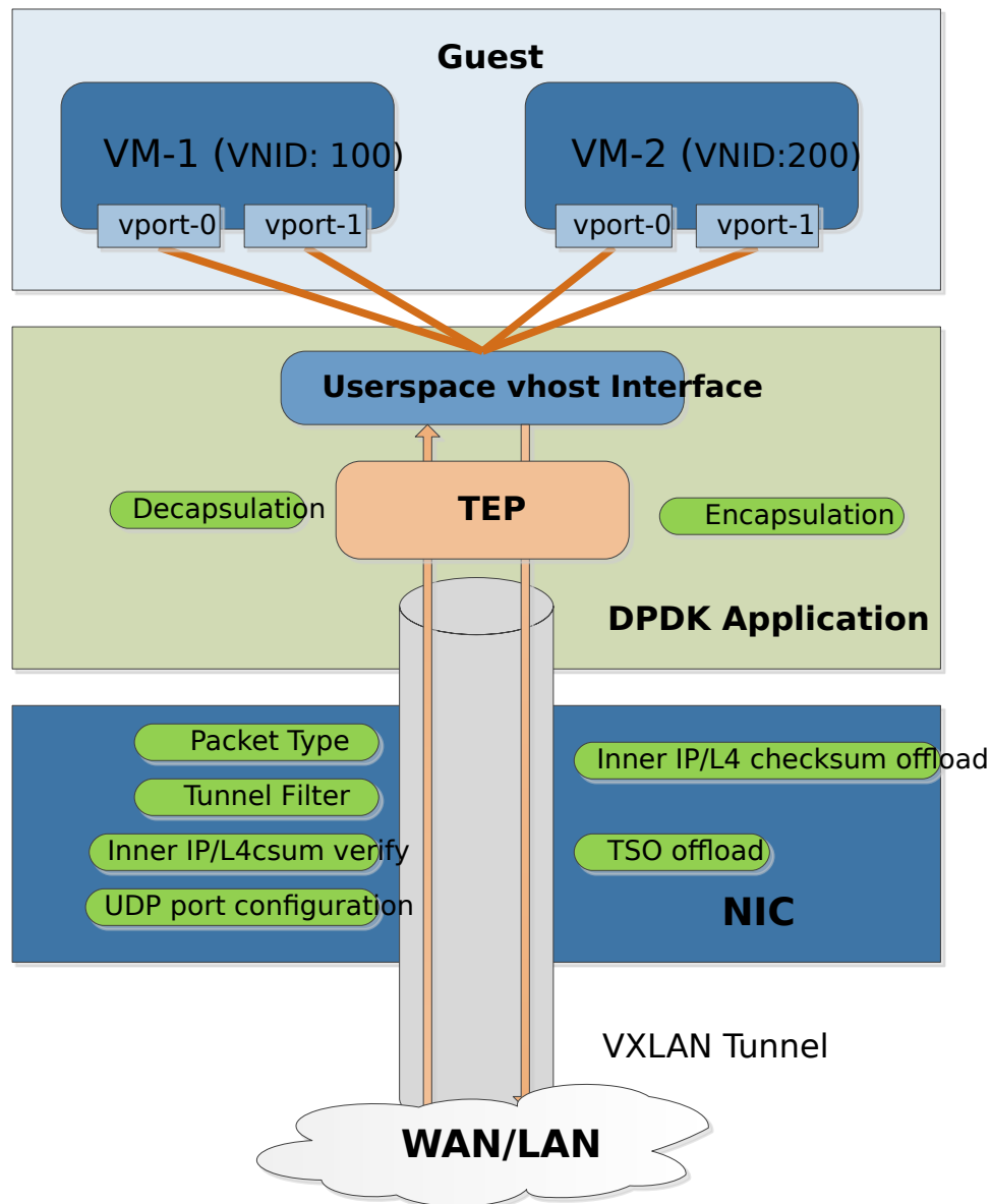
Fig. 38.2: TEP termination Framework Overview
