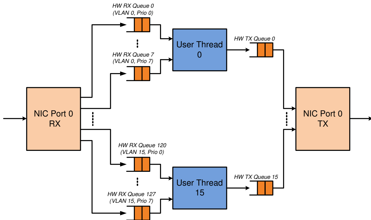
Fig. 31.1: Packet Flow Through the VMDQ and DCB Sample Application
