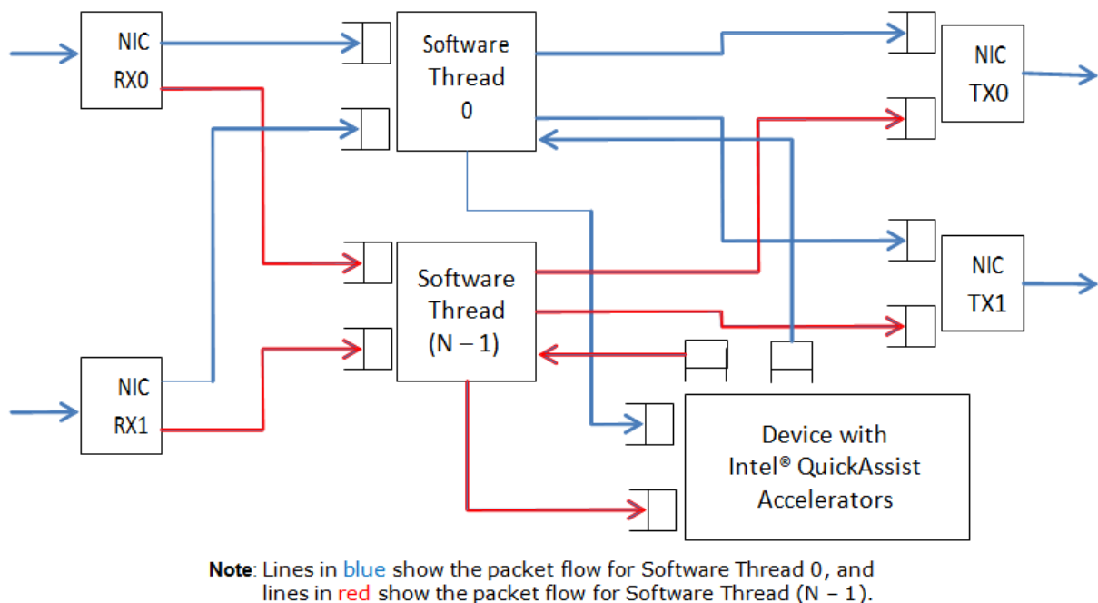
Fig. 27.1: Intel® QuickAssist Technology Application Block Diagram
