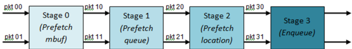
Fig. 27.5: Prefetch Pipeline for the Hierarchical Scheduler Enqueue Operation
