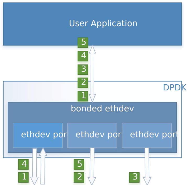
Fig. 12.2: Round-Robin (Mode 0)
