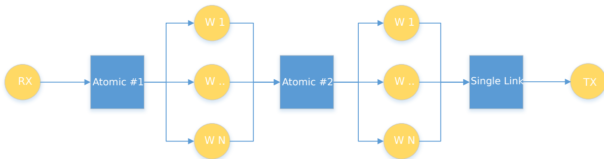
Fig. 26.1: Sample eventdev usage, with RX, two atomic stages and a single-link to TX.
