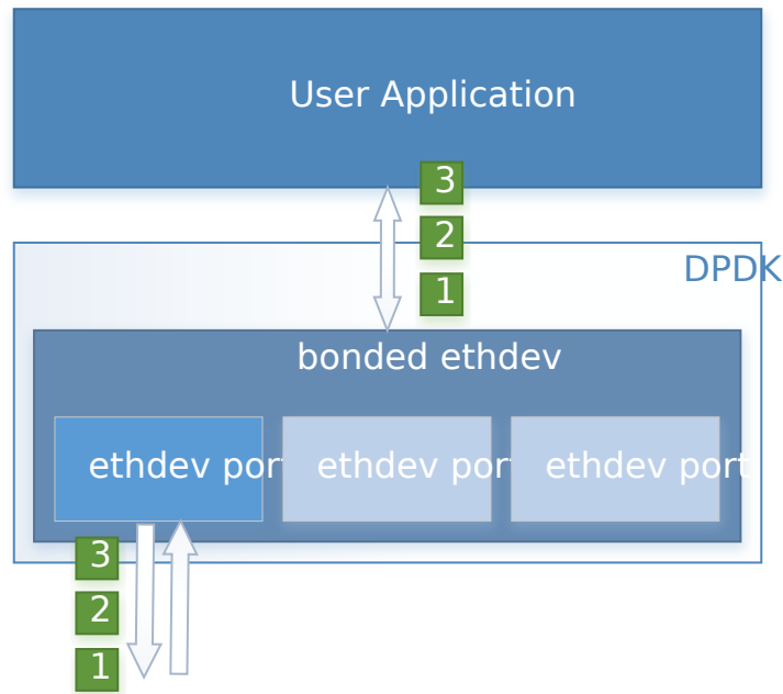
Fig. 12.3: Active Backup (Mode 1)
