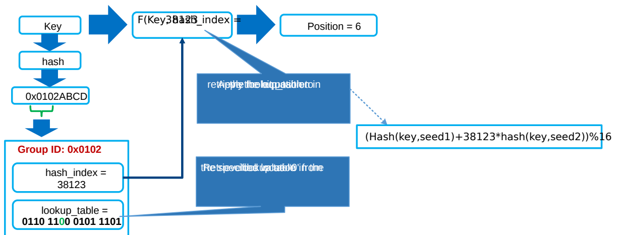
Fig. 15.11: EFD Lookup Operation
