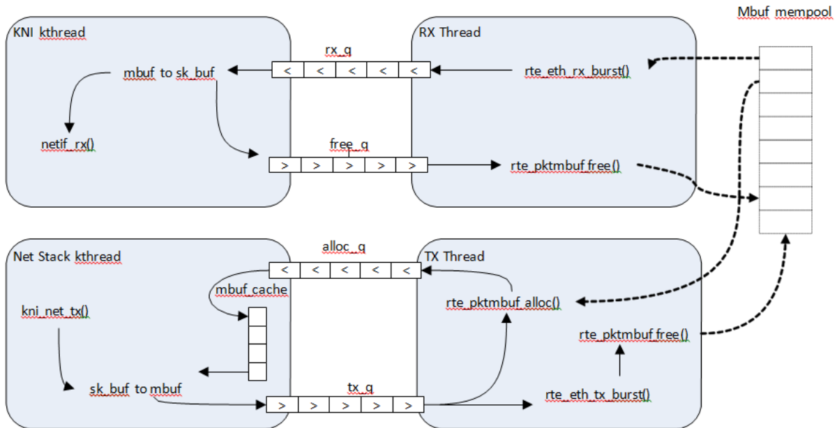
Fig. 24.2: Packet Flow via mbufs in the DPDK KNI
