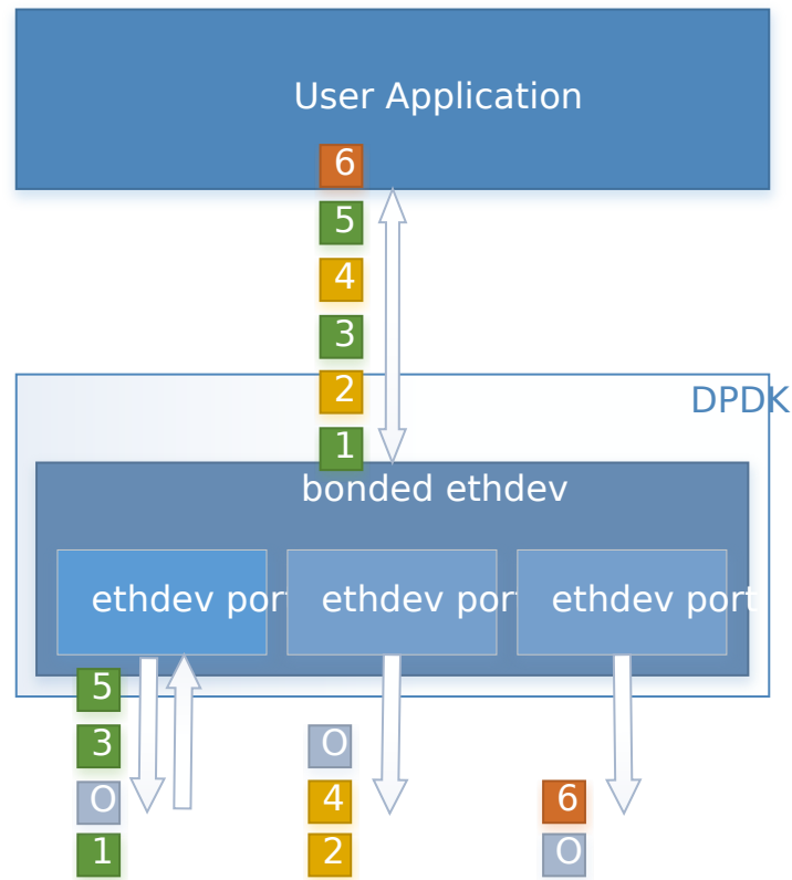
Fig. 12.6: Link Aggregation 802.3AD (Mode 4)
