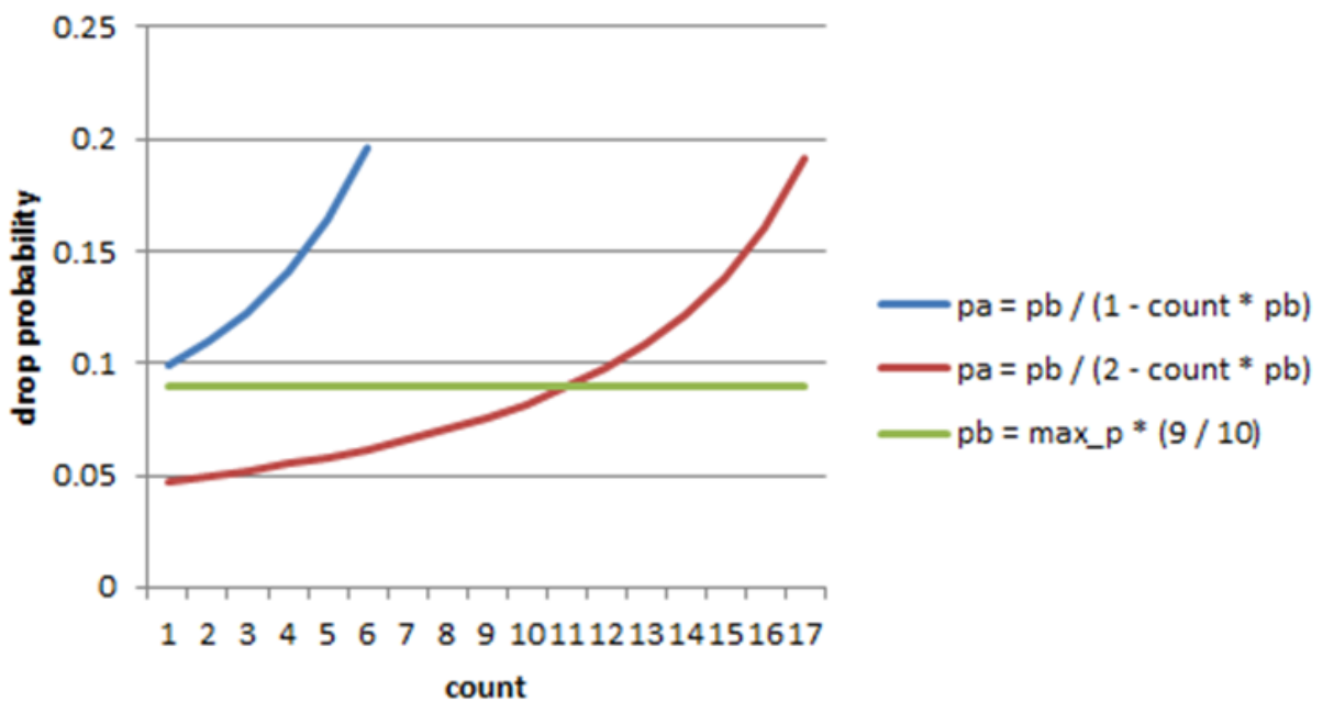
Fig. 27.11: Initial Drop Probability (pb), Actual Drop probability (pa) Computed Using a Factor 1 (Blue Curve) and a Factor 2 (Red Curve)
