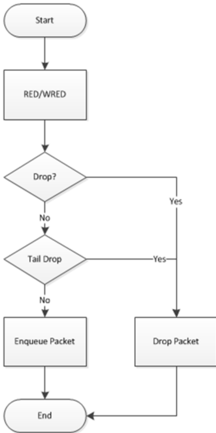
Fig. 27.8: Flow Through the Dropper
