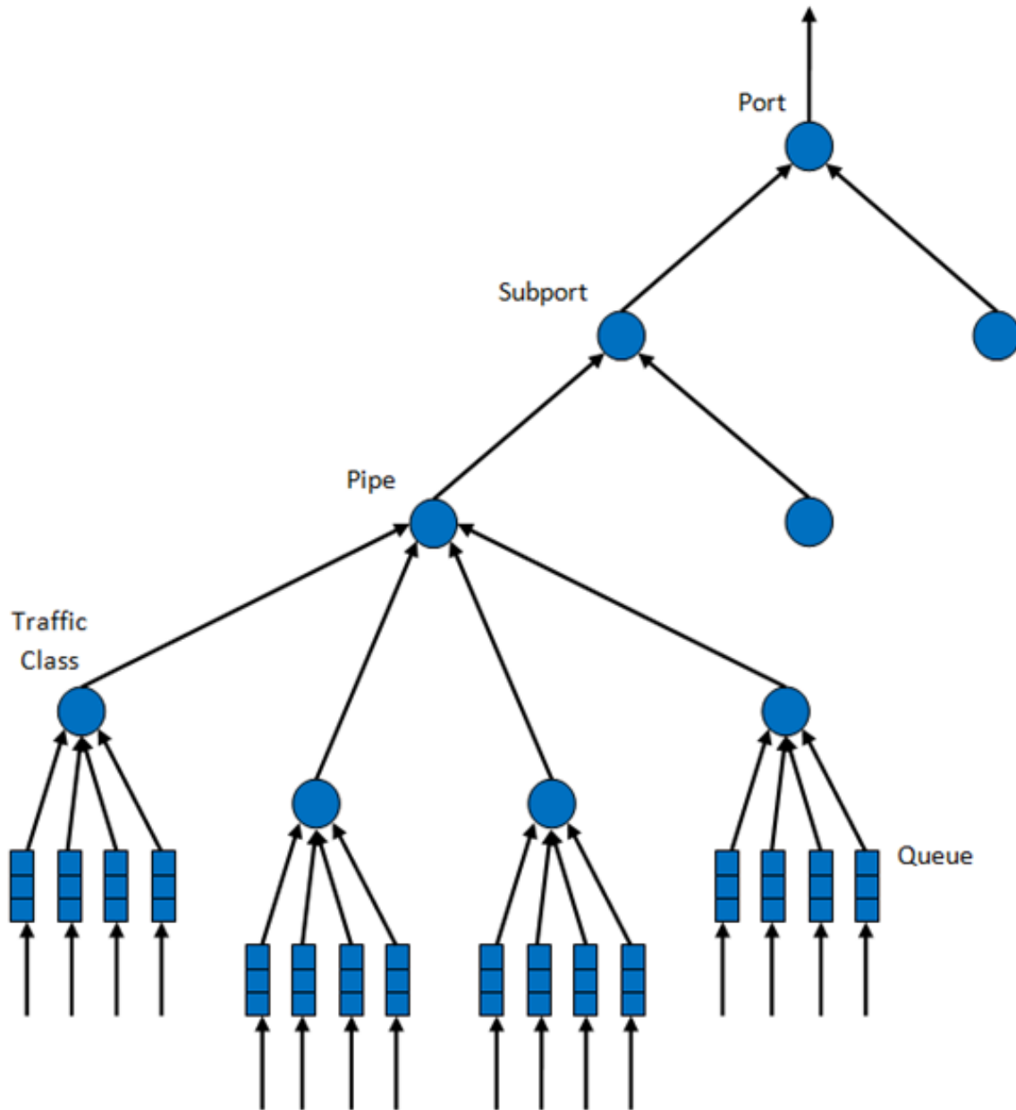
Fig. 27.3: Scheduling Hierarchy per Port
