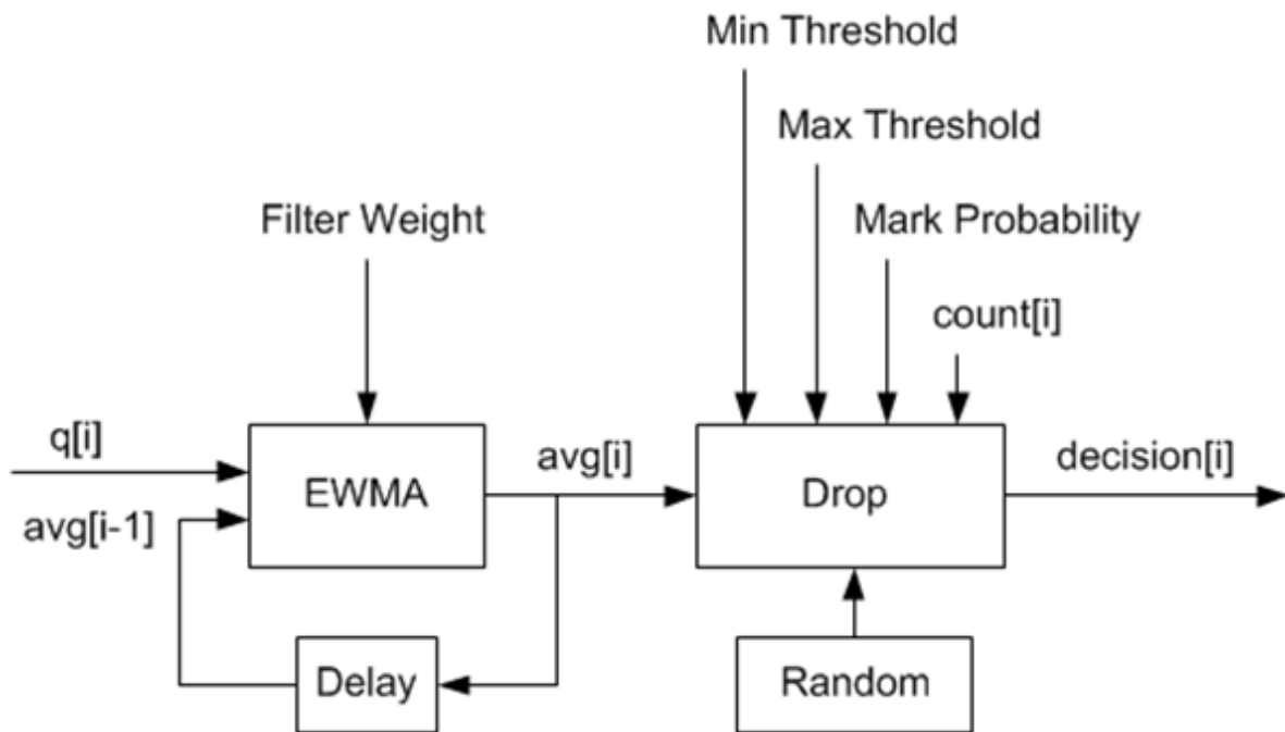
Fig. 27.9: Example Data Flow Through Dropper
