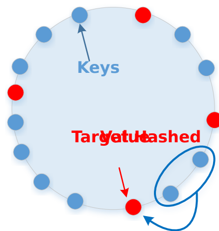
Fig. 15.2: Consistent Hashing
