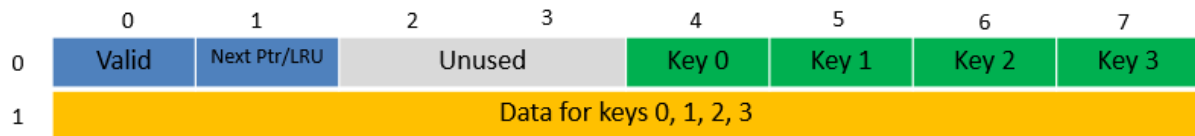
Fig. 30.5: Data Structures for 8-byte Key Hash Tables
