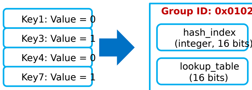
Fig. 15.8: Perfect Hash Search - Assigned Keys & Target Value
