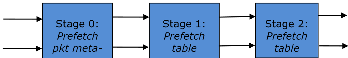
Fig. 30.7: Bucket Search Pipeline for Key Lookup Operation (Single Key Size Hash Tables)
