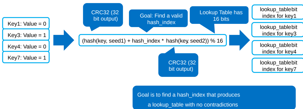
Fig. 15.9: Perfect Hash Search - Satisfy Target Values
