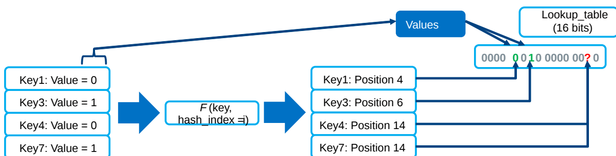
Fig. 15.10: Finding Hash Index for Conflict Free lookup_table
