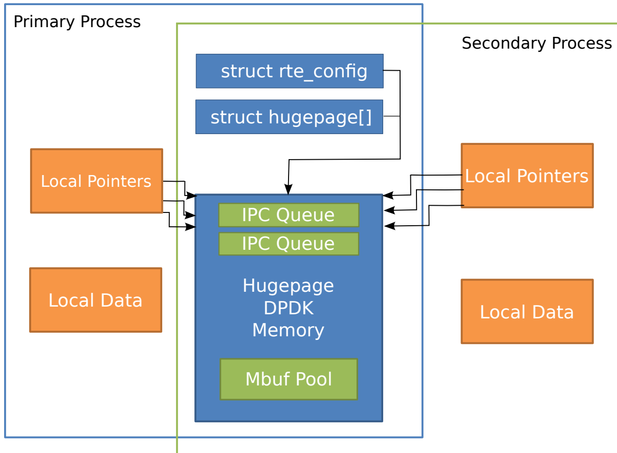
Fig. 23.1: Memory Sharing in the DPDK Multi-process Sample Application
