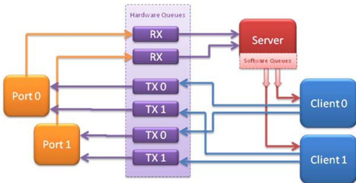
Fig. 24.2: Example Data Flow in a Client-Server Symmetric Multi-process Application
