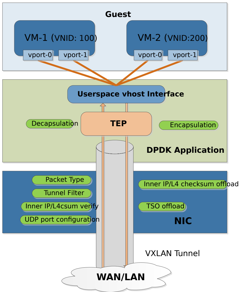
Fig. 39.2: TEP termination Framework Overview
