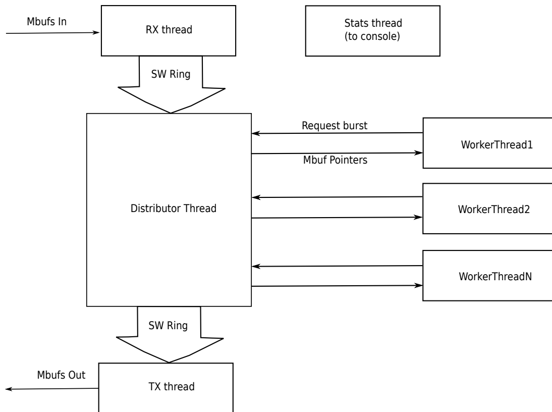
Fig. 37.2: Distributor Sample Application Layout
