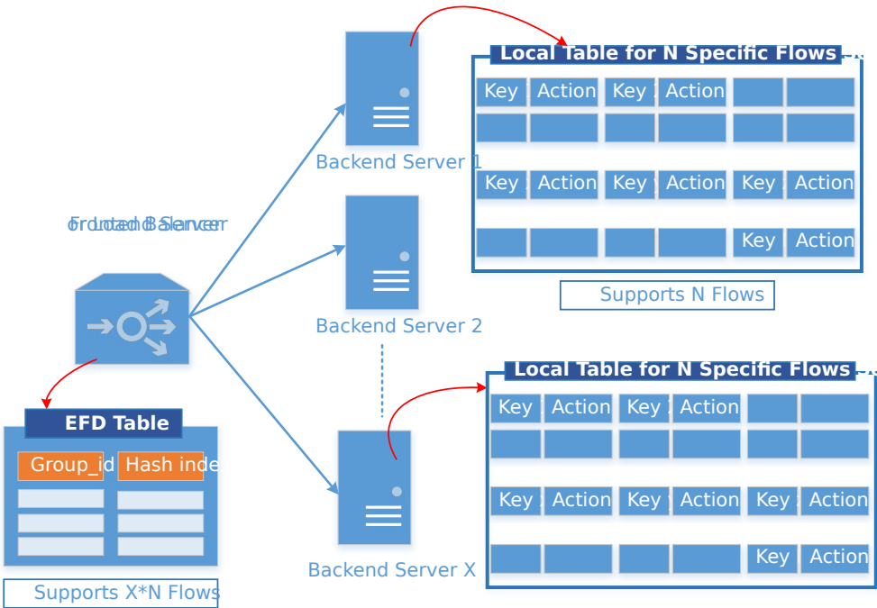
Fig. 23.1: Using EFD as a Flow-Level Load Balancer
