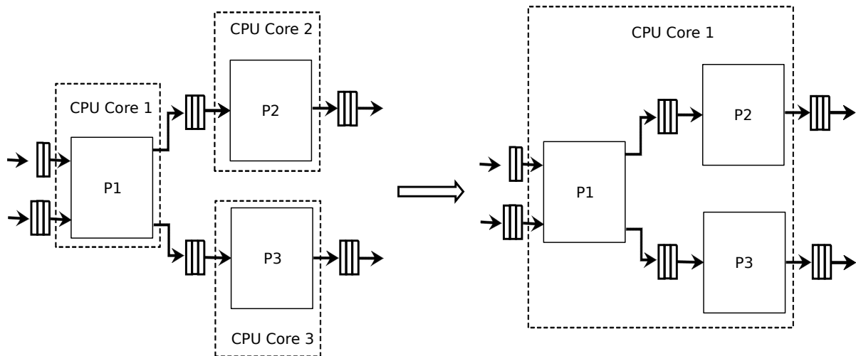
Fig. 34.1: Example of moving pipeline instances across different CPU cores
