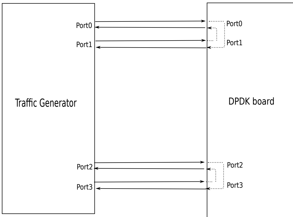
Fig. 37.1: Performance Benchmarking Setup (Basic Environment)
