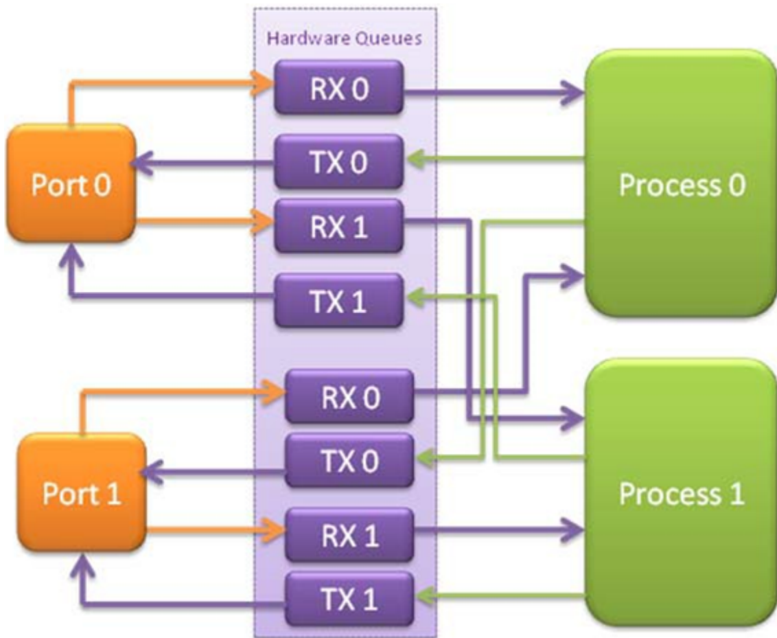
Fig. 24.1: Example Data Flow in a Symmetric Multi-process Application
