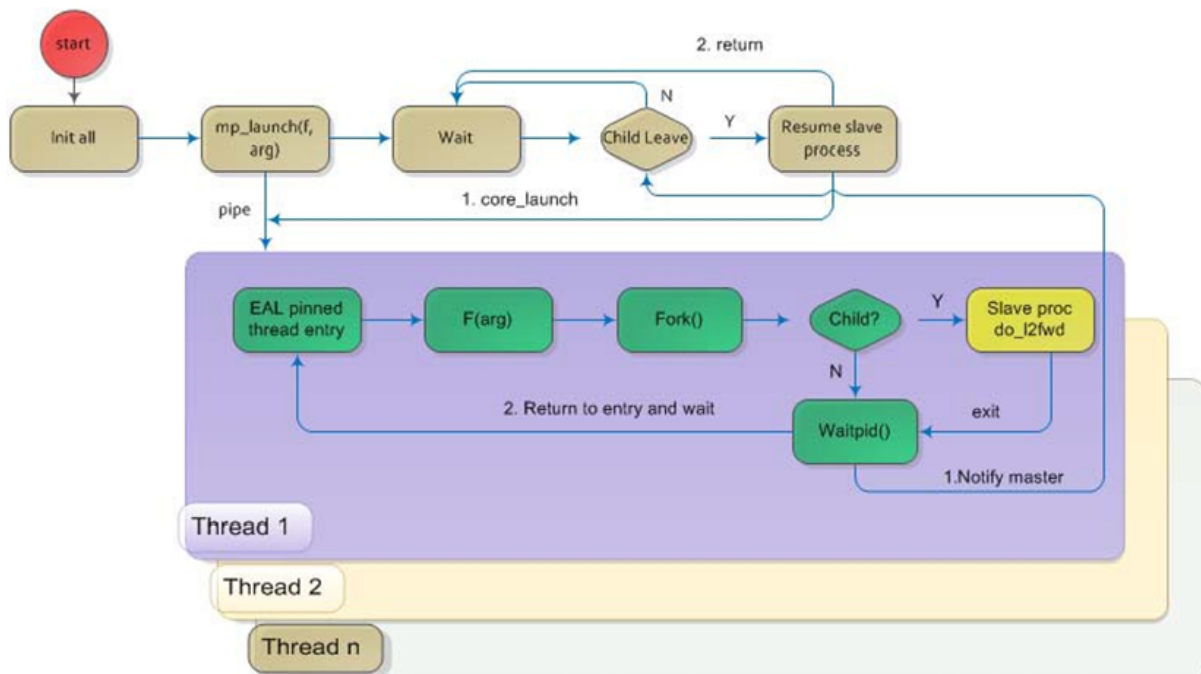
Fig. 24.3: Master-slave Process Workflow
