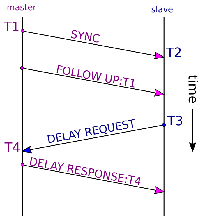
Fig. 40.1: PTP Synchronization Protocol
