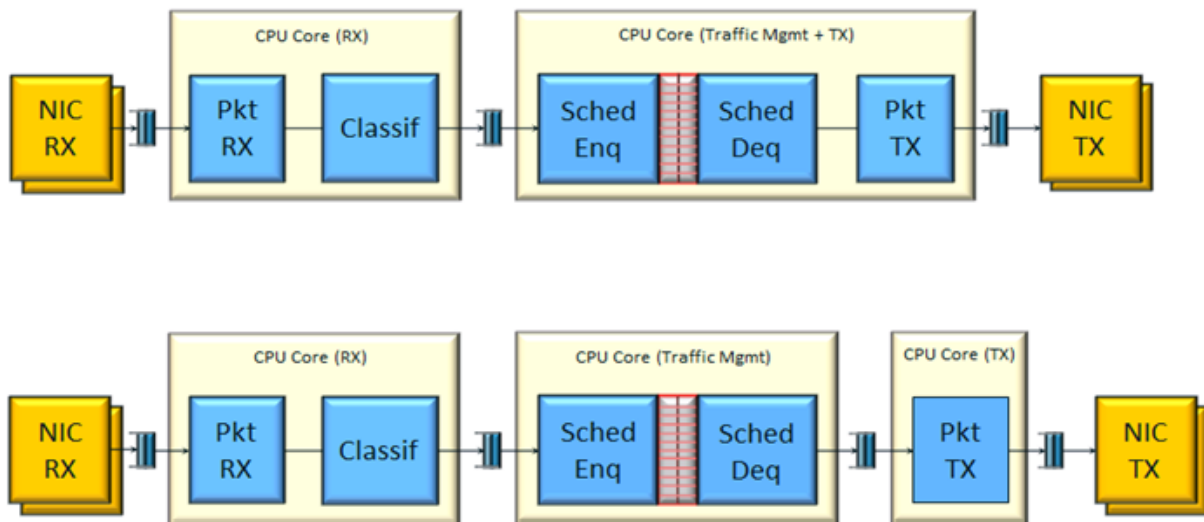
Fig. 26.1: QoS Scheduler Application Architecture
