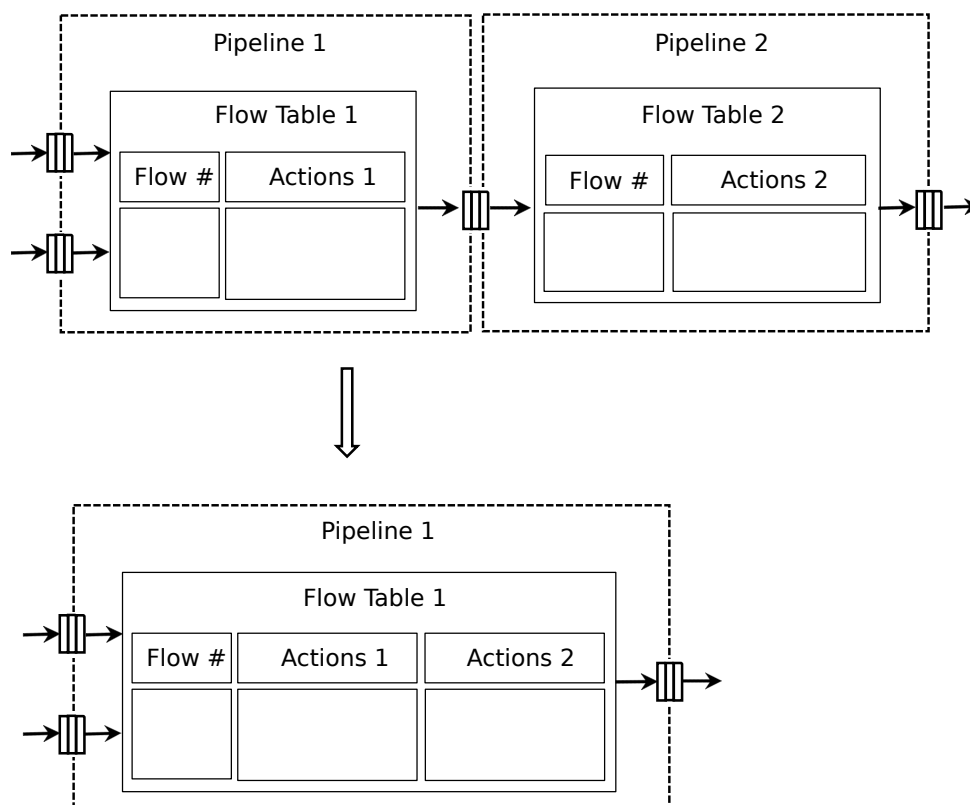
Fig. 34.3: Example of moving actions across different tables and pipeline instances
