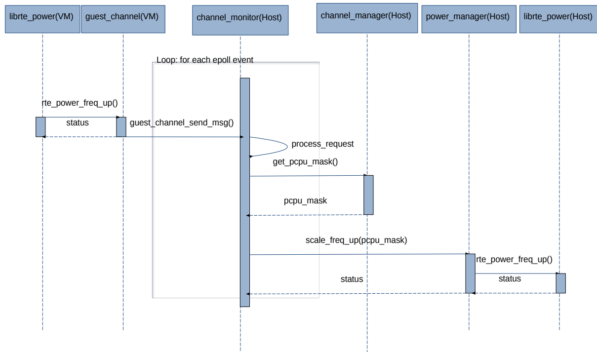
Fig. 38.2: VM request to scale frequency
