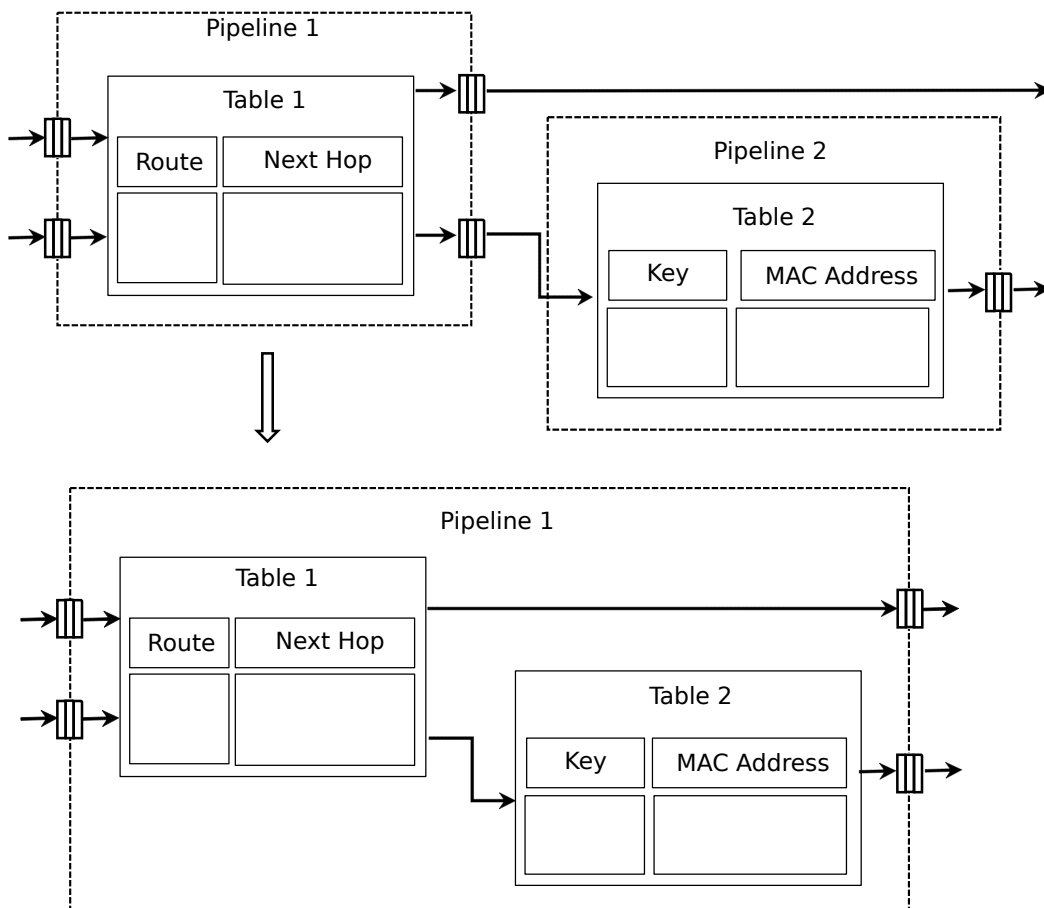
Fig. 34.2: Example of moving tables across different pipeline instances
