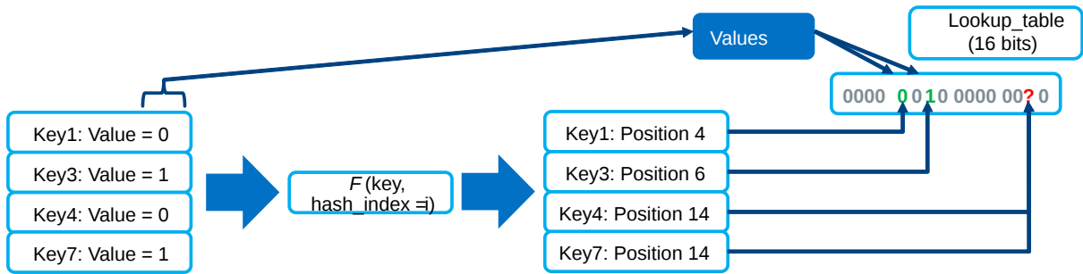
Fig. 17.10: Finding Hash Index for Conflict Free lookup_table
