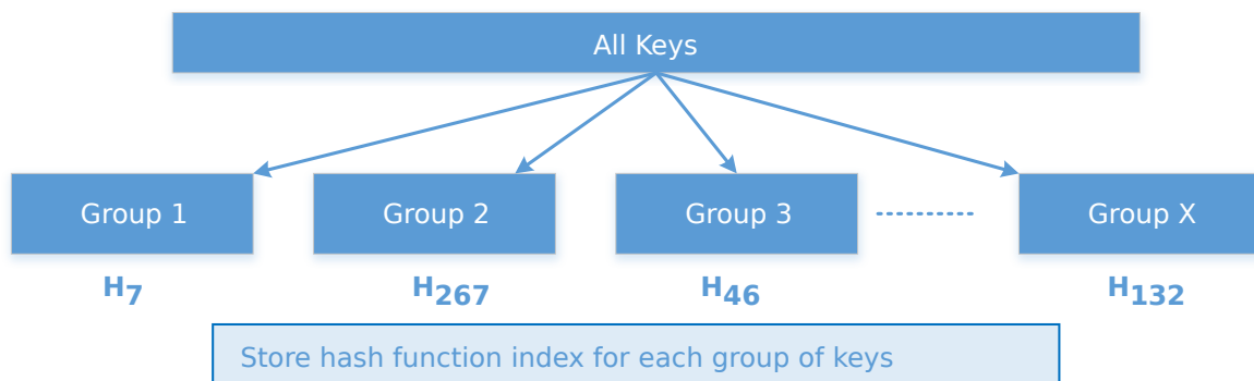
Fig. 17.5: Divide and Conquer for Millions of Keys
