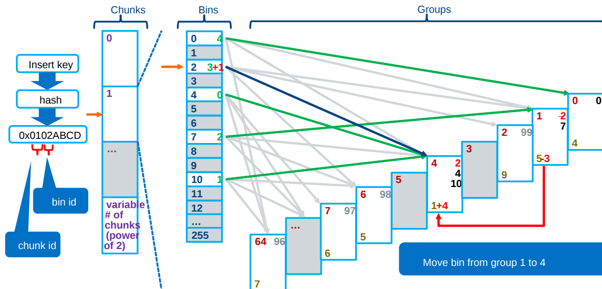
Fig. 17.12: Runtime Group Rebalancing
