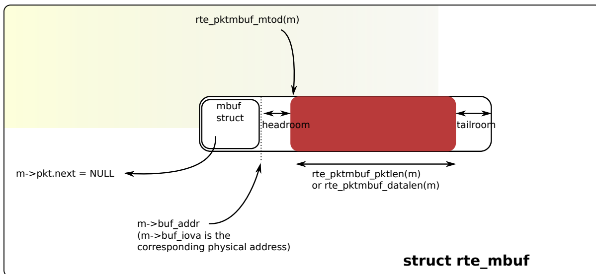
Fig. 7.1: An mbuf with One Segment
