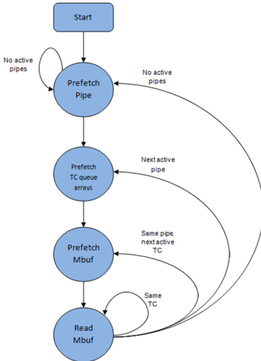
Fig. 33.6: Pipe Prefetch State Machine for the Hierarchical Scheduler Dequeue Operation
