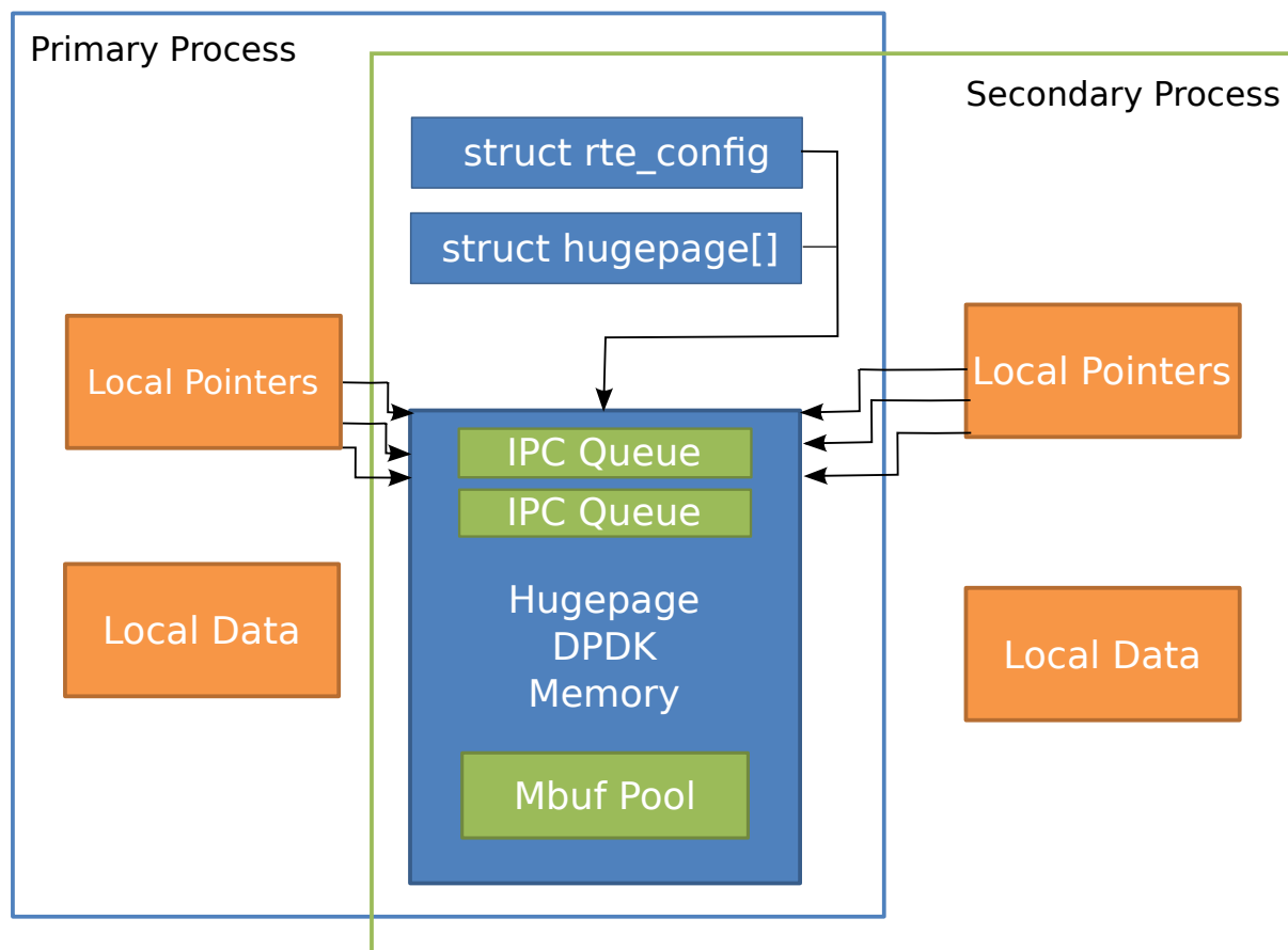
Fig. 28.1: Memory Sharing in the DPDK Multi-process Sample Application
