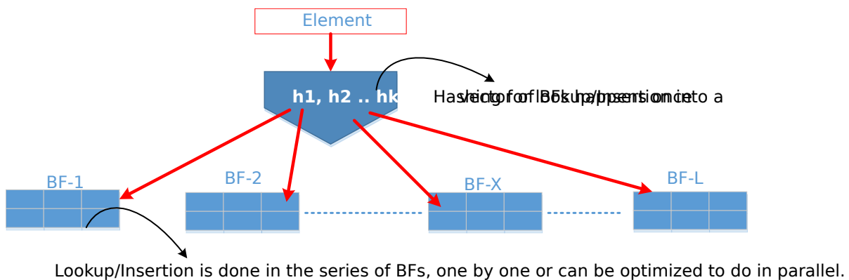
Fig. 18.4: Vector Bloom Filter (vBF) Overview
