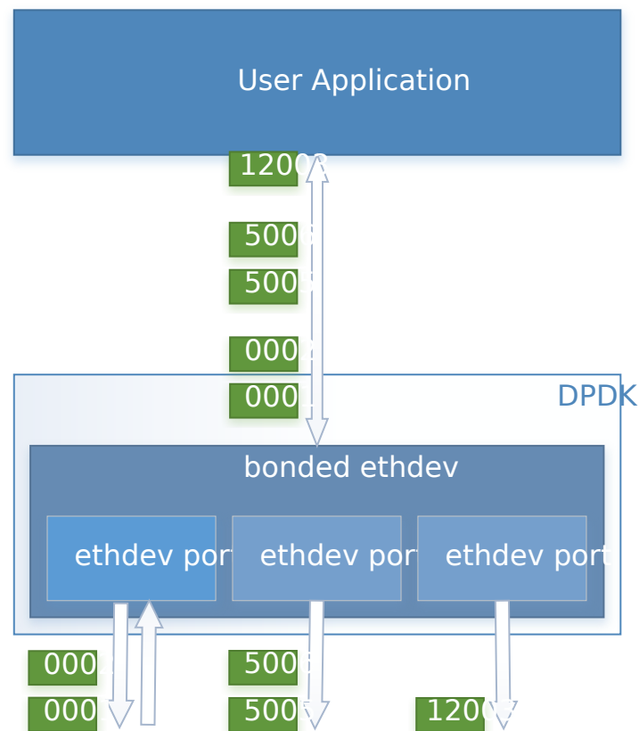
Fig. 14.7: Transmit Load Balancing (Mode 5)
