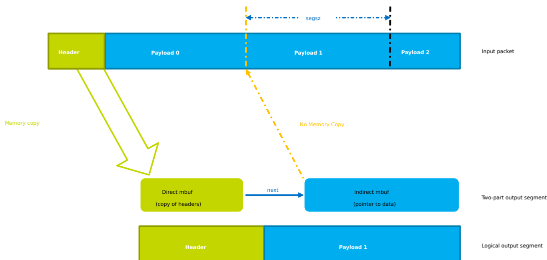
Fig. 26.1: Two-part GSO output segment
