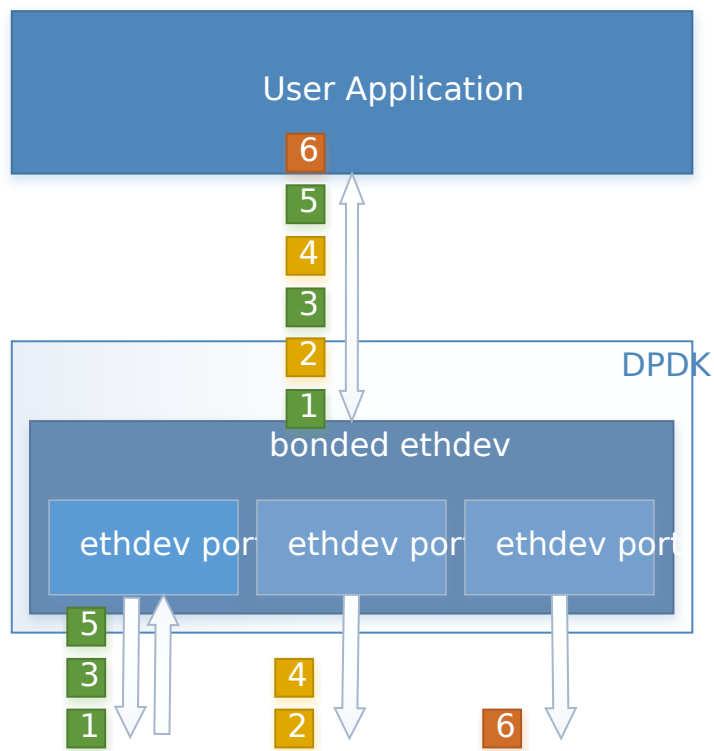
Fig. 14.4: Balance XOR (Mode 2)
