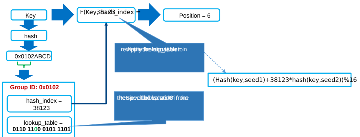
Fig. 17.11: EFD Lookup Operation
