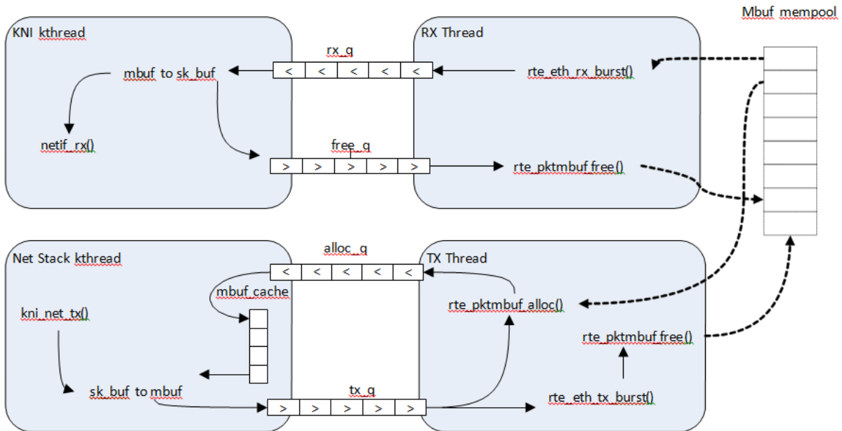
Fig. 29.2: Packet Flow via mbufs in the DPDK KNI
