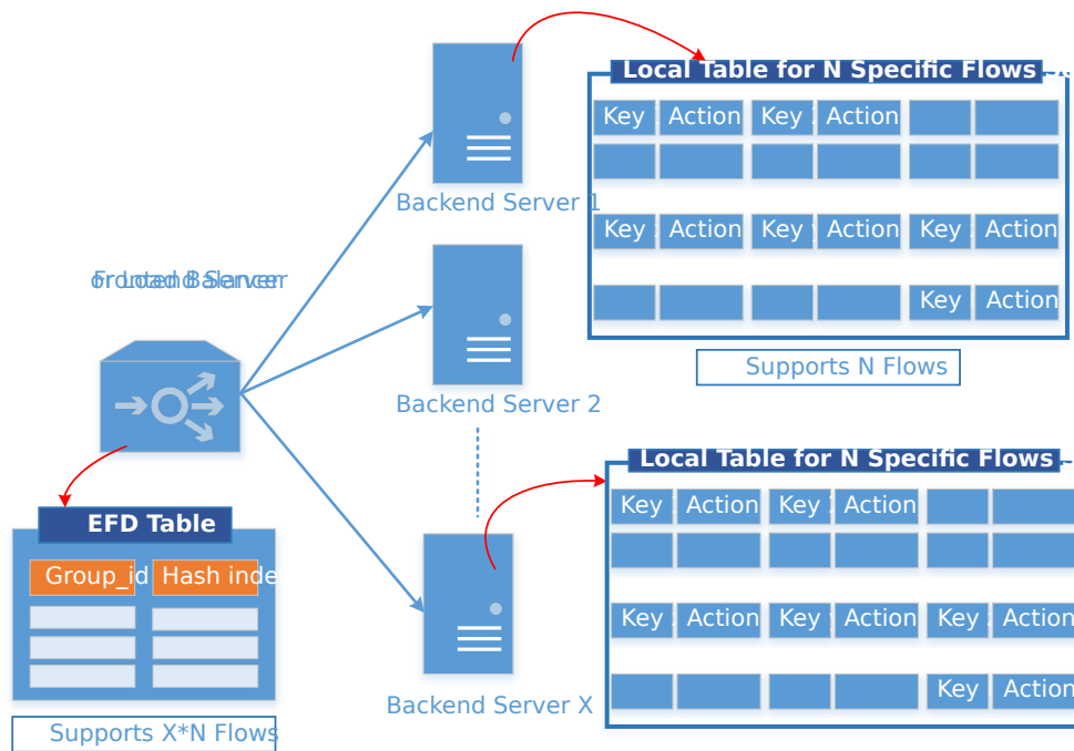
Fig. 17.6: EFD as a Flow-Level Load Balancer
