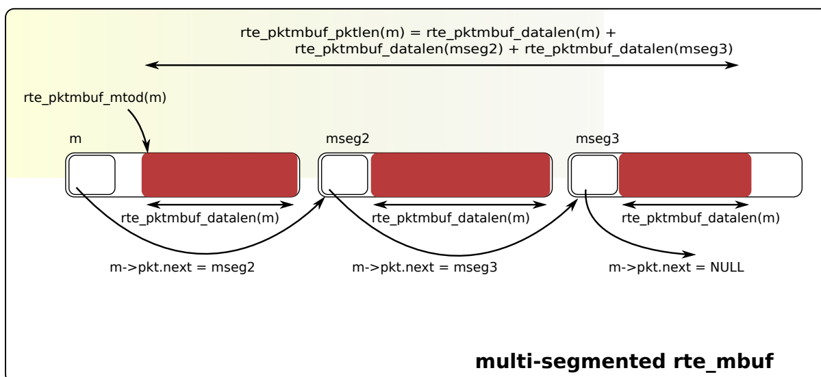
Fig. 7.2: An mbuf with Three Segments
