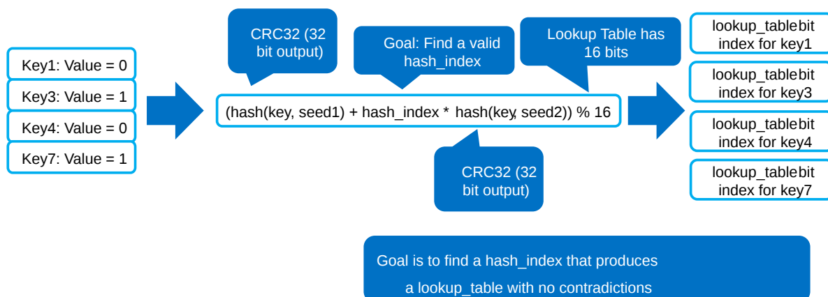
Fig. 17.9: Perfect Hash Search - Satisfy Target Values
