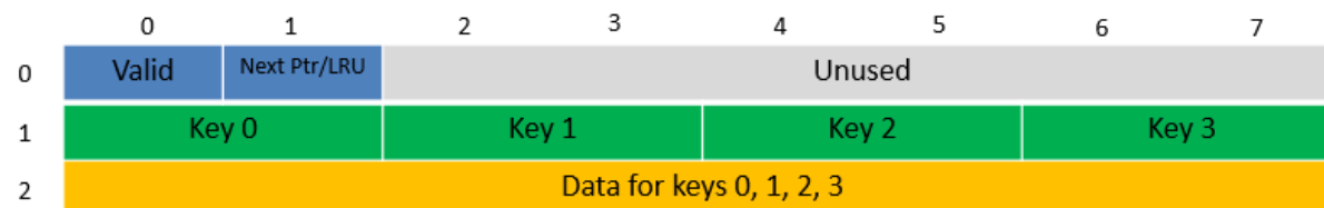
Fig. 36.6: Data Structures for 16-byte Key Hash Tables
