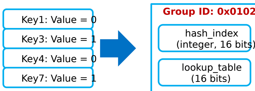
Fig. 17.8: Perfect Hash Search - Assigned Keys & Target Value
