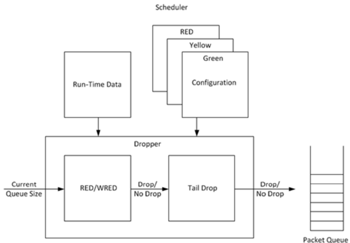
Fig. 33.7: High-level Block Diagram of the DPDK Dropper
