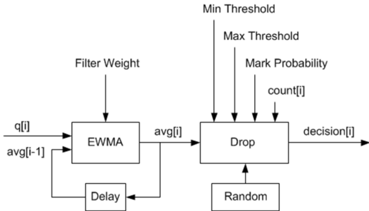
Fig. 33.9: Example Data Flow Through Dropper
