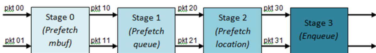
Fig. 33.5: Prefetch Pipeline for the Hierarchical Scheduler Enqueue Operation
