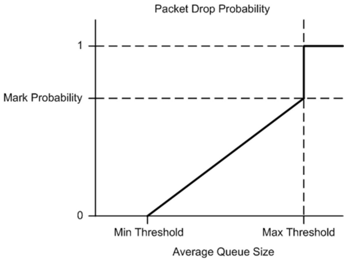
Fig. 33.10: Packet Drop Probability for a Given RED Configuration
