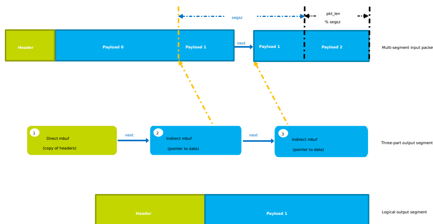
Fig. 26.2: Three-part GSO output segment
