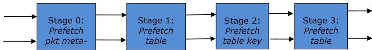
Fig. 36.4: Bucket Search Pipeline for Key Lookup Operation (Configurable Key Size Hash Tables)
