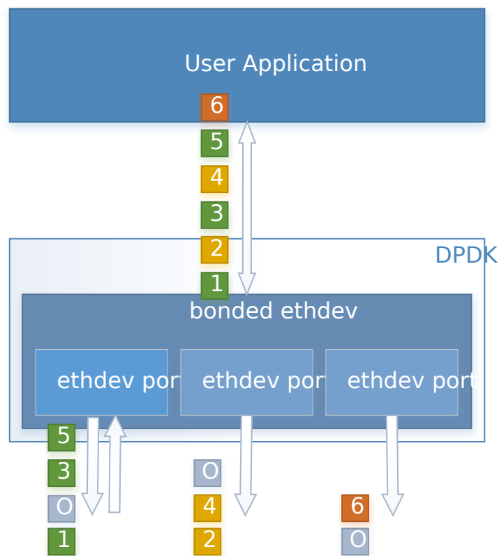
Fig. 14.6: Link Aggregation 802.3AD (Mode 4)
