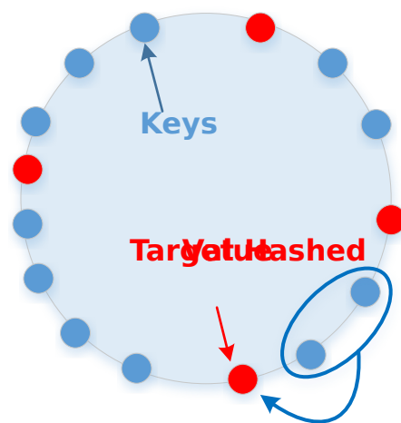
Fig. 17.2: Consistent Hashing
