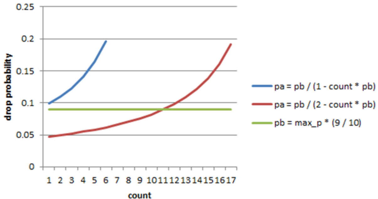
Fig. 33.11: Initial Drop Probability (pb), Actual Drop probability (pa) Computed Using a Factor 1 (Blue Curve) and a Factor 2 (Red Curve)
