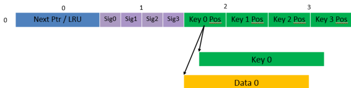
Fig. 36.3: Data Structures for Configurable Key Size Hash Tables
