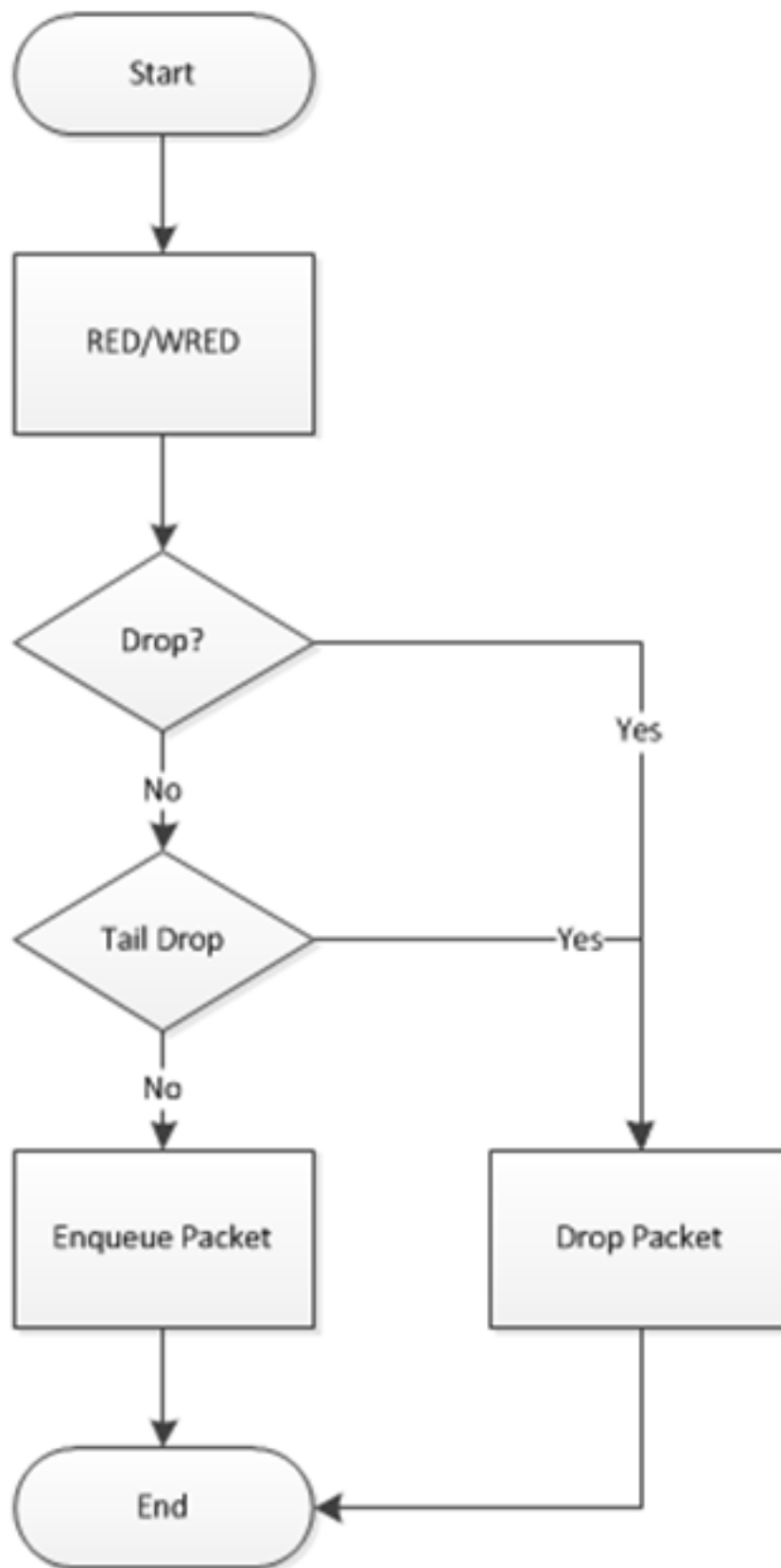
Fig. 33.8: Flow Through the Dropper
