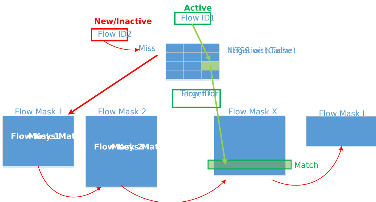
Fig. 18.7: Using HTSS with False Negatives for Wild Card Classification
