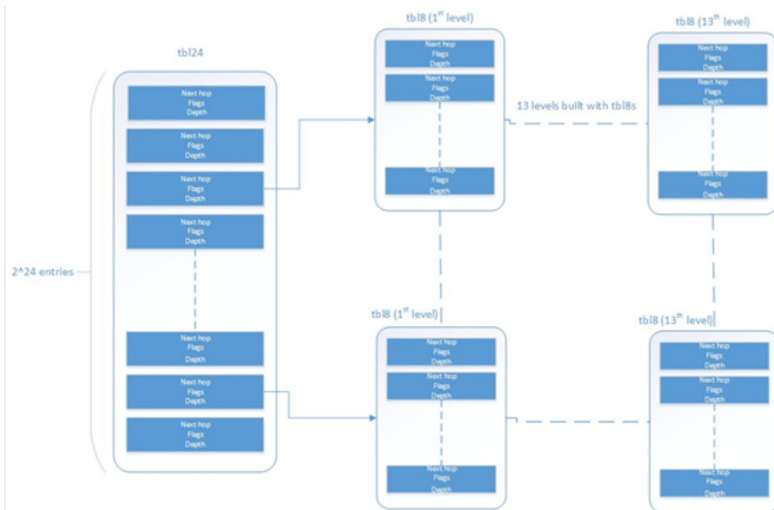
Fig. 24.1: Table split into different levels
