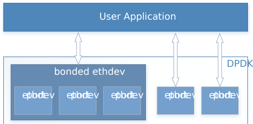
Fig. 18.1: Bonded PMDs
