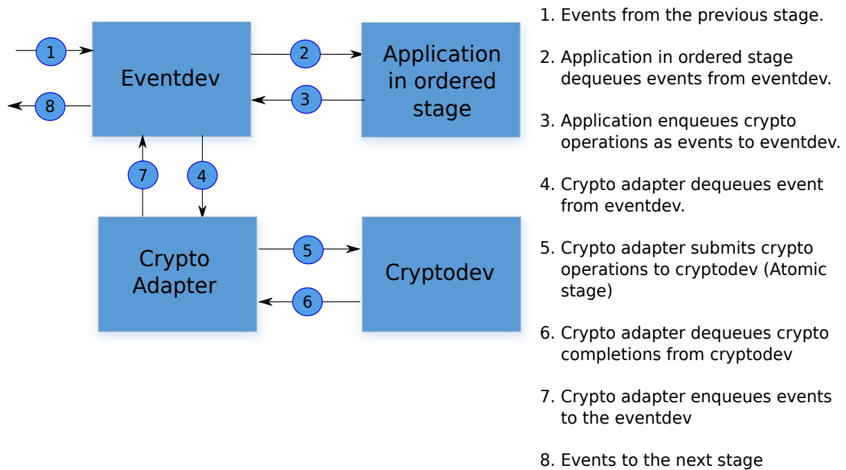
Fig. 39.2: Working model of RTE_EVENT_CRYPTODEV_ADAPTER_OP_FORWARD mode
