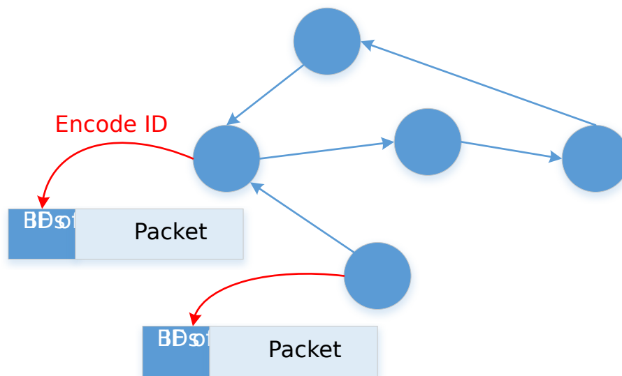
Fig. 22.3: Detecting Routing Loops Using BF
