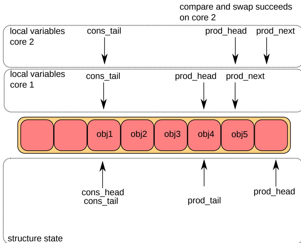
Fig. 5.10: Multiple producer enqueue third step
