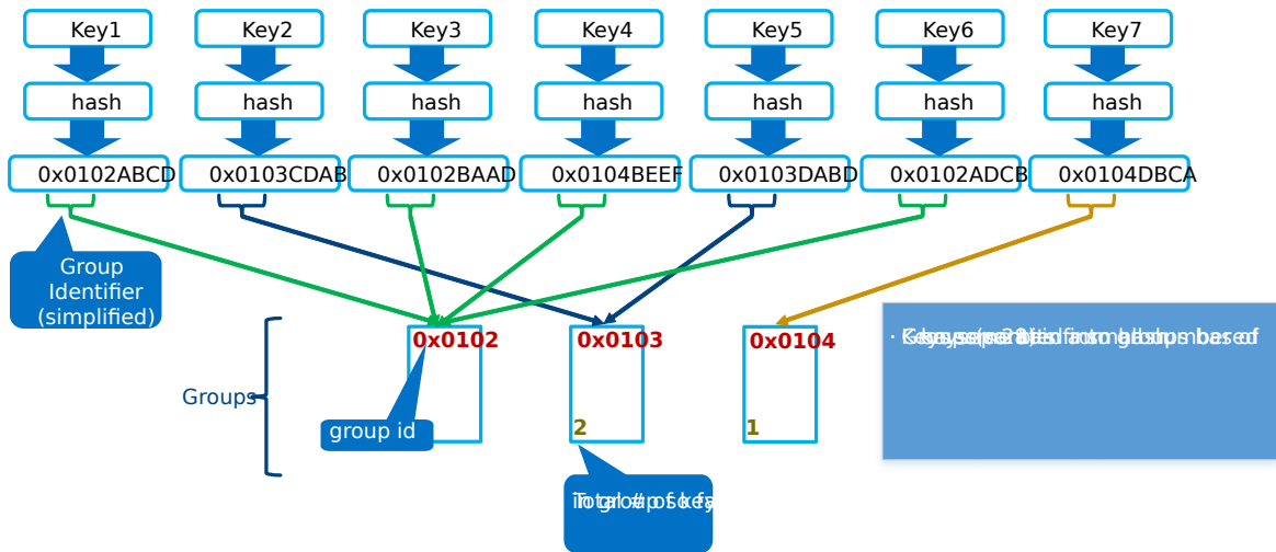
Fig. 21.7: Group Assignment
