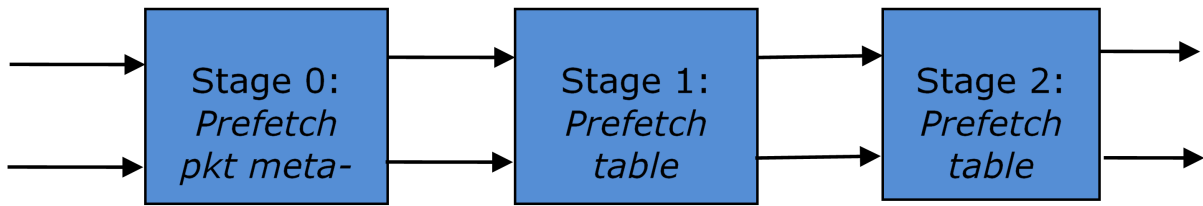
Fig. 43.7: Bucket Search Pipeline for Key Lookup Operation (Single Key Size Hash Tables)
