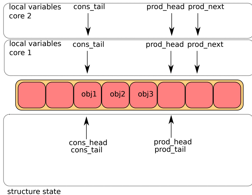
Fig. 6.8: Multiple producer enqueue first step
