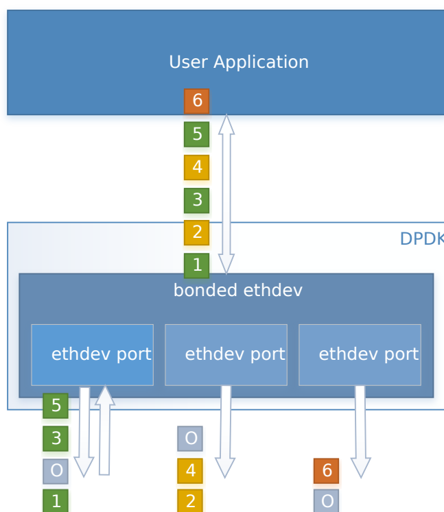
Fig. 20.6: Link Aggregation 802.3AD (Mode 4)
