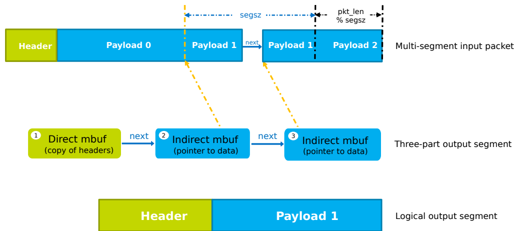
Fig. 32.2: Three-part GSO output segment
