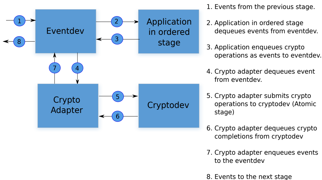
Fig. 41.2: Working model of RTE_EVENT_CRYPTOP_ADAPTER_OP_FORWARD mode
