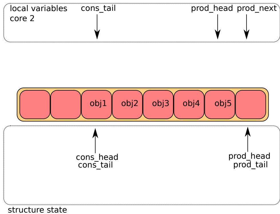
Fig. 6.12: Multiple producer enqueue last step
