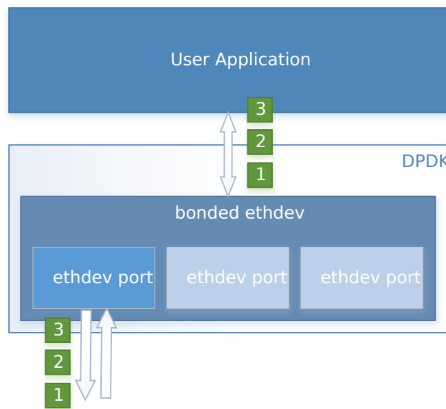
Fig. 20.3: Active Backup (Mode 1)
