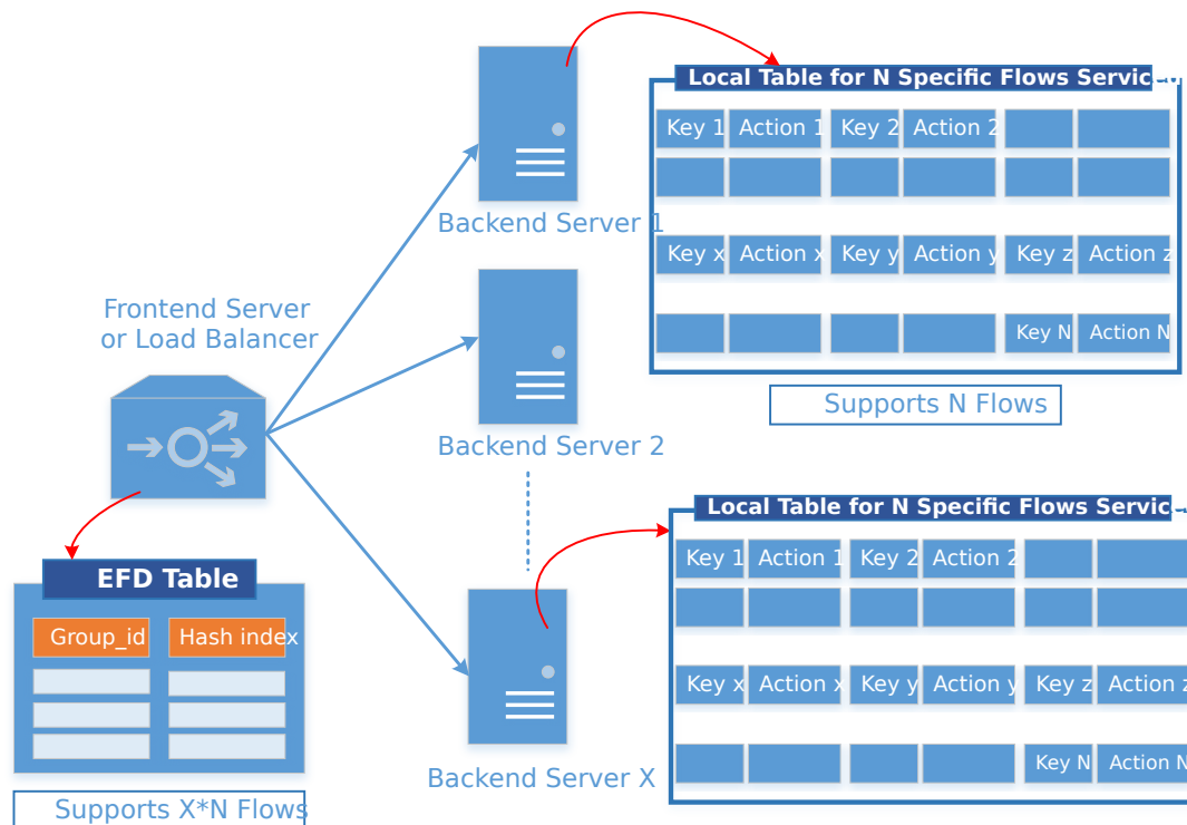
Fig. 23.6: EFD as a Flow-Level Load Balancer
