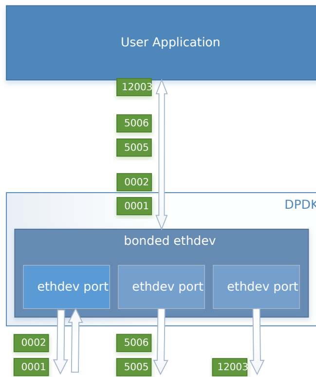
Fig. 20.7: Transmit Load Balancing (Mode 5)
