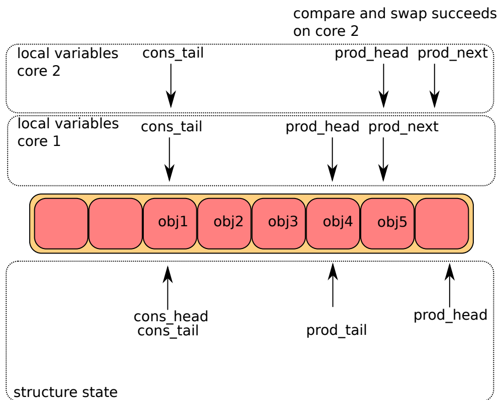
Fig. 6.10: Multiple producer enqueue third step
