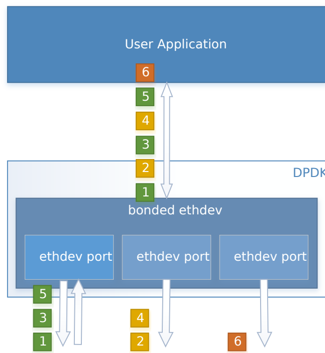
Fig. 20.4: Balance XOR (Mode 2)
