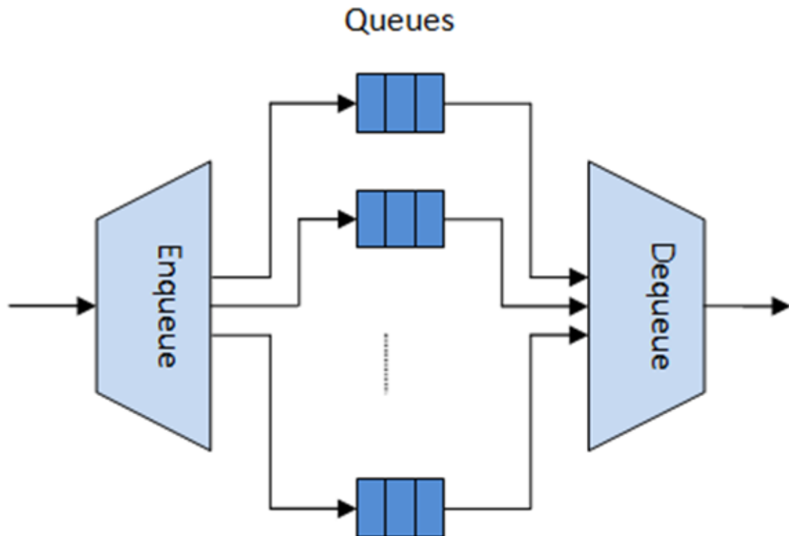
Fig. 42.2: Hierarchical Scheduler Block Internal Diagram
