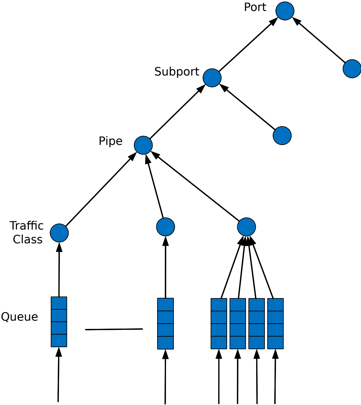
Fig. 42.3: Scheduling Hierarchy per Port
