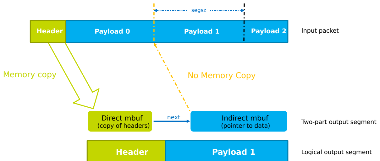
Fig. 32.1: Two-part GSO output segment
