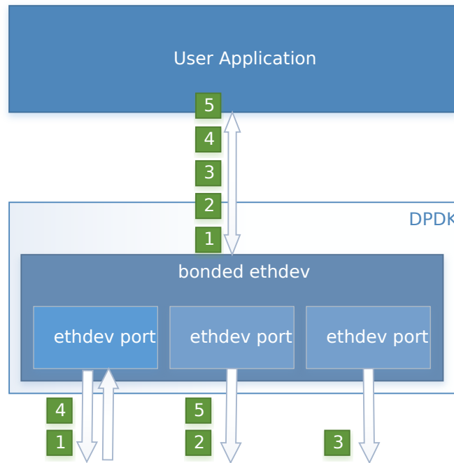
Fig. 20.2: Round-Robin (Mode 0)
