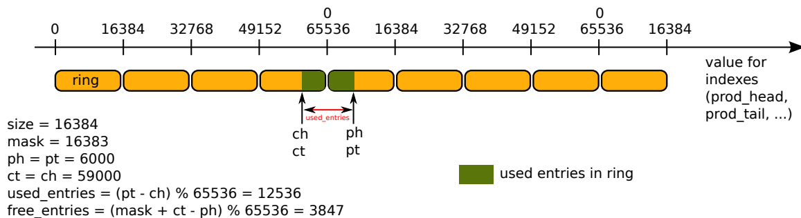
Fig. 6.14: Modulo 32-bit indexes - Example 2
