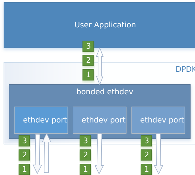
Fig. 20.5: Broadcast (Mode 3)
