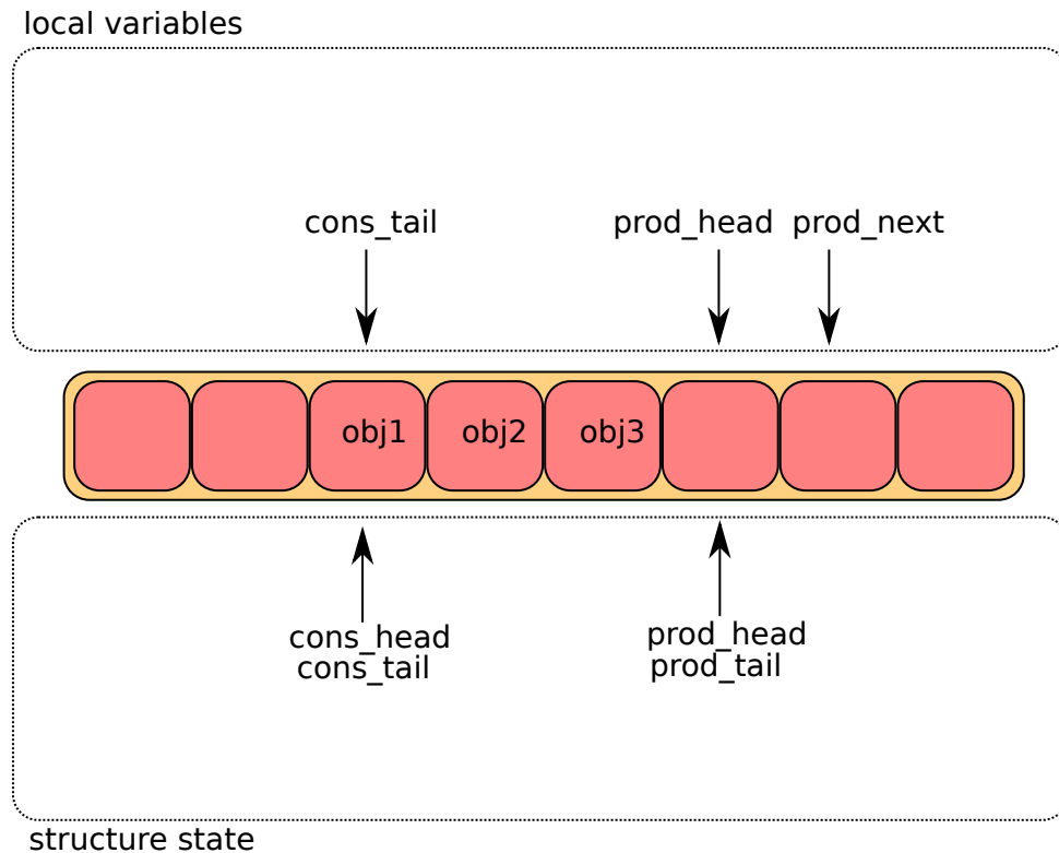
Fig. 6.2: Enqueue first step
