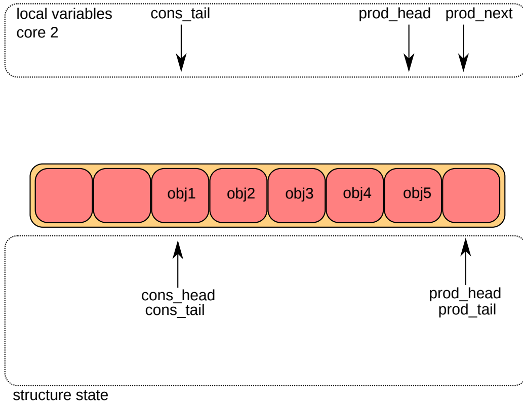
Fig. 6.12: Multiple producer enqueue last step
