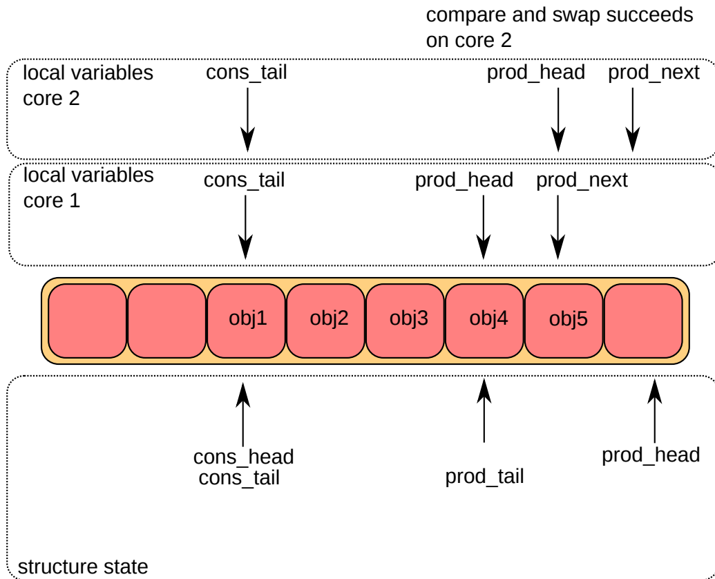
Fig. 6.10: Multiple producer enqueue third step
