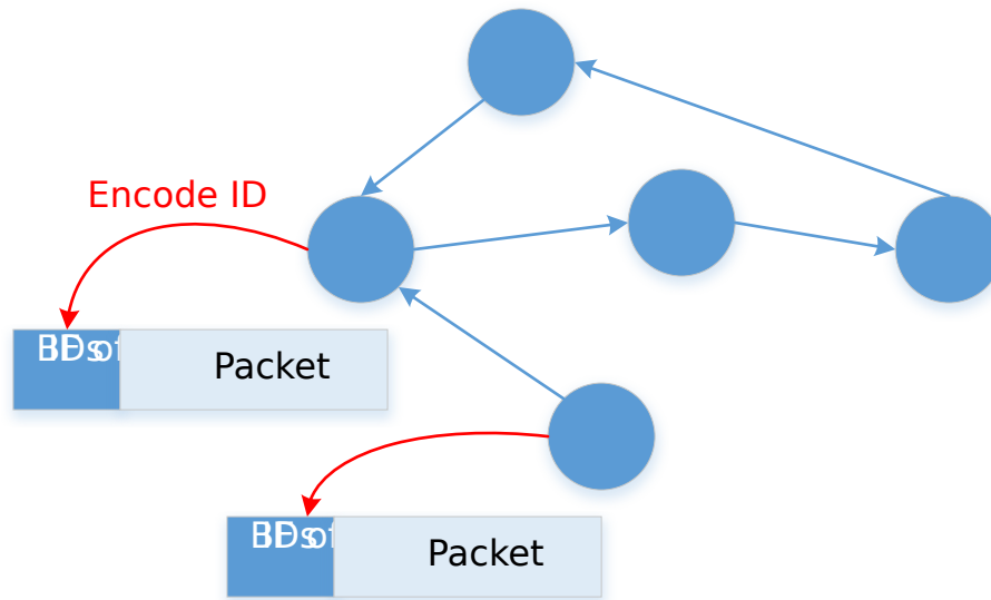
Fig. 24.3: Detecting Routing Loops Using BF
