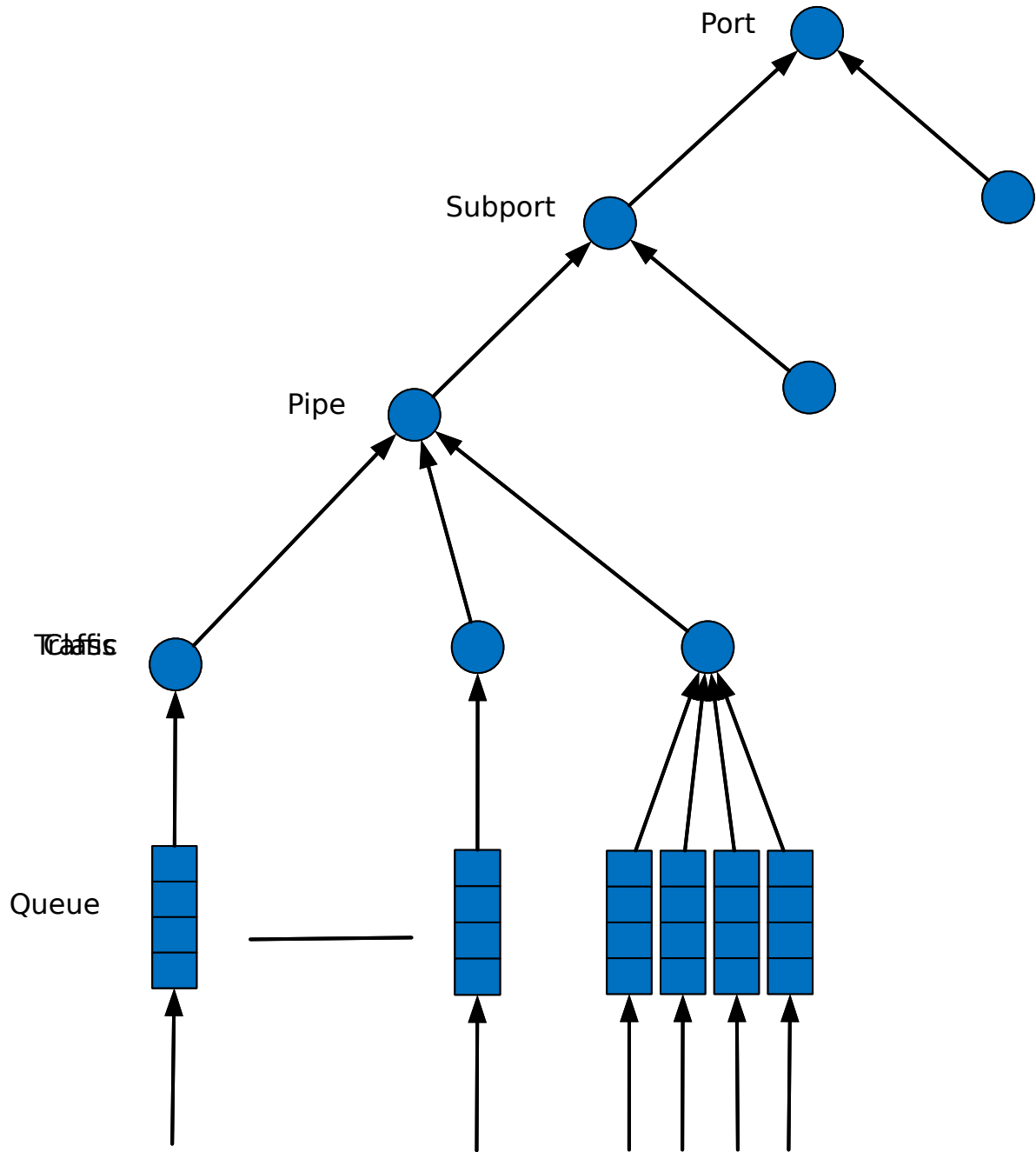
Fig. 42.3: Scheduling Hierarchy per Port
