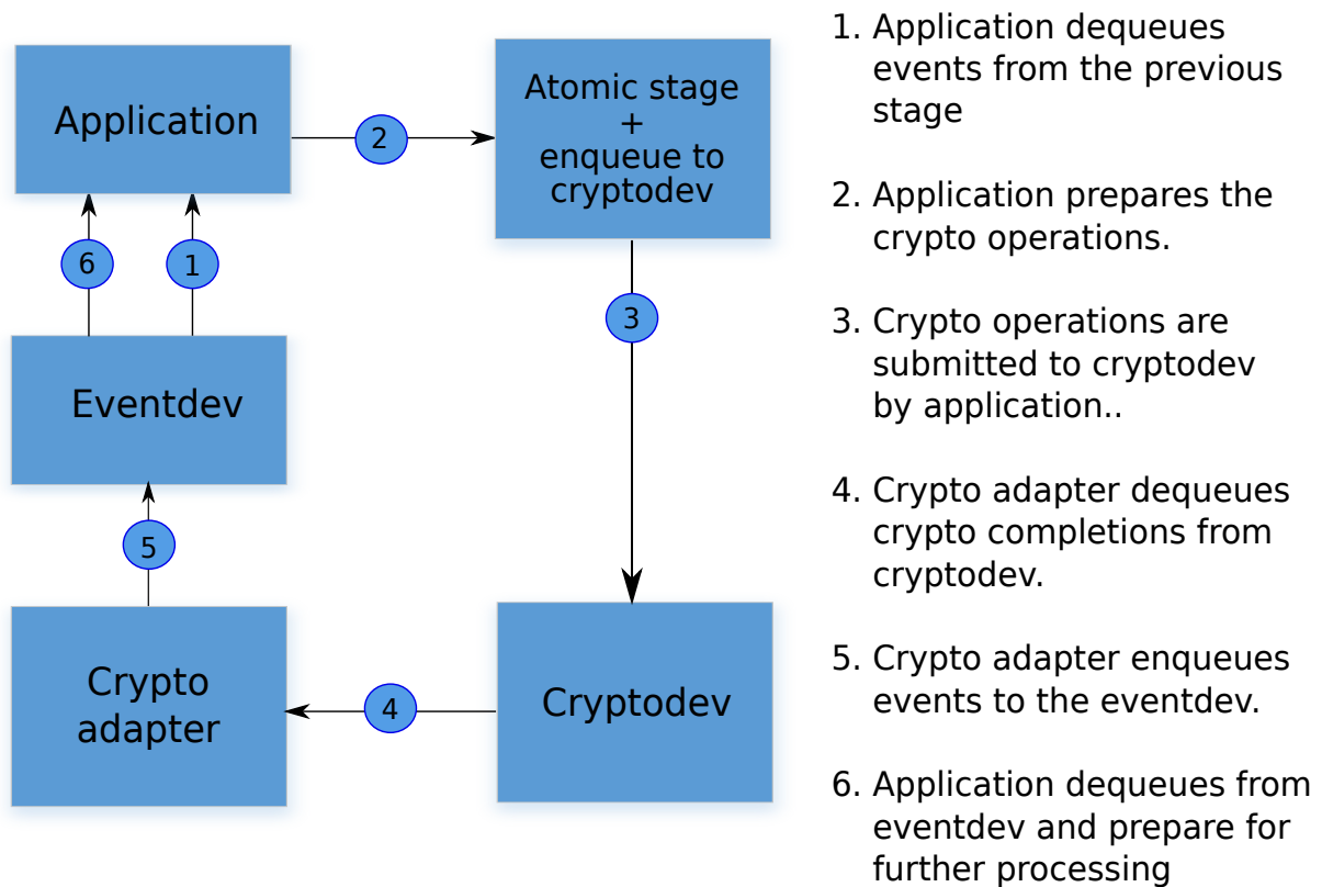
Fig. 41.1: Working model of RTE_EVENT_CRYPTODEV_ADAPTER_OP_NEW mode
