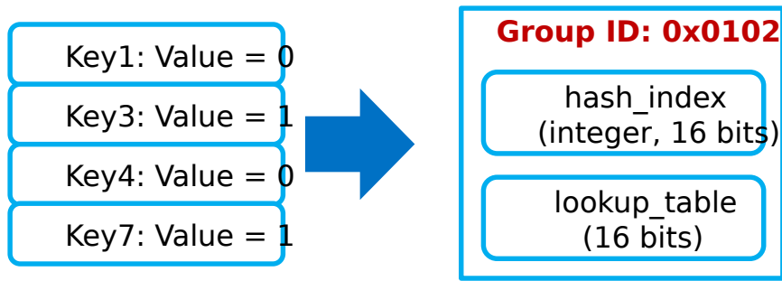
Fig. 23.8: Perfect Hash Search - Assigned Keys & Target Value
