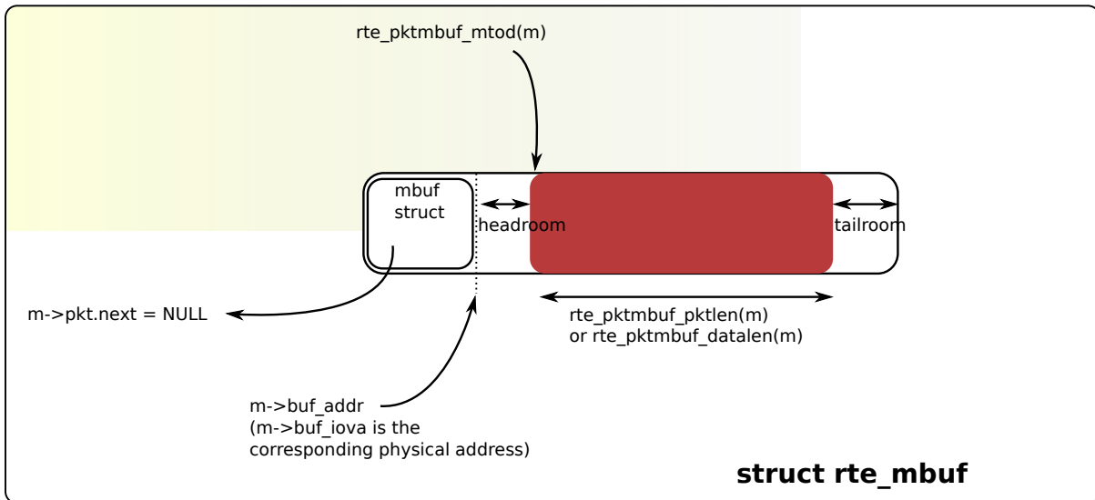
Fig. 9.1: An mbuf with One Segment
