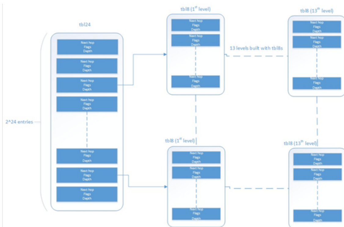
Fig. 26.1: Table split into different levels
