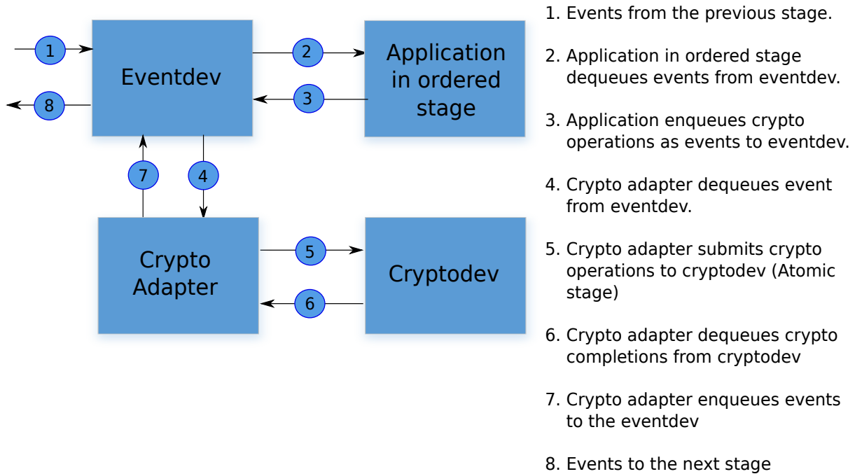
Fig. 41.2: Working model of RTE_EVENT_CRYPTODEV_ADAPTER_OP_FORWARD mode
