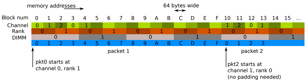
Fig. 8.2: Three Channels and Two Dual-ranked DIMM Example
