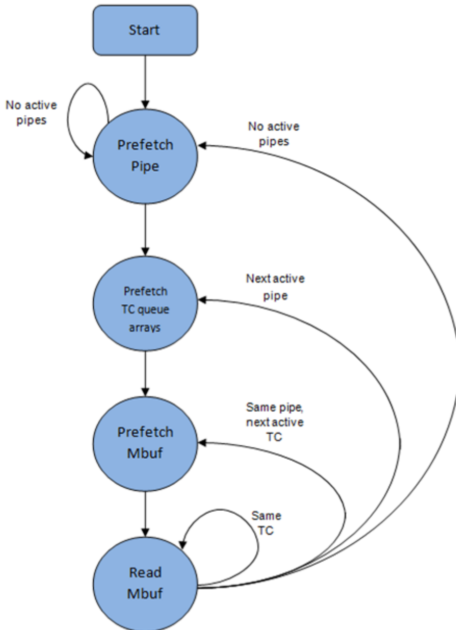
Fig. 42.6: Pipe Prefetch State Machine for the Hierarchical Scheduler Dequeue Operation
