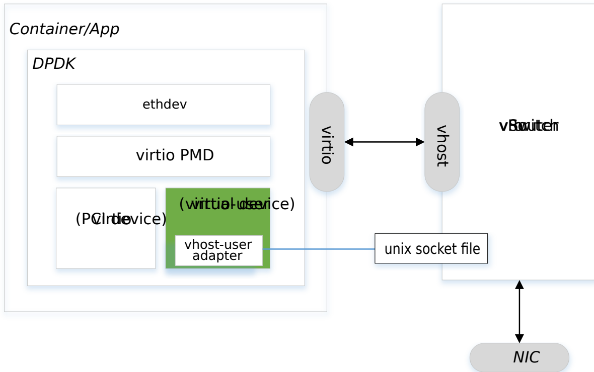
Fig. 6.2: Overview of accelerating container networking by virtio-user
