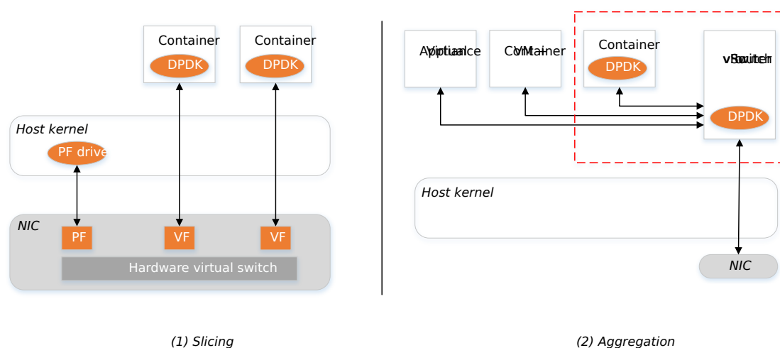
Fig. 6.1: Use models of running DPDK inside container
