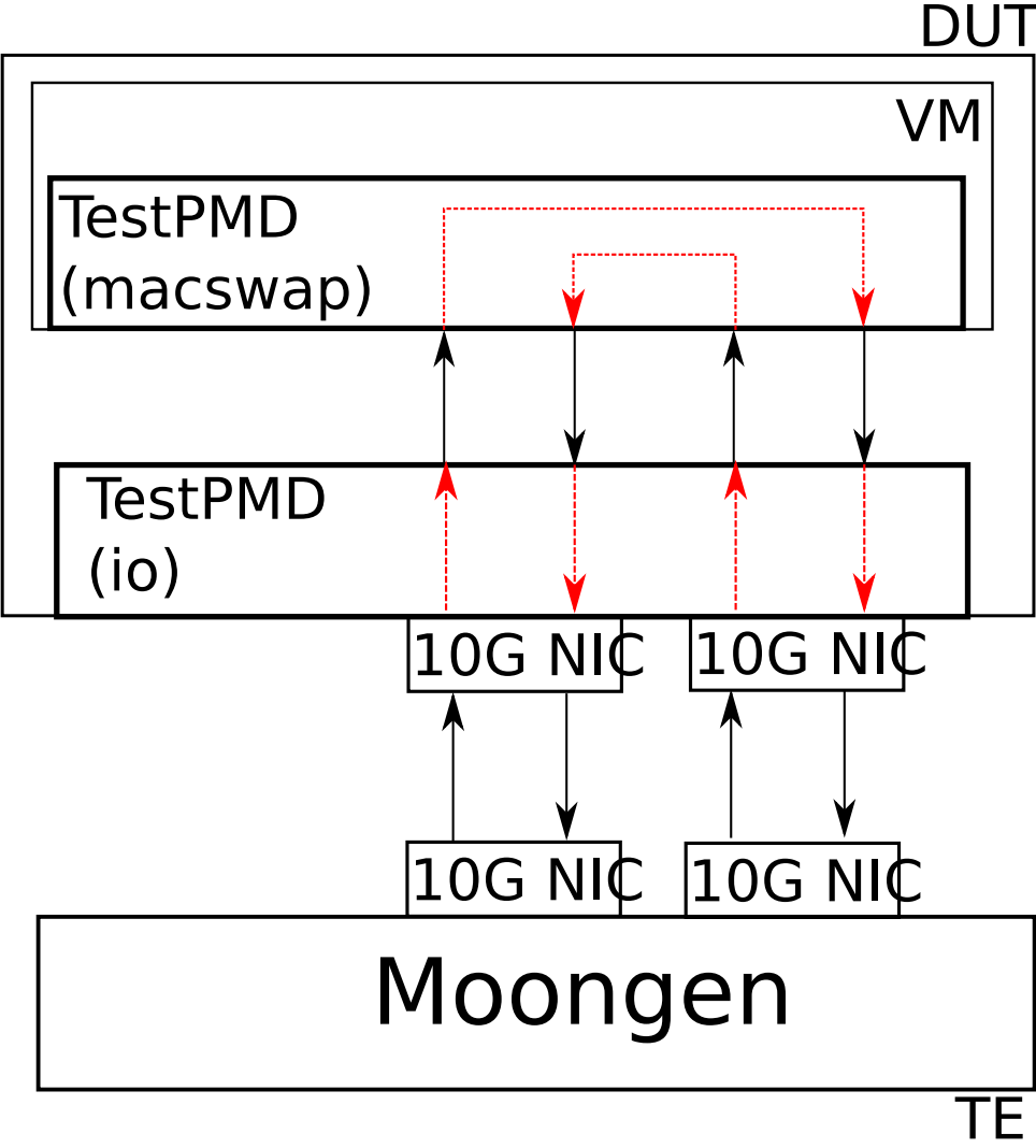
Fig. 4.1: PVP setup using 2 NICs
