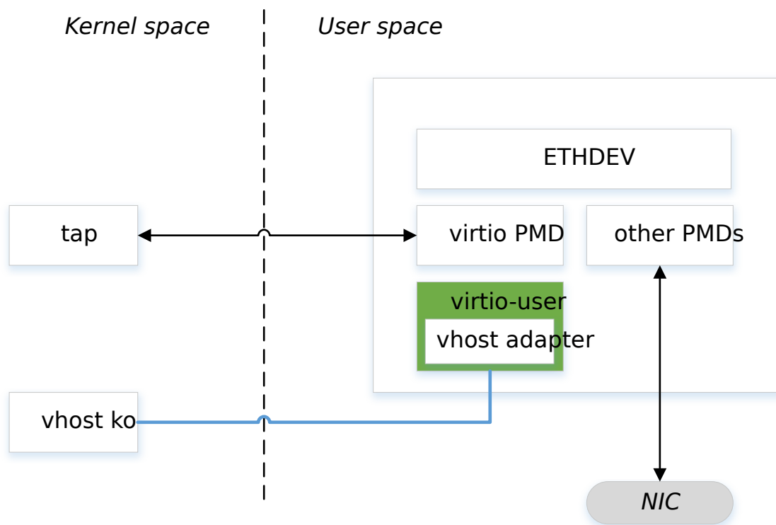
Fig. 7.1: Overview of a DPDK app using virtio-user as exceptional path
