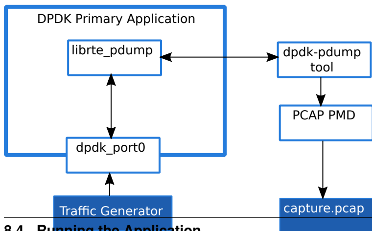
Fig. 8.1: Packet capturing on a DPDK port using the dpdk-pdump tool.
