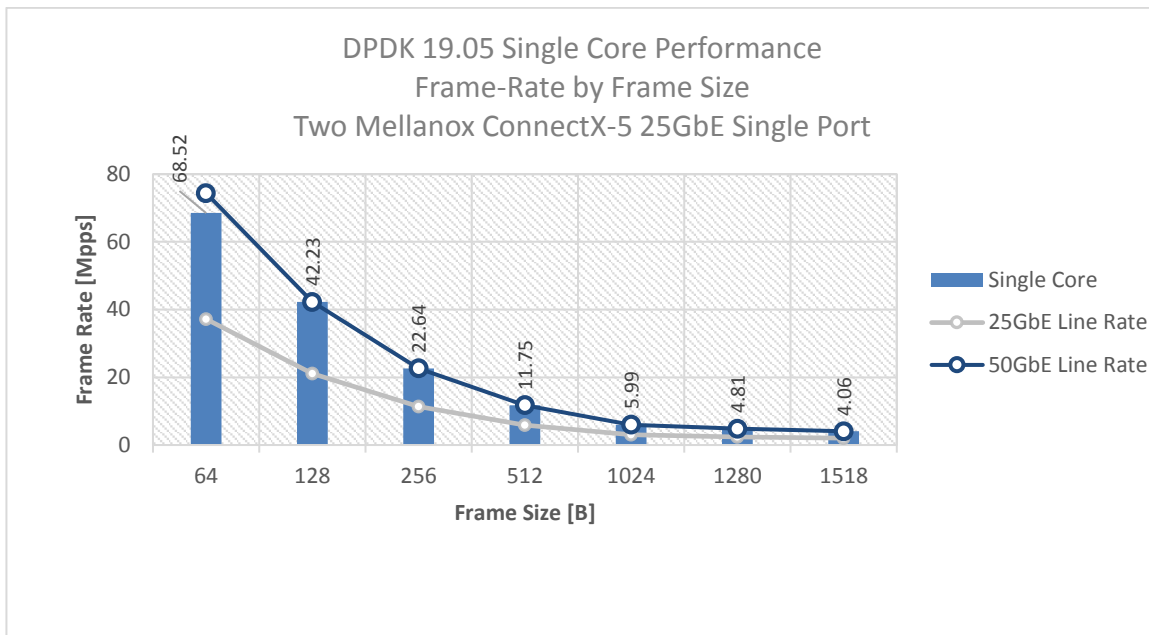
Figure 12: Test #6 Results – Mellanox ConnectX-5 25GbE Single Core Performance
