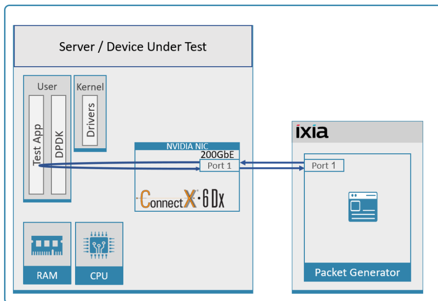
Figure 9 - Test #5 Setup – NVIDIA ConnectX-6 Dx 200GbE connected to IXIA
