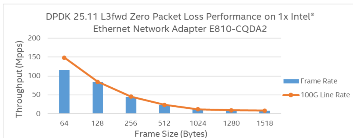
Figure 8: RFC2544 zero packet loss test on 1x Intel® Ethernet Network Adapter E810-CQDA2
