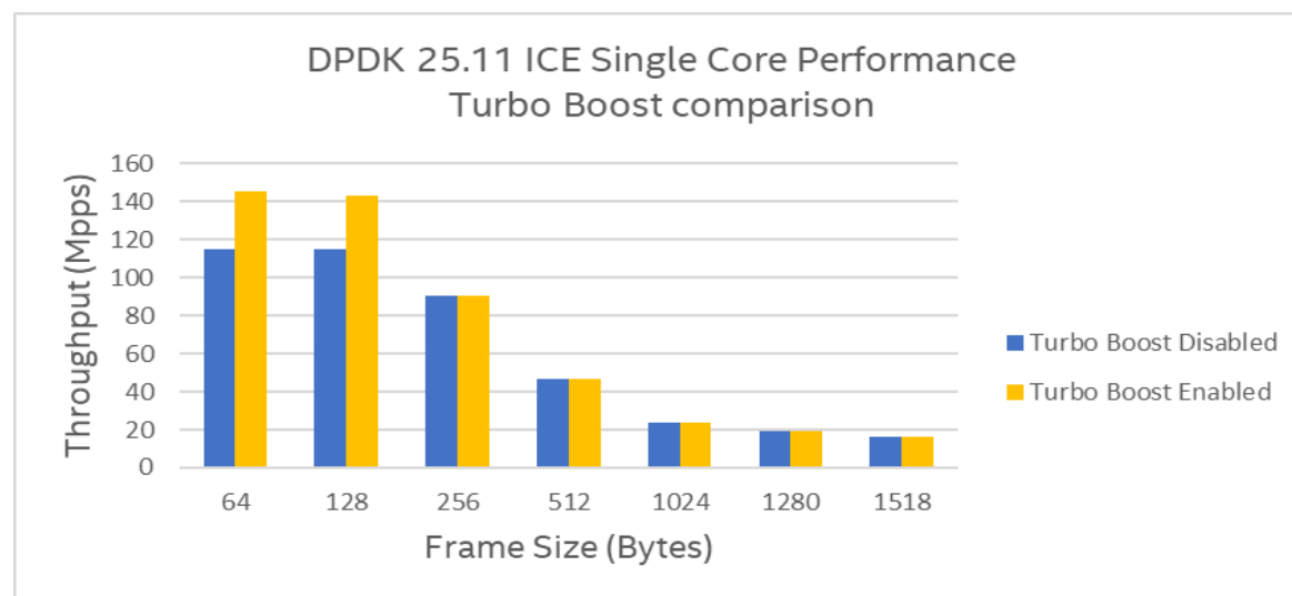
Figure 10: ice PMD Single core performance on 2x Intel® Ethernet Network Adapter E810-QCDA2 with turbo boost comparison
