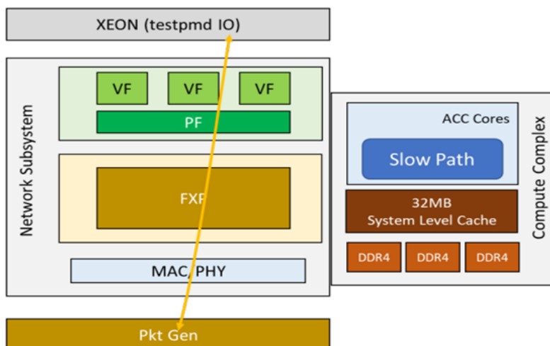
Figure 22: Test #10 Setup – 1x Intel® IPU Adapter E2100-CCQDA2 connected to IXIA
