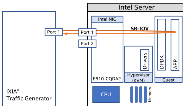
Figure 12: Test #5 Setup – 1x Intel® Ethernet Network Adapter E810-CQDA2 connected to IXIA (Single port)
