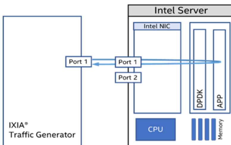
Figure 16: Test #7 Setup – 1x Intel® Ethernet Network Adapter E830-CQDA2 connected to IXIA ( 2 ports used on 1 NIC)
