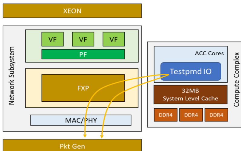
Figure 25: Test #11 Setup – 1x Intel® IPU Adapter E2100-CCQDA2 connected to IXIA
