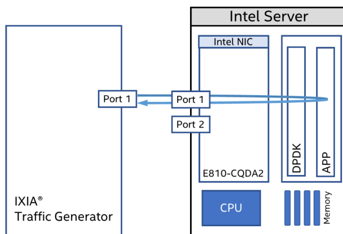
Figure 7: Test #3 Setup – 1x Intel® Ethernet Network Adapter E810-CQDA2 connected to IXIA (Single port)
