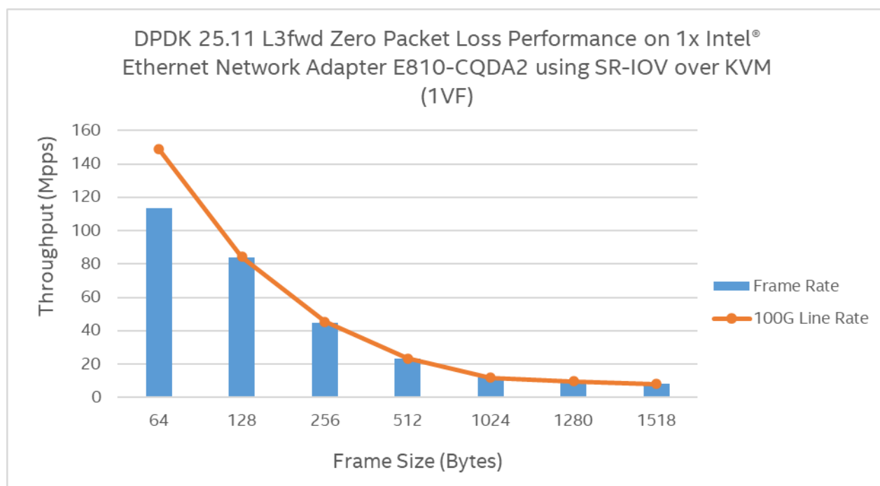
Figure 13: RFC2544 zero packet loss test on 1x Intel® Ethernet Network Adapter E810-CQDA2 using SRIOV over KVM
