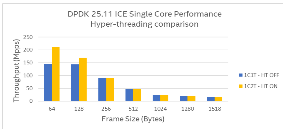
Figure 11: ice PMD Single core performance on 2x Intel® Ethernet Network Adapter E810-QCDA2 with hyper-threading comparison
