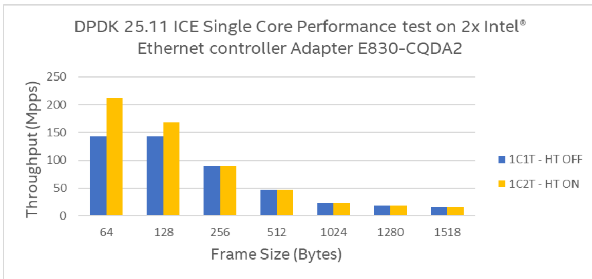
Figure 19: ice PMD Single core performance on 2x Intel® Ethernet Network Adapter E830-CQDA2
