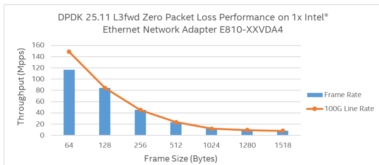
Figure 15: RFC2544 zero packet loss test on 1x Intel® Ethernet Network Adapter E810-XXVDA4
