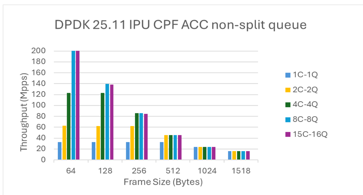
Figure 27: ACC non-split queue on 1x Intel® IPU Adapter E2100-CCQDA2
