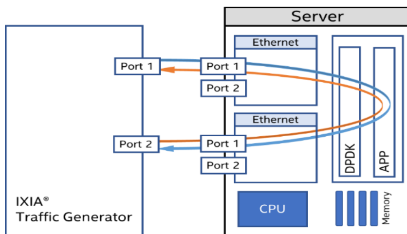
Figure 18: Test #8 Setup – 2x Intel® Ethernet Network Adapter E830-CQDA2 connected to IXIA
