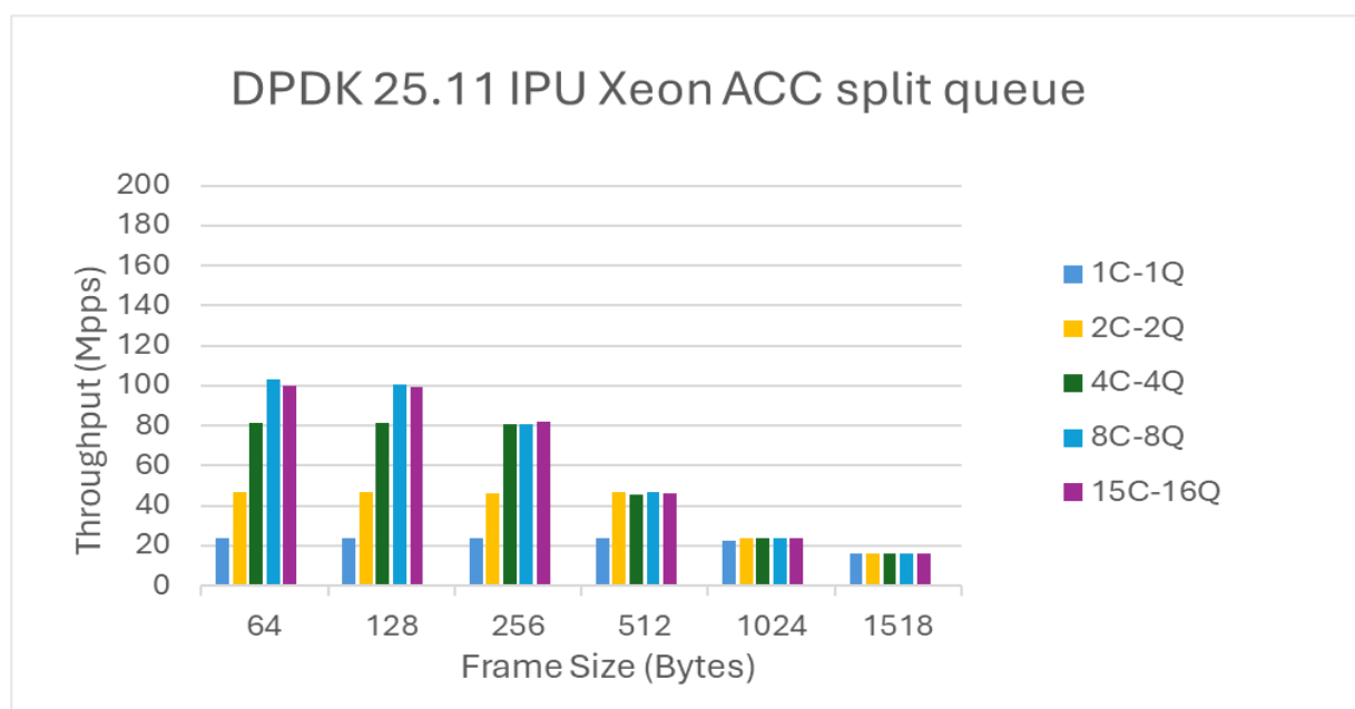
Figure 29: split queue on 1x Intel® IPU Adapter E2100-CCQDA2
