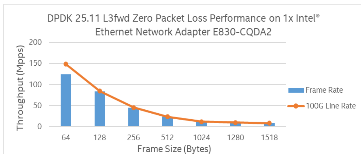
Figure 17: RFC2544 zero packet loss test on 1x Intel® Ethernet Network Adapter E830-CQDA2
