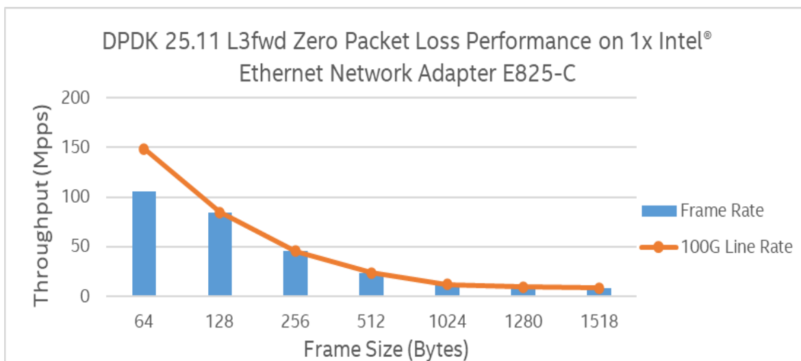
Figure 21: RFC2544 zero packet loss test on 1x Intel® Ethernet Network Adapter E825-C
