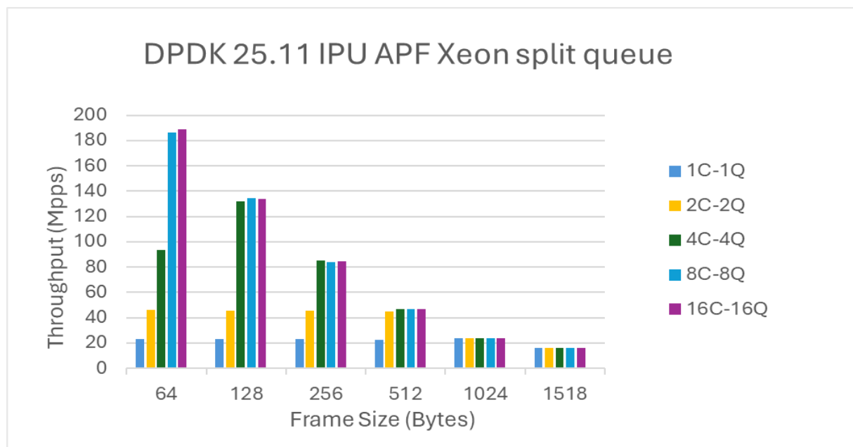
Figure 23: Xeon split queue on 1x Intel® IPU Adapter E2100-CCQDA2
