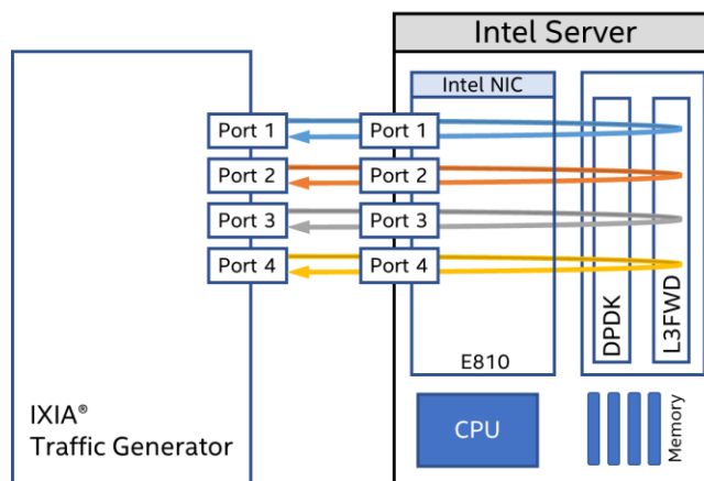
Figure 14: Test #6 Setup – 1x Intel® Ethernet Network Adapter E810-XXVDA4 connected to IXIA (4 ports of 1 NIC)
