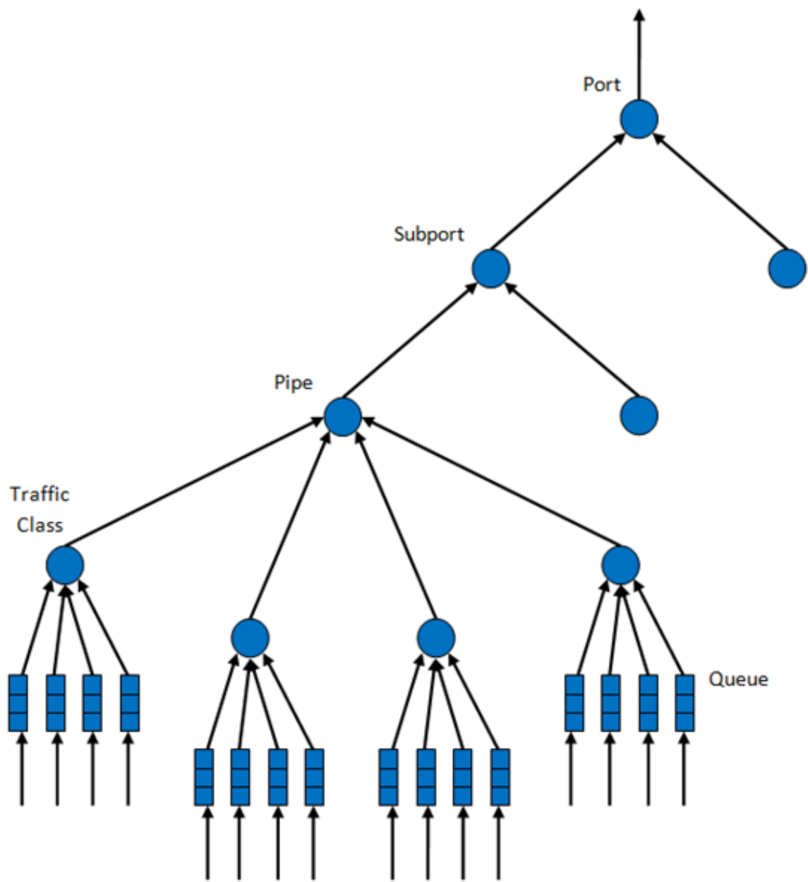
Fig. 22.3: Scheduling Hierarchy per Port
