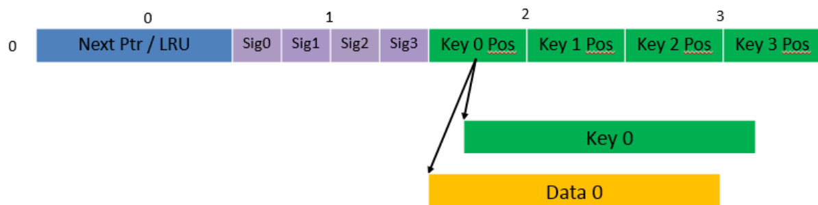
Fig. 25.3: Data Structures for Configurable Key Size Hash Tables
