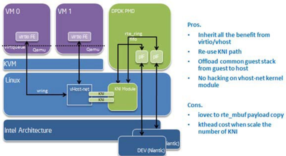
Fig. 20.3: vHost-net Architecture Overview
