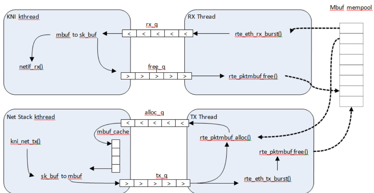
Fig. 20.2: Packet Flow via mbufs in the DPDK KNI
