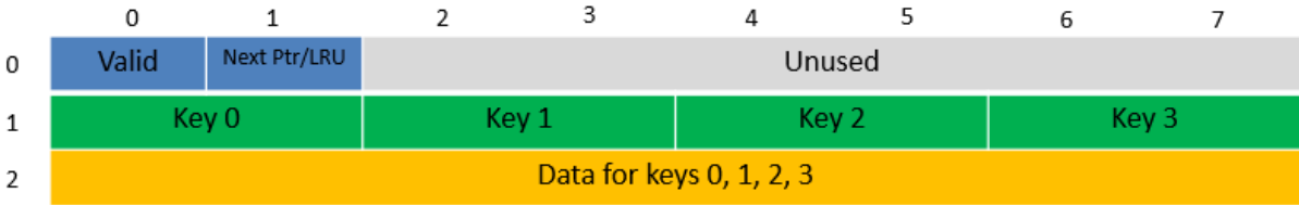
Fig. 25.6: Data Structures for 16-byte Key Hash Tables
