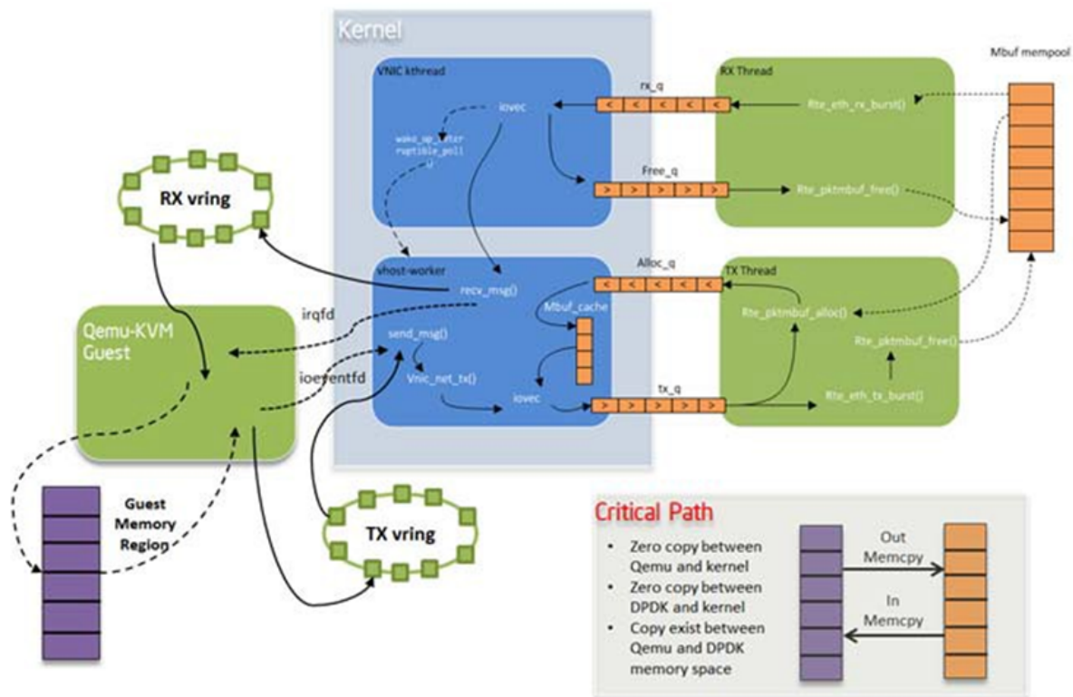
Fig. 20.4: KNI Traffic Flow
