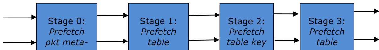
Fig. 25.4: Bucket Search Pipeline for Key Lookup Operation (Configurable Key Size Hash Tables)
