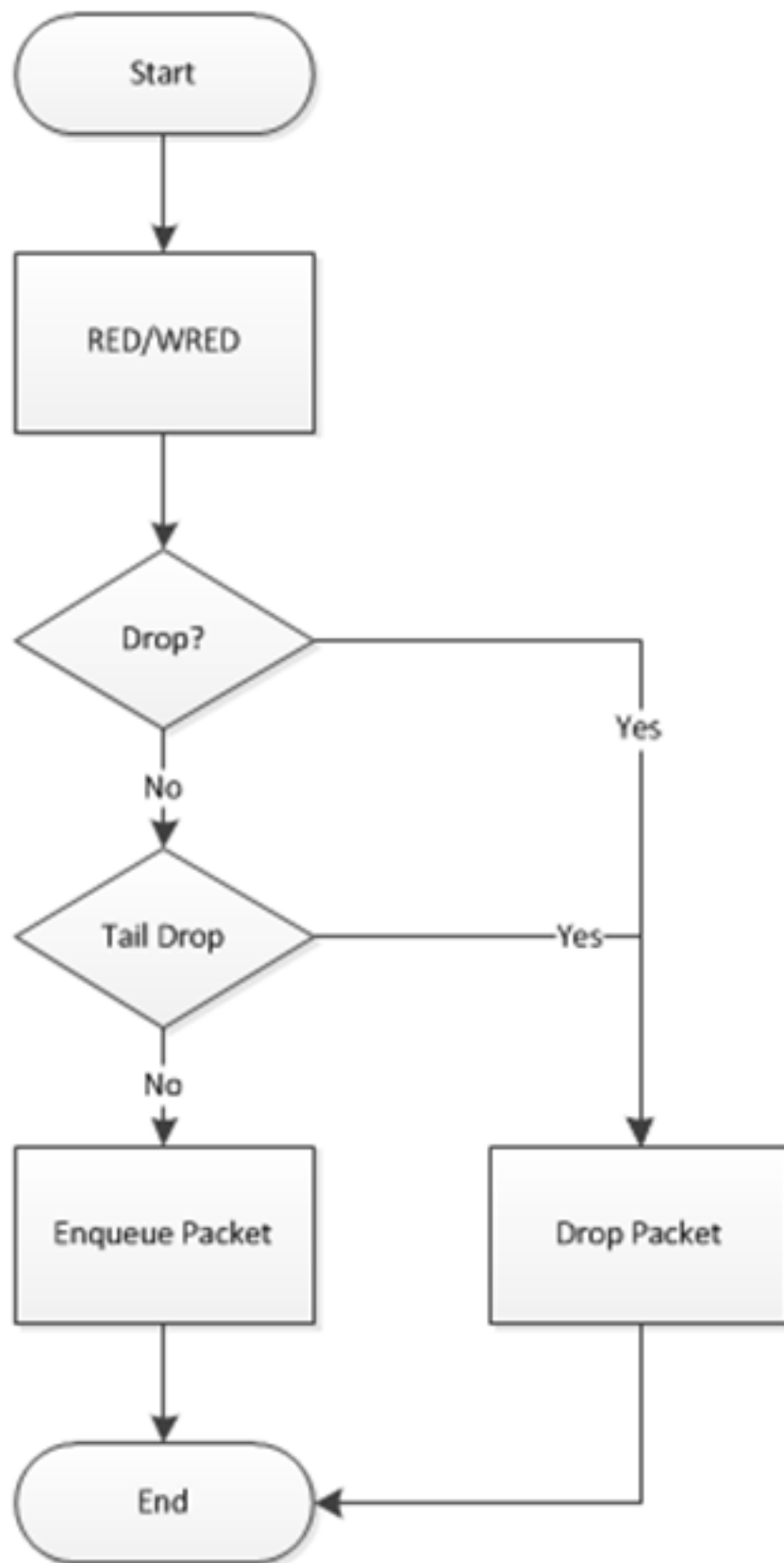
Fig. 22.8: Flow Through the Dropper
