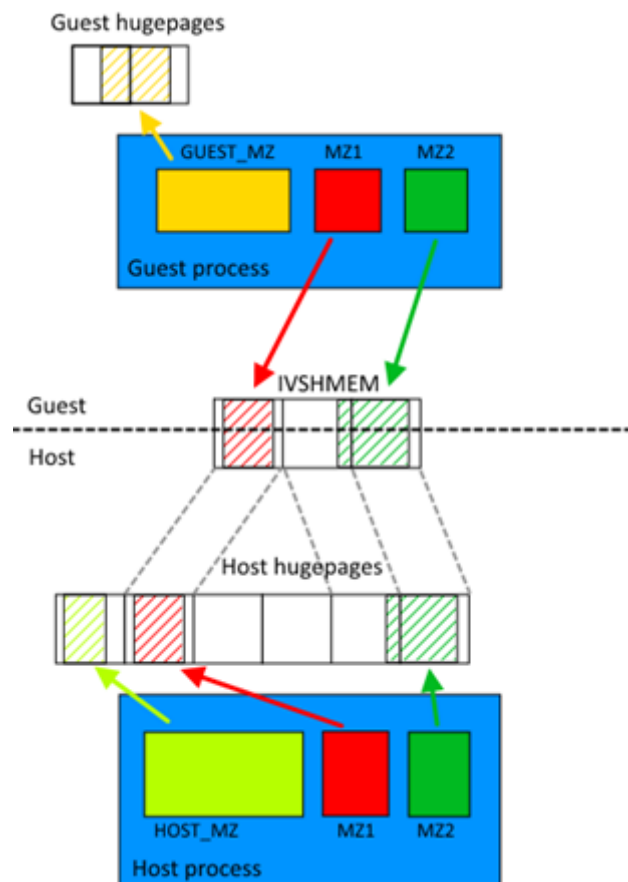
Fig. 9.1: Typical Ivshmem use case
