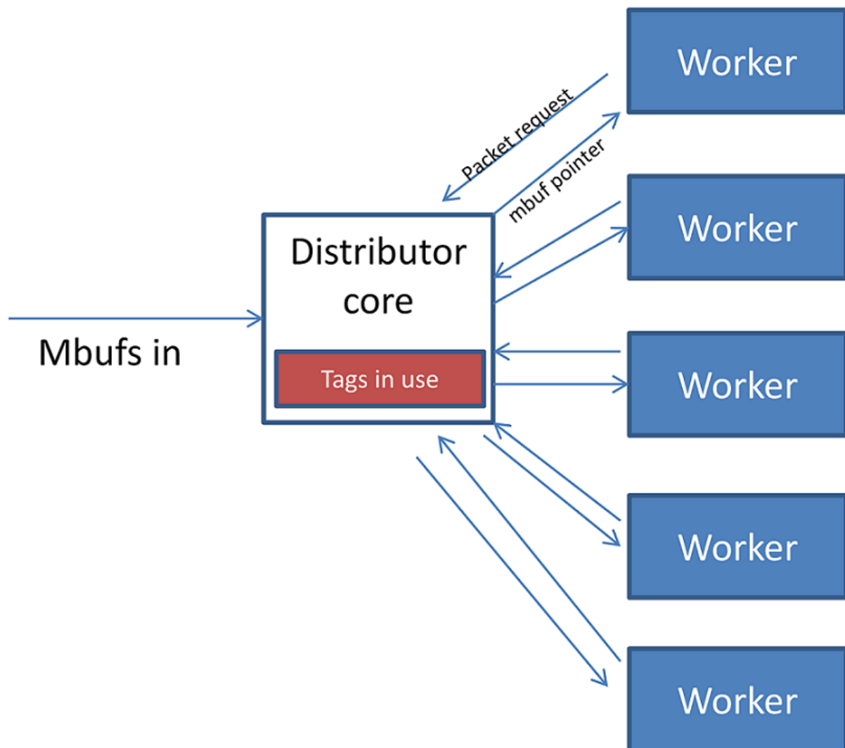
Fig. 16.1: Packet Distributor mode of operation
