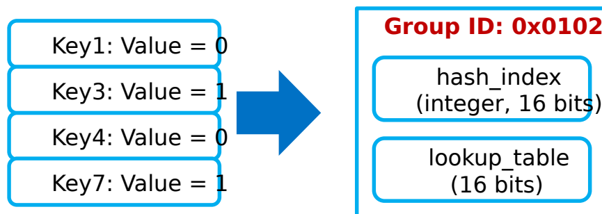
Fig. 13.8: Perfect Hash Search - Assigned Keys & Target Value
