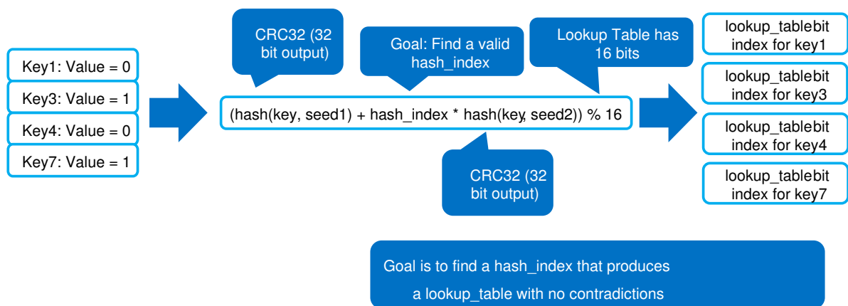
Fig. 13.9: Perfect Hash Search - Satisfy Target Values
