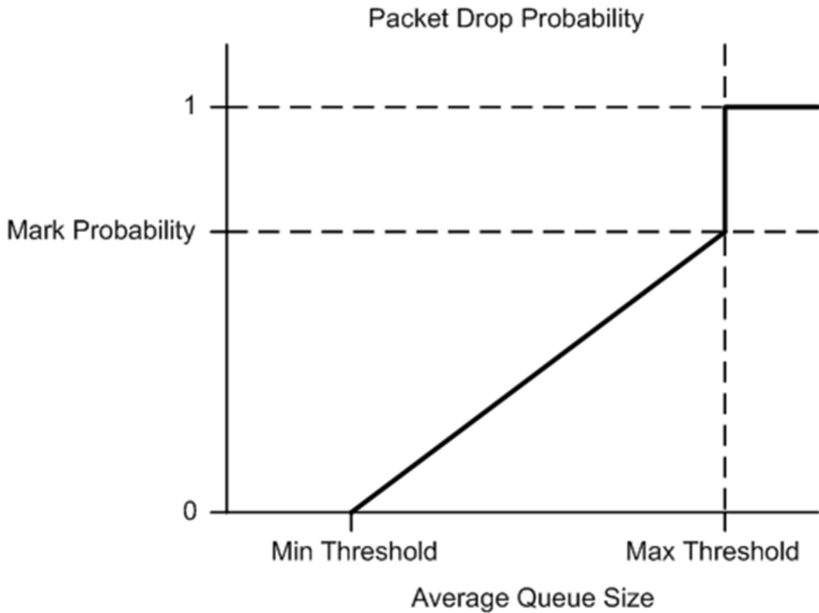
Fig. 23.10: Packet Drop Probability for a Given RED Configuration
