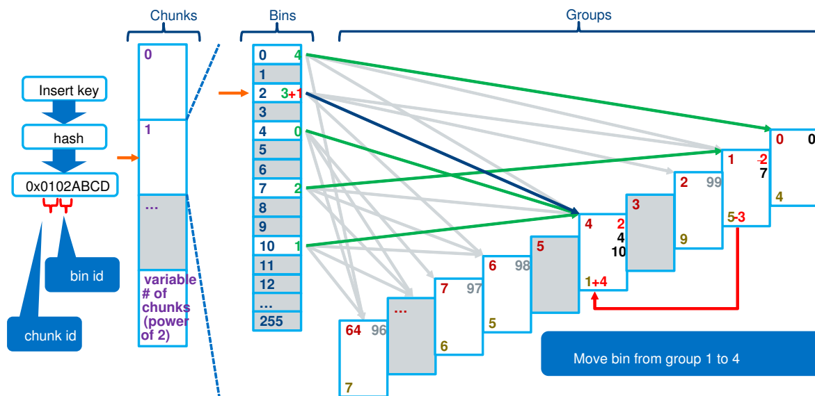
Fig. 13.12: Runtime Group Rebalancing
