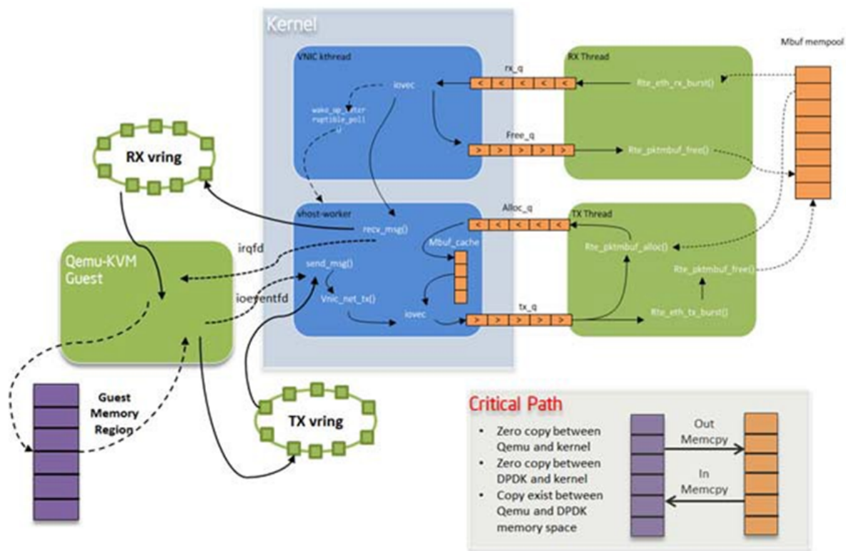
Fig. 21.4: KNI Traffic Flow
