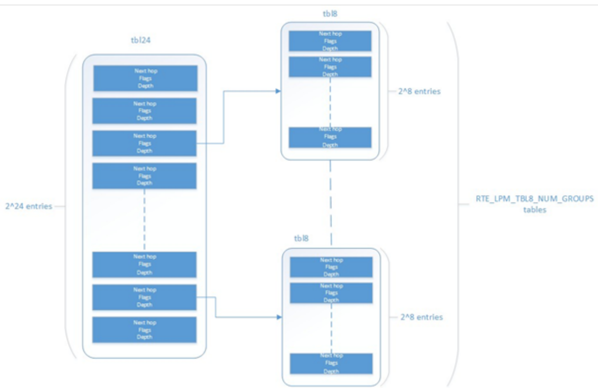
Fig. 14.1: Table split into different levels
