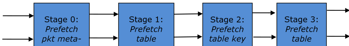
Fig. 26.4: Bucket Search Pipeline for Key Lookup Operation (Configurable Key Size Hash Tables)
