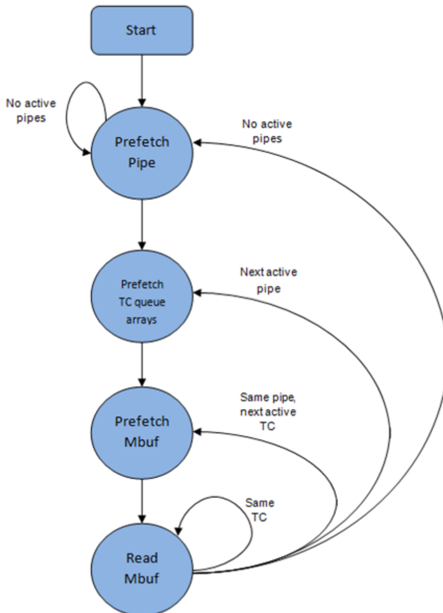
Fig. 23.6: Pipe Prefetch State Machine for the Hierarchical Scheduler Dequeue Operation
