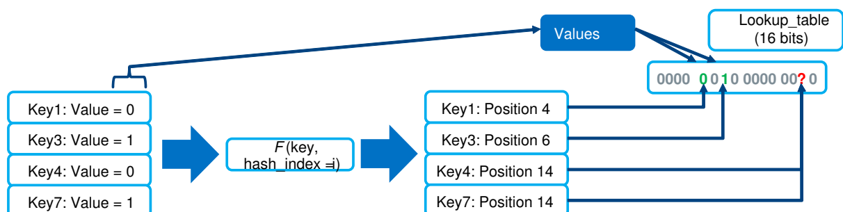
Fig. 13.10: Finding Hash Index for Conflict Free lookup_table
