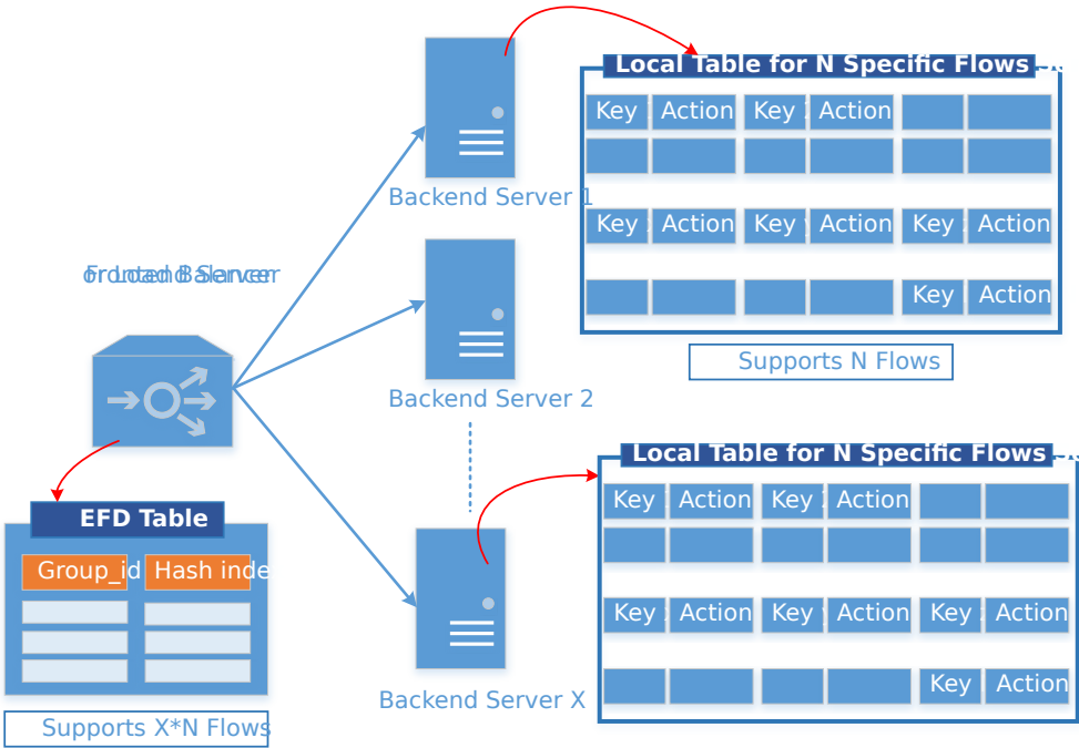
Fig. 13.6: EFD as a Flow-Level Load Balancer
