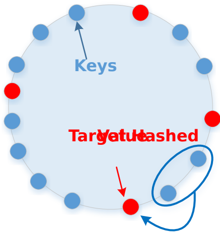
Fig. 13.2: Consistent Hashing
