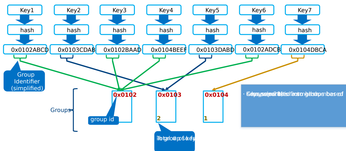
Fig. 13.7: Group Assignment
