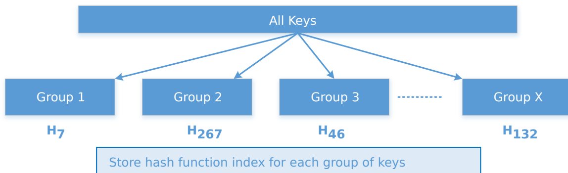
Fig. 13.5: Divide and Conquer for Millions of Keys
