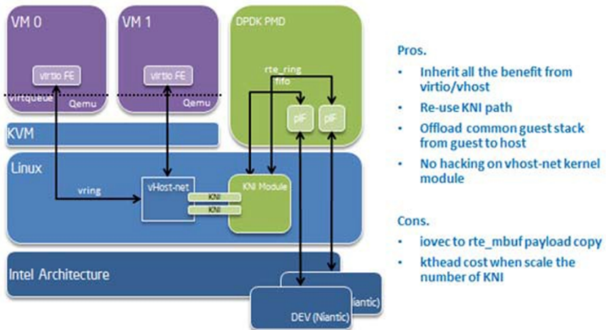
Fig. 21.3: vHost-net Architecture Overview
