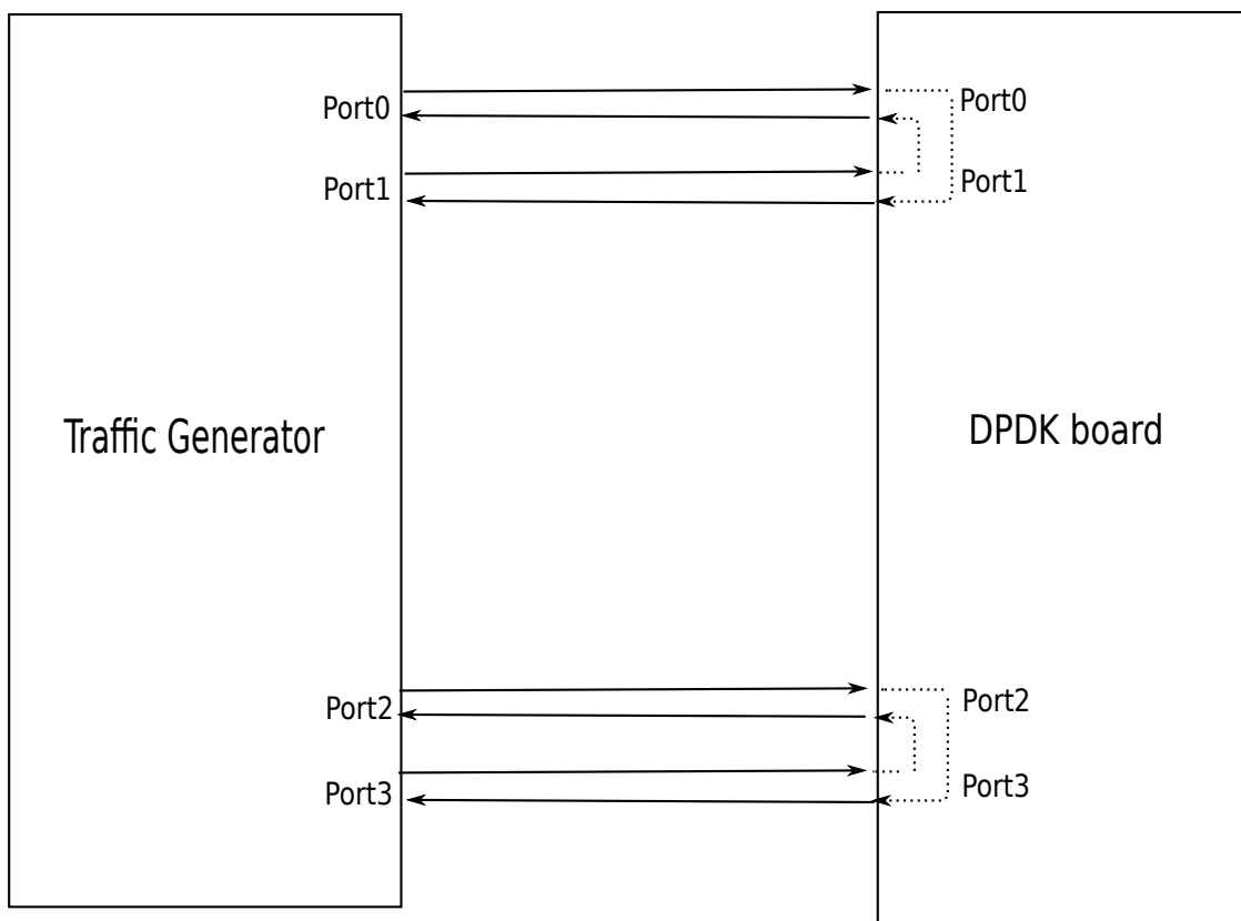
Fig. 41.1: Performance Benchmarking Setup (Basic Environment)
