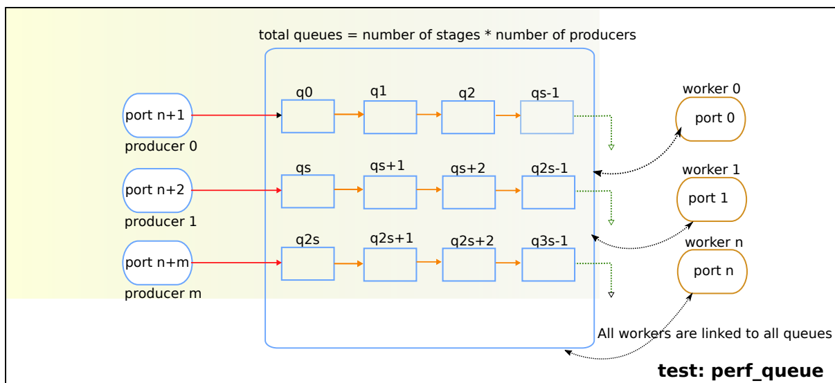
Fig. 7.3: perf queue test operation.
