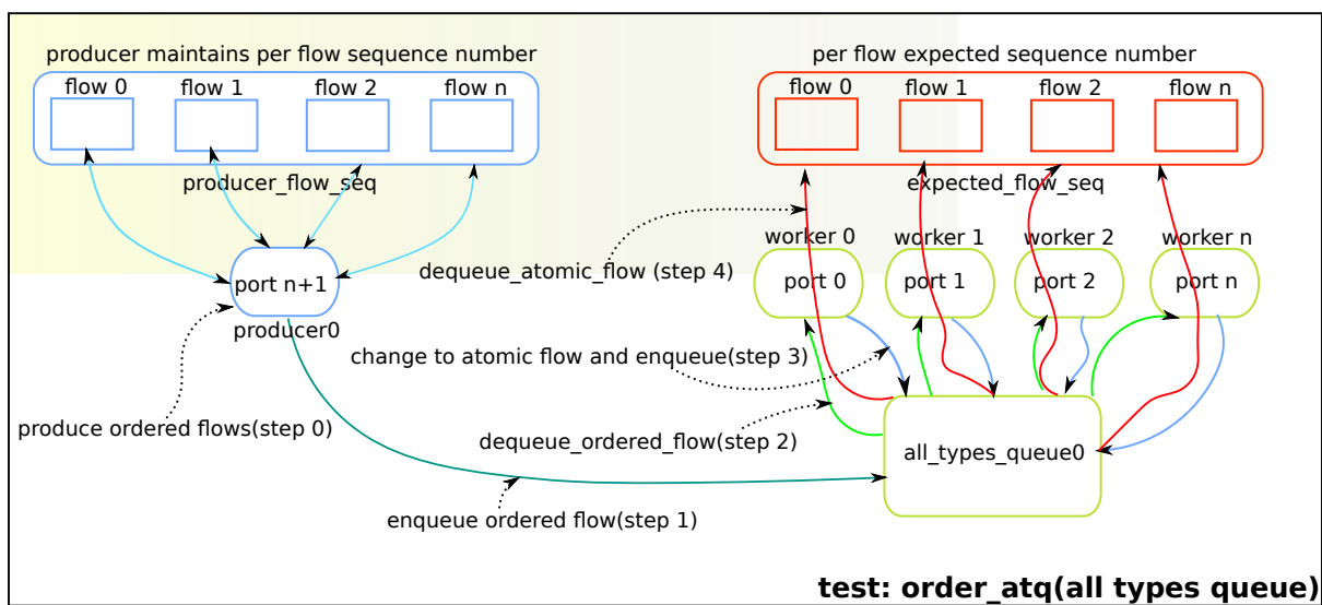
Fig. 7.2: order all types queue test operation.
