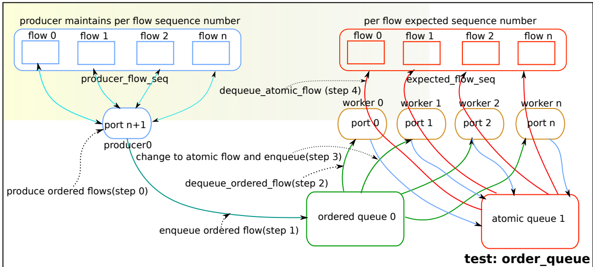
Fig. 7.1: order queue test operation.
