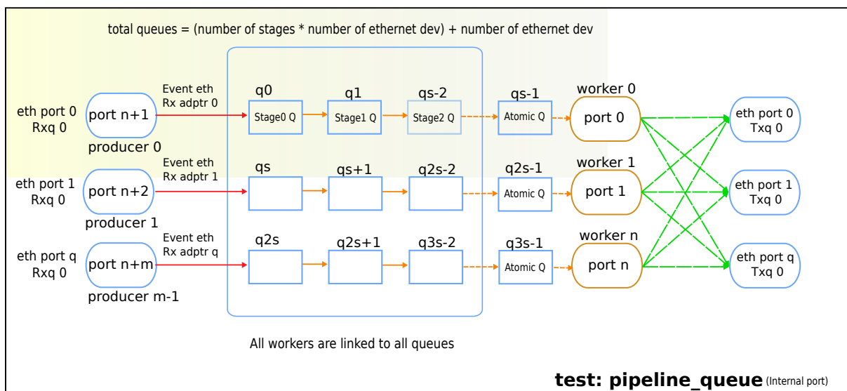
Fig. 7.5: pipeline queue test operation.
