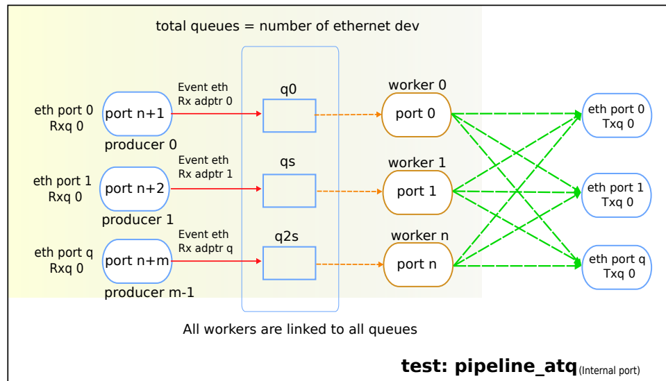
Fig. 7.6: pipeline atq test operation.
