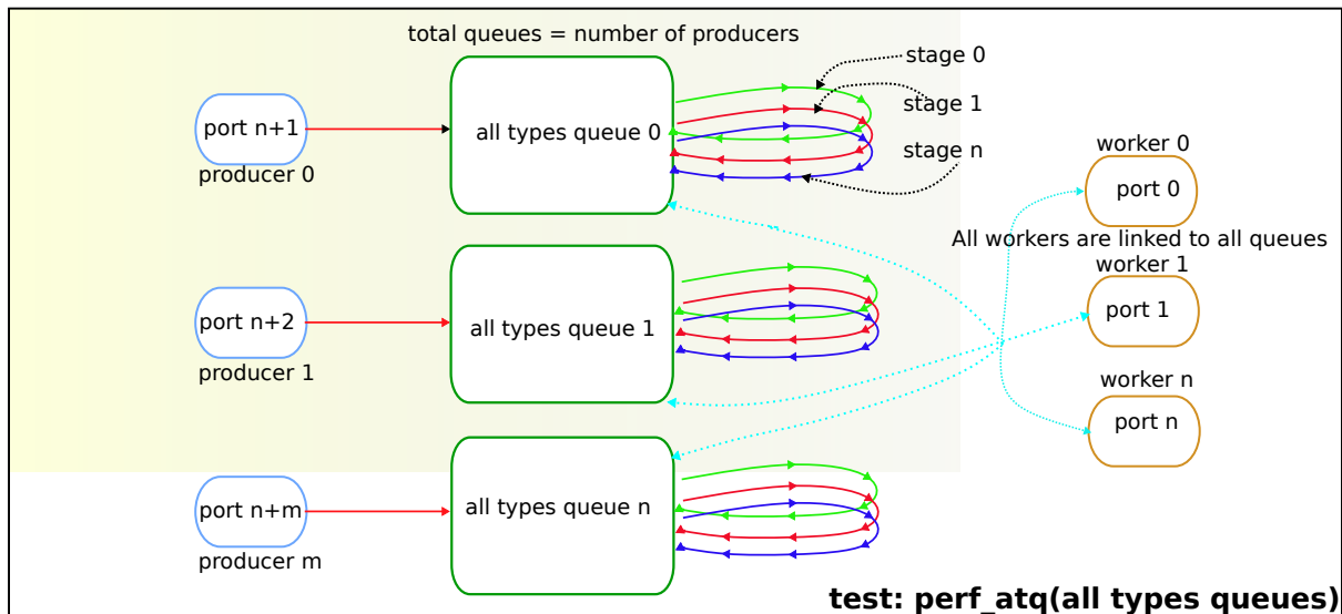
Fig. 7.4: perf all types queue test operation.
