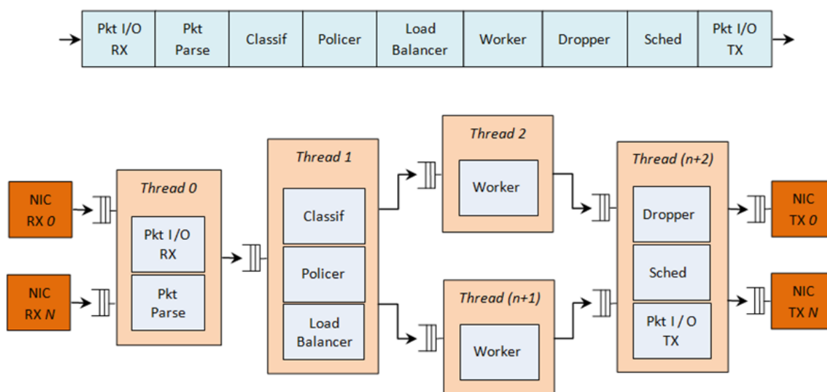
Fig. 40.1: Complex Packet Processing Pipeline with QoS Support
