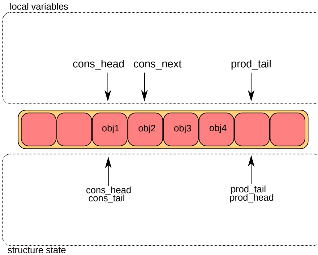
Fig. 5.5: Dequeue last step
