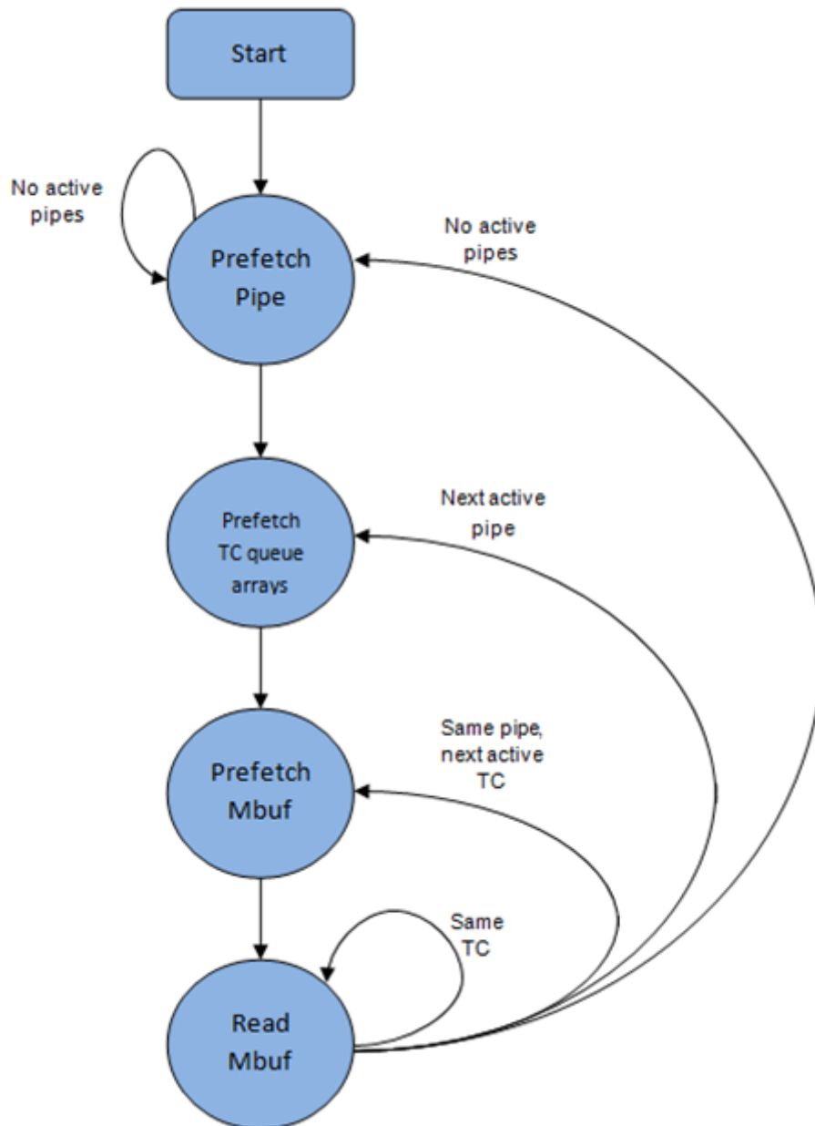
Fig. 40.6: Pipe Prefetch State Machine for the Hierarchical Scheduler Dequeue Operation
