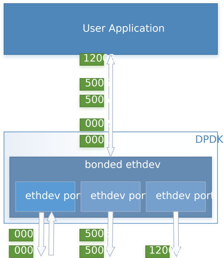
Fig. 18.7: Transmit Load Balancing (Mode 5)
