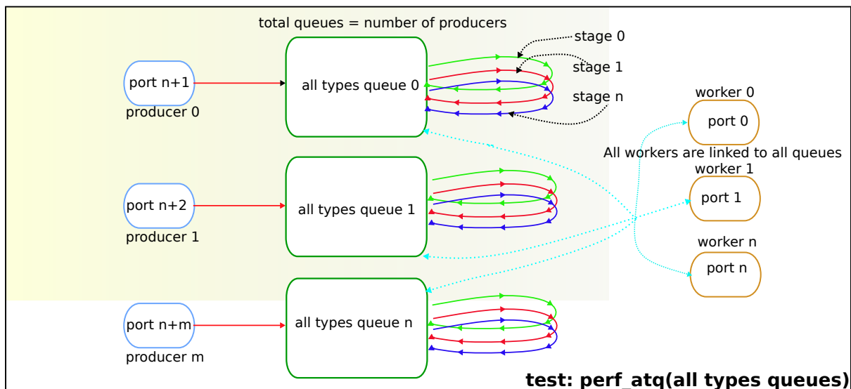
Fig. 9.4: perf all types queue test operation.
