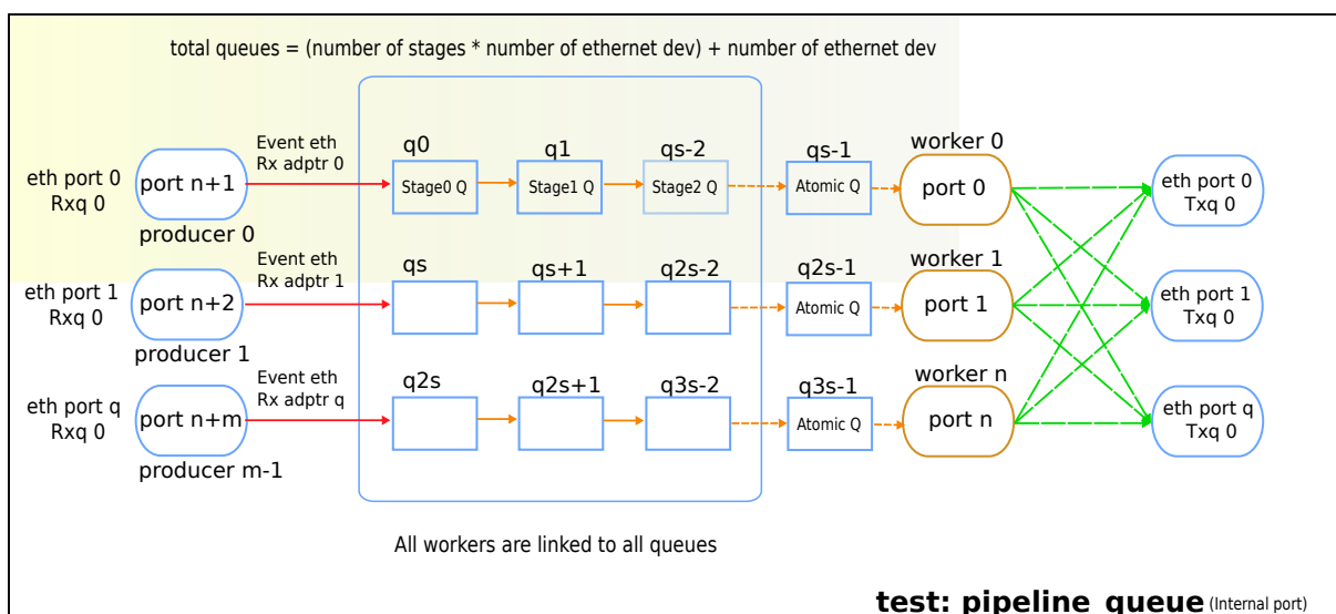
Fig. 9.5: pipeline queue test operation.
