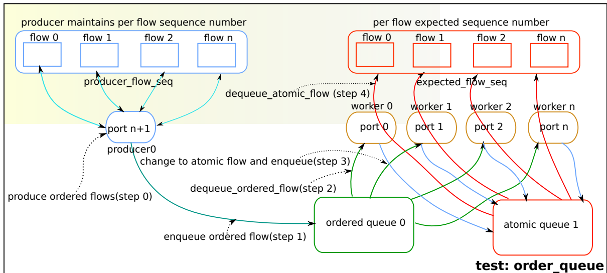
Fig. 9.1: order queue test operation.
