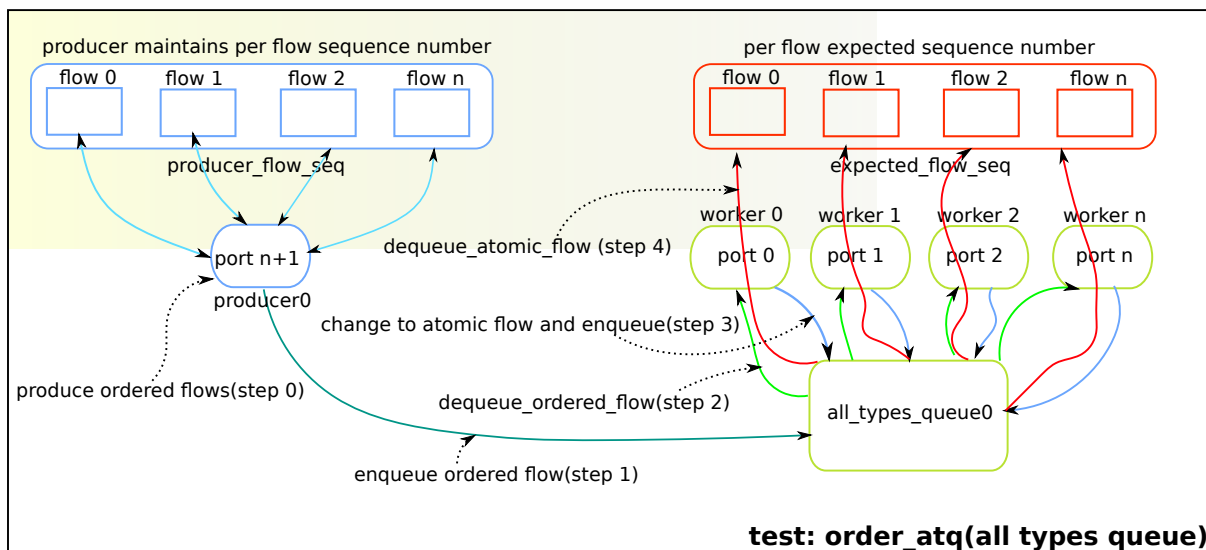
Fig. 9.2: order all types queue test operation.
