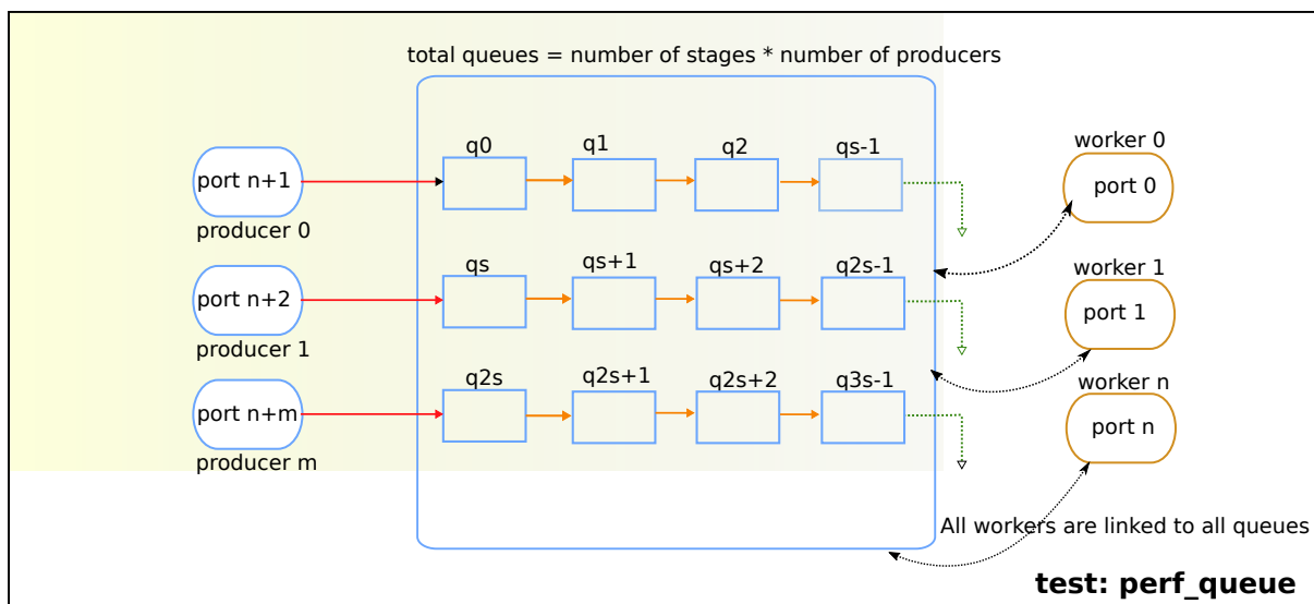
Fig. 9.3: perf queue test operation.
