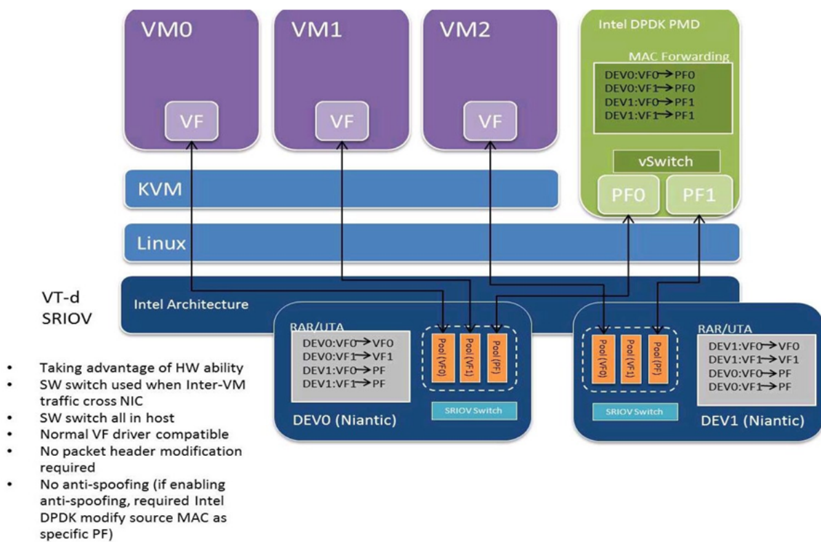
Fig. 27.4: Inter-VM Communication
