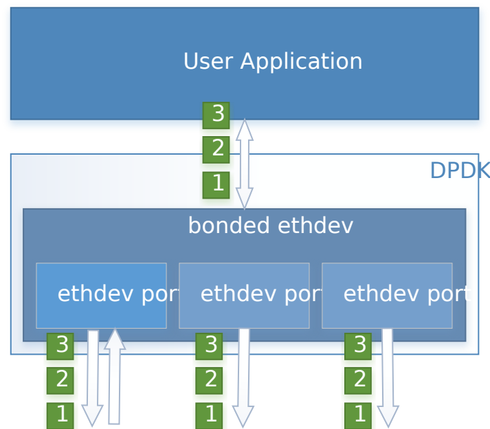
Fig. 20.5: Broadcast (Mode 3)
