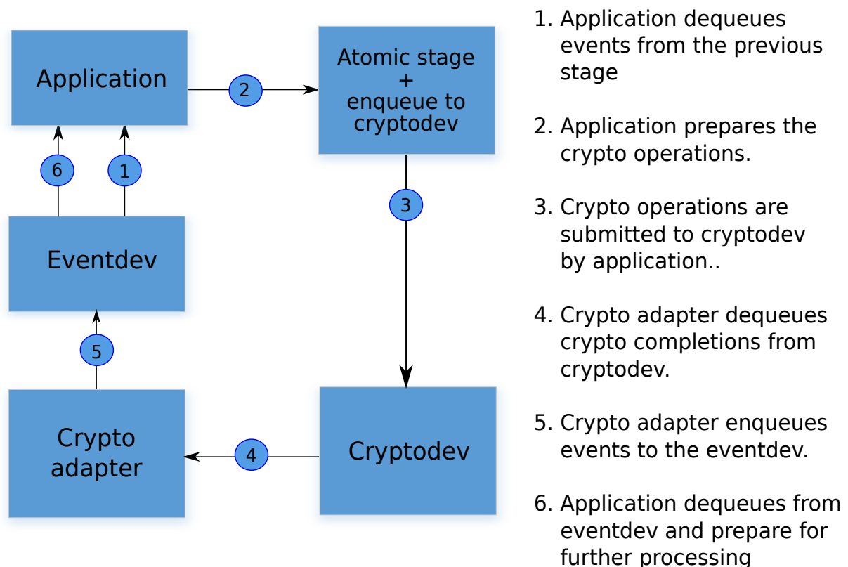
Fig. 41.1: Working model of RTE_EVENT_CRYPTOP_ADAPTER_OP_NEW mode
