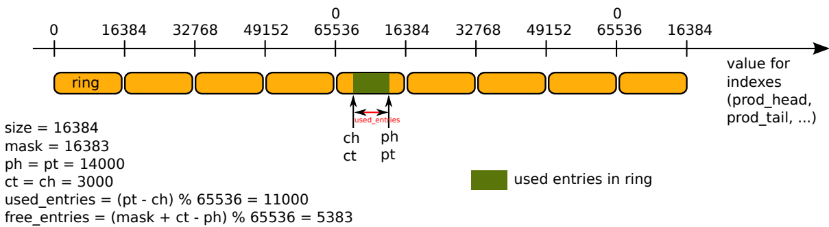
Fig. 6.13: Modulo 32-bit indexes - Example 1
