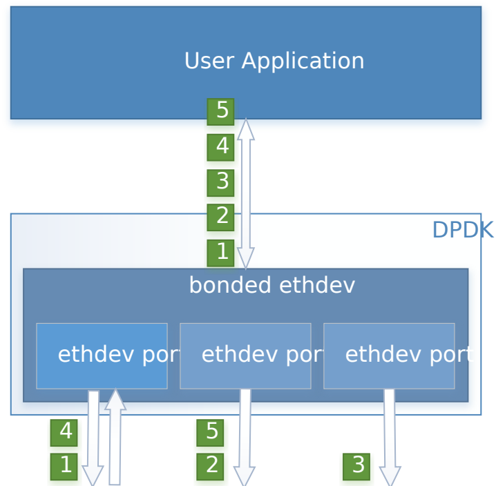
Fig. 20.2: Round-Robin (Mode 0)
