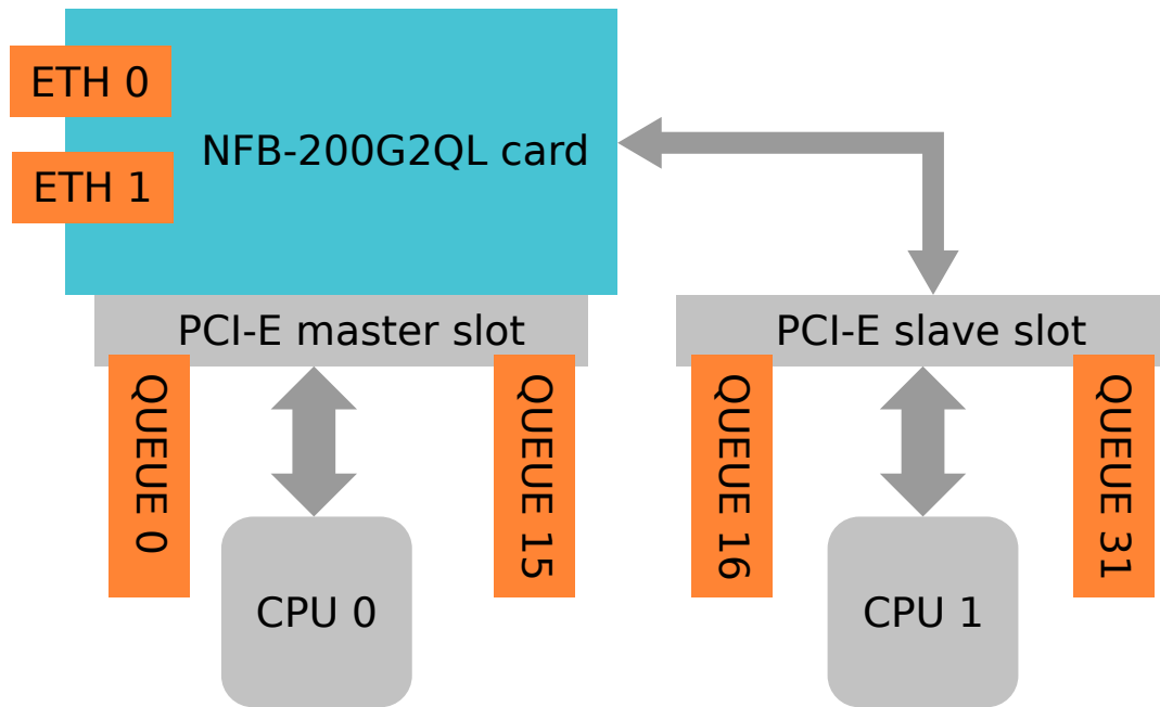
Fig. 47.1: NFB-200G2QL high-level diagram
