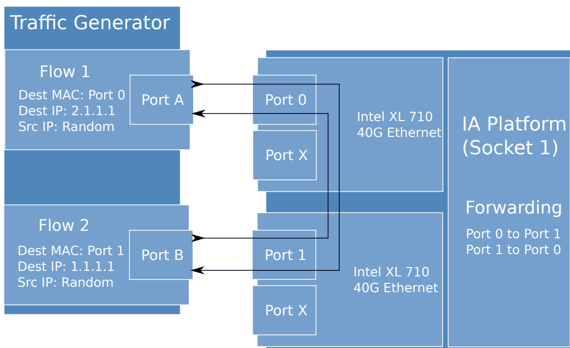
Fig. 23.1: Performance Test Setup
