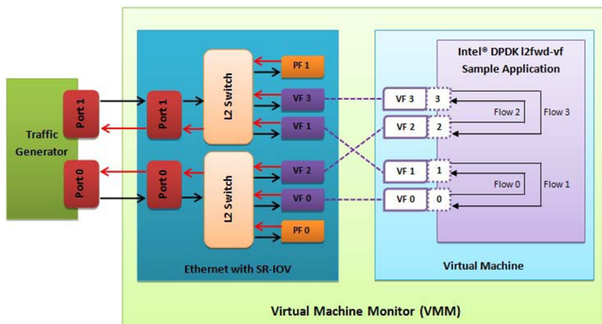
Fig. 27.2: Performance Benchmark Setup
