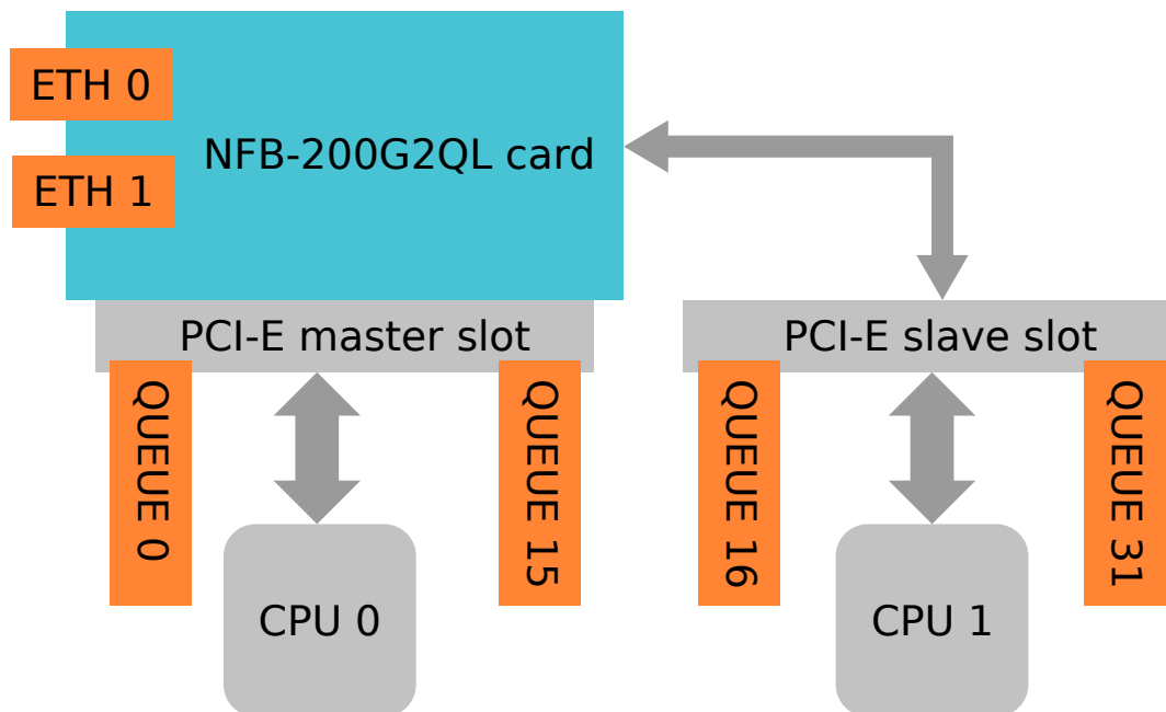
Fig. 38.1: NFB-200G2QL high-level diagram
