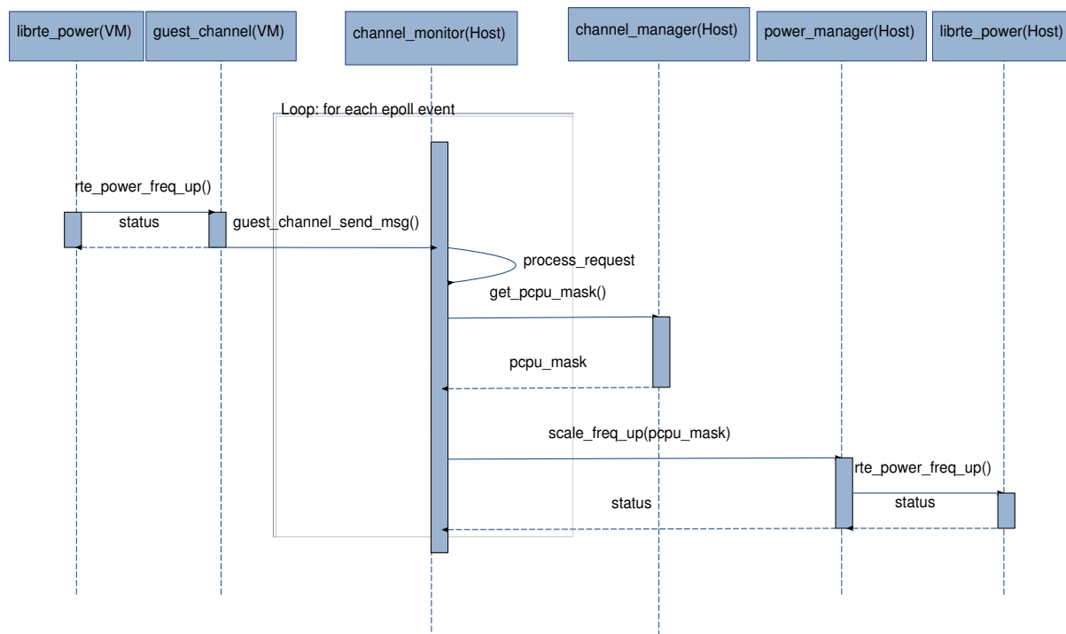
Fig. 32.2: VM request to scale frequency
