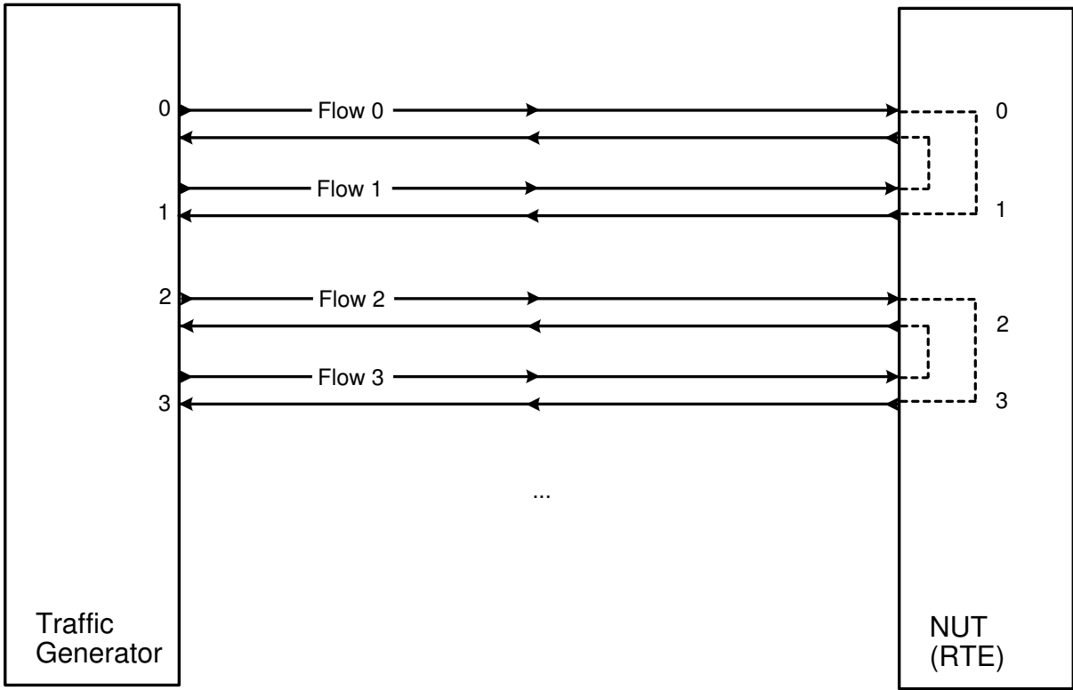
Fig. 11.1: Performance Benchmark Setup (Basic Environment)
