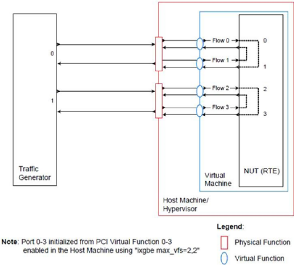
Fig. 11.2: Performance Benchmark Setup (Virtualized Environment)
