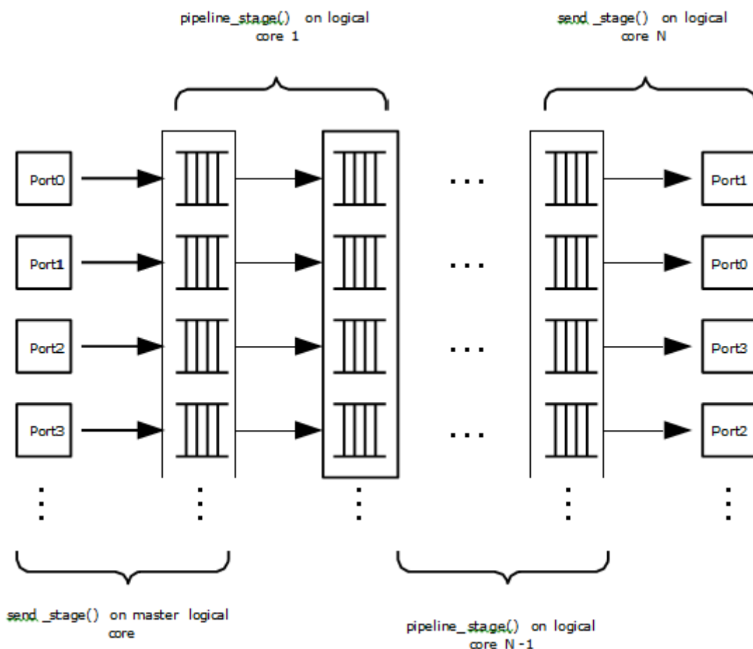
Fig. 23.3: Threads and Pipelines
