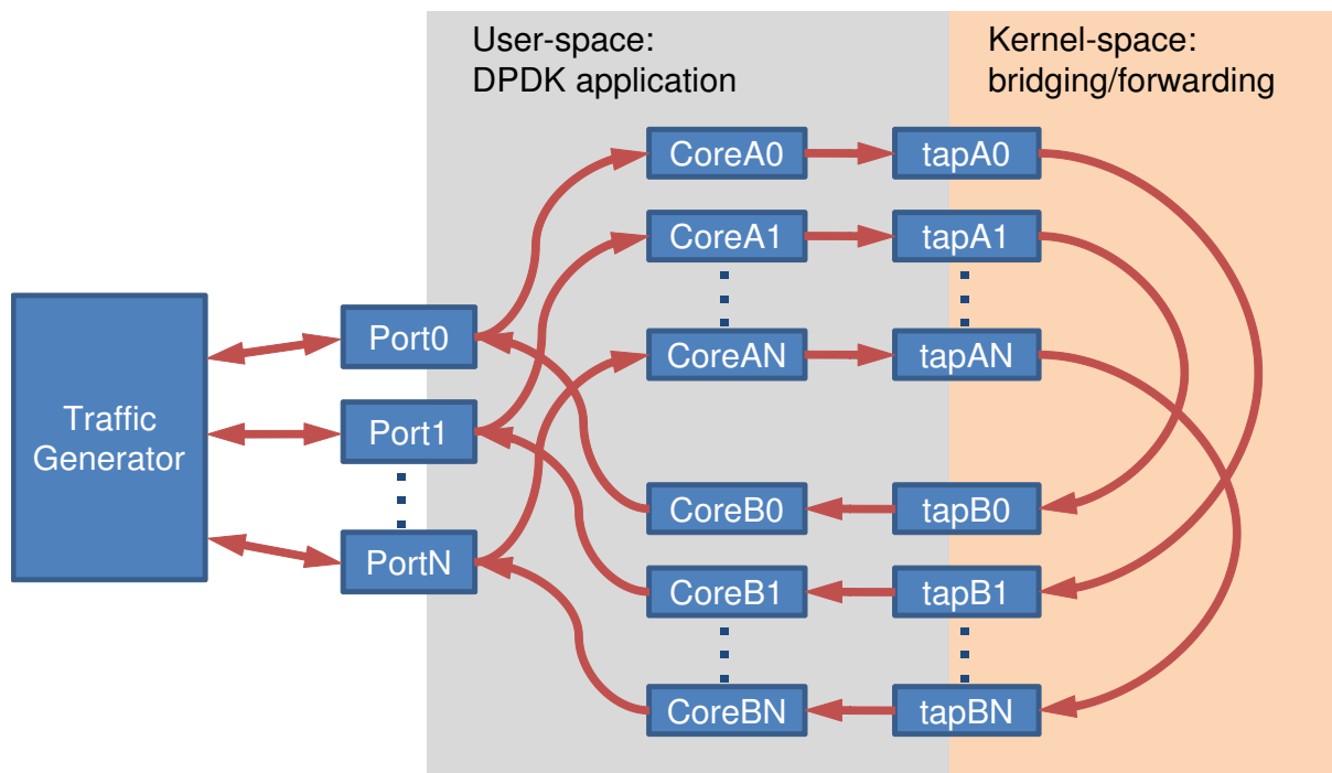
Fig. 3.1: Packet Flow
