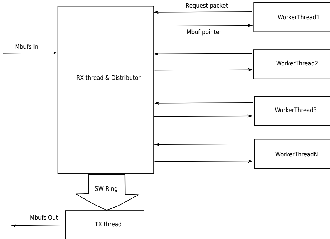
Fig. 31.2: Distributor Sample Application Layout
