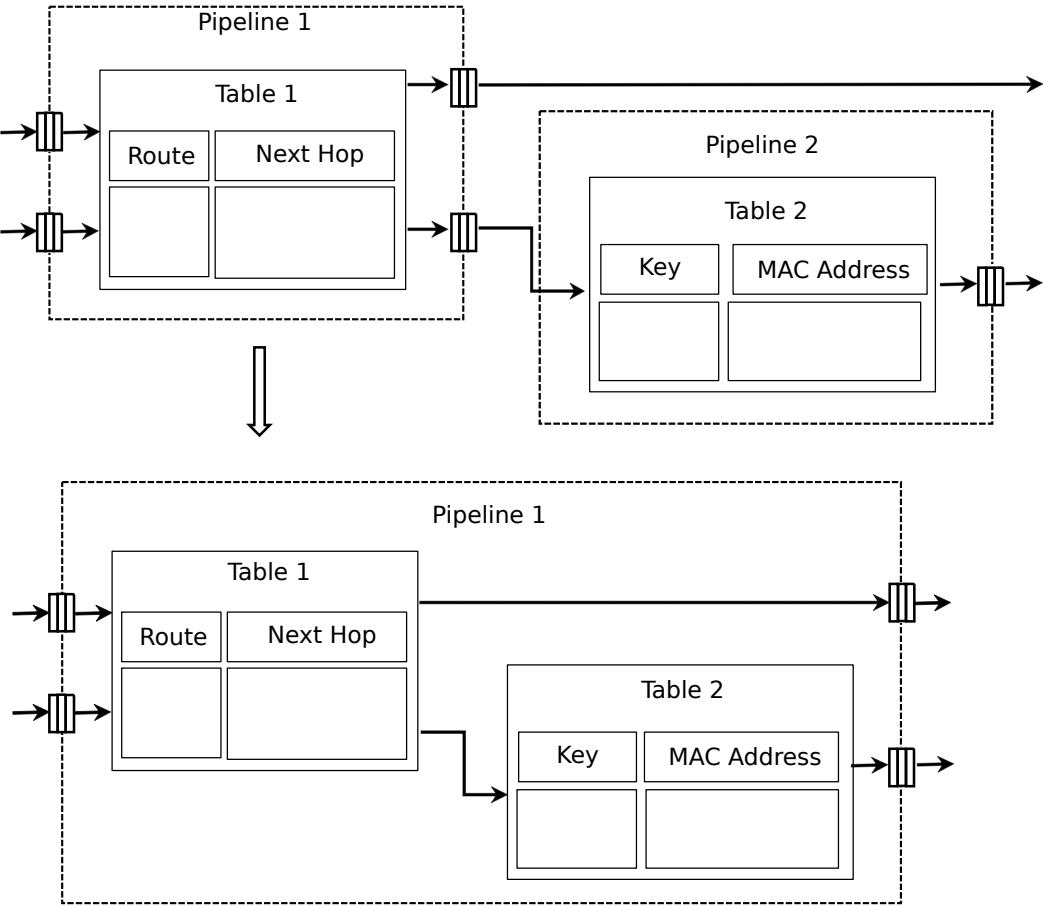
Fig. 29.2: Example of moving tables across different pipeline instances
