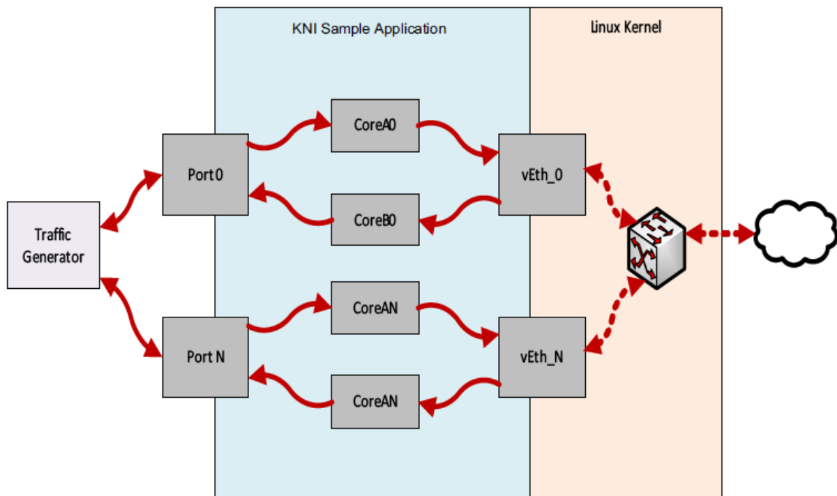
Fig. 10.1: Kernel NIC Application Packet Flow
