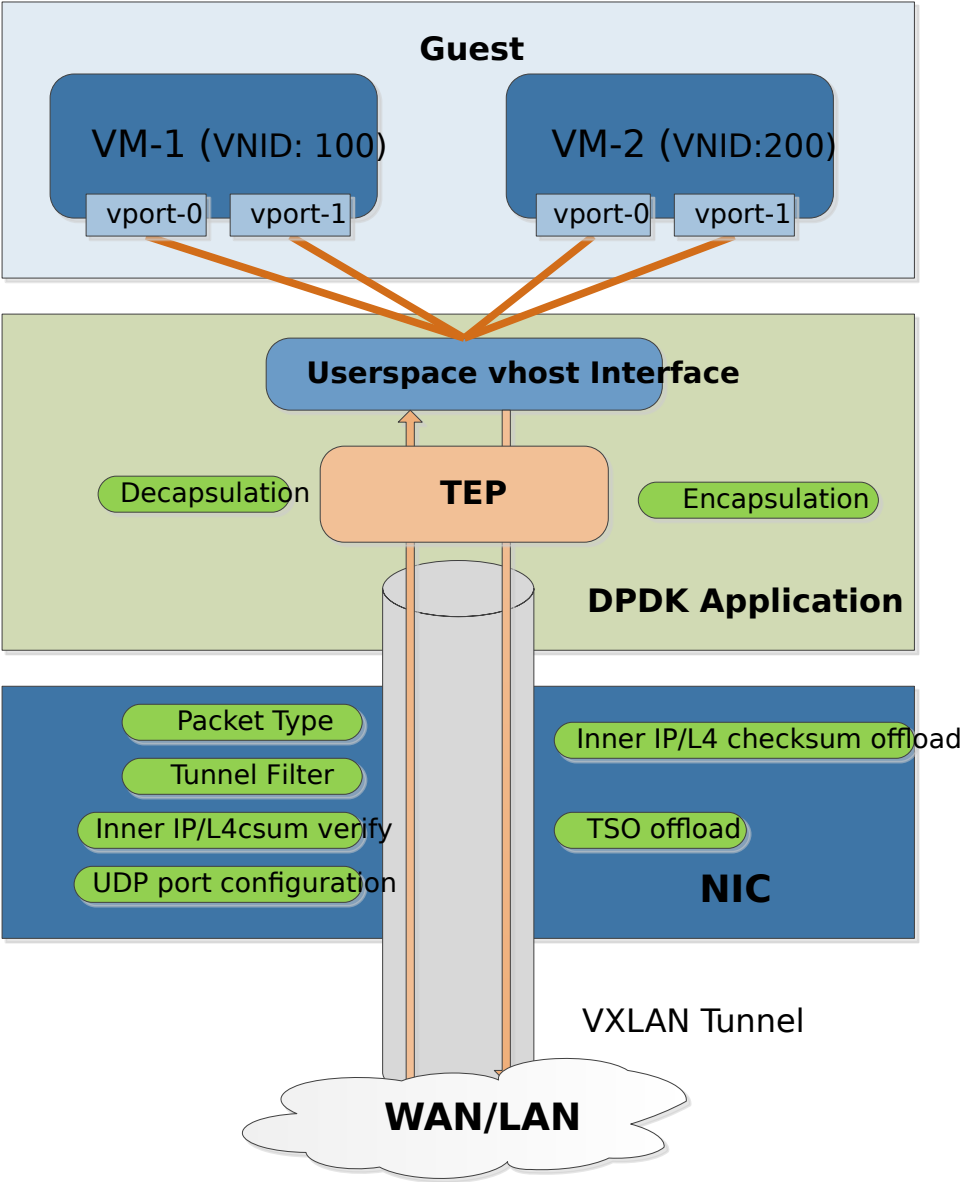
Fig. 33.2: TEP termination Framework Overview
