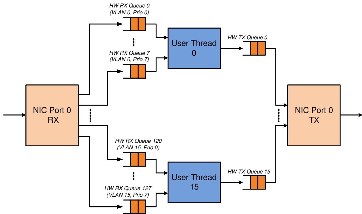
Fig. 26.1: Packet Flow Through the VMDQ and DCB Sample Application
