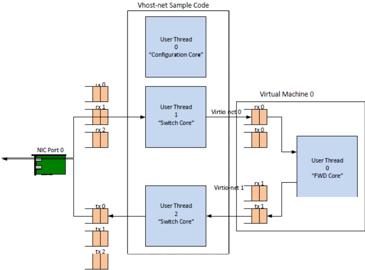
Fig. 27.4: Packet Flow Through the vhost-net Sample Application
