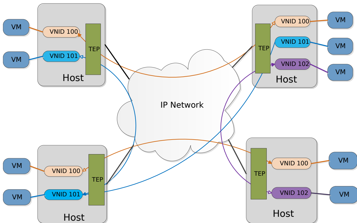
Fig. 33.1: Overlay Networking.
