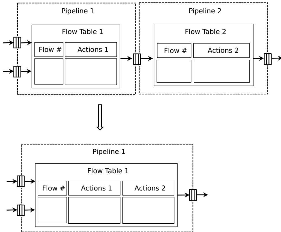
Fig. 29.3: Example of moving actions across different tables and pipeline instances
