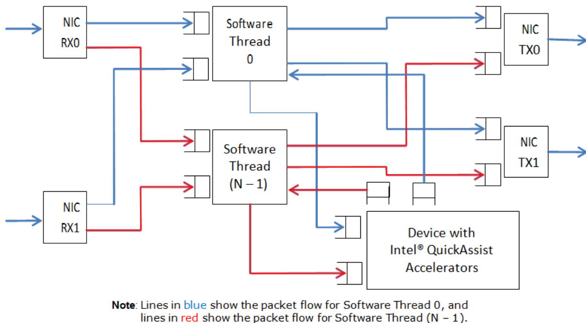
Fig. 22.1: Intel® QuickAssist Technology Application Block Diagram
