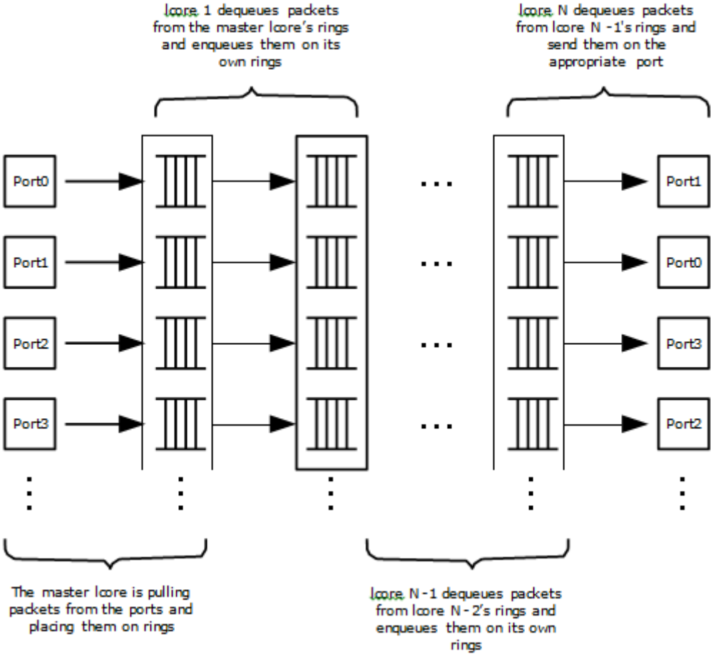
Fig. 23.1: Pipeline Overview
