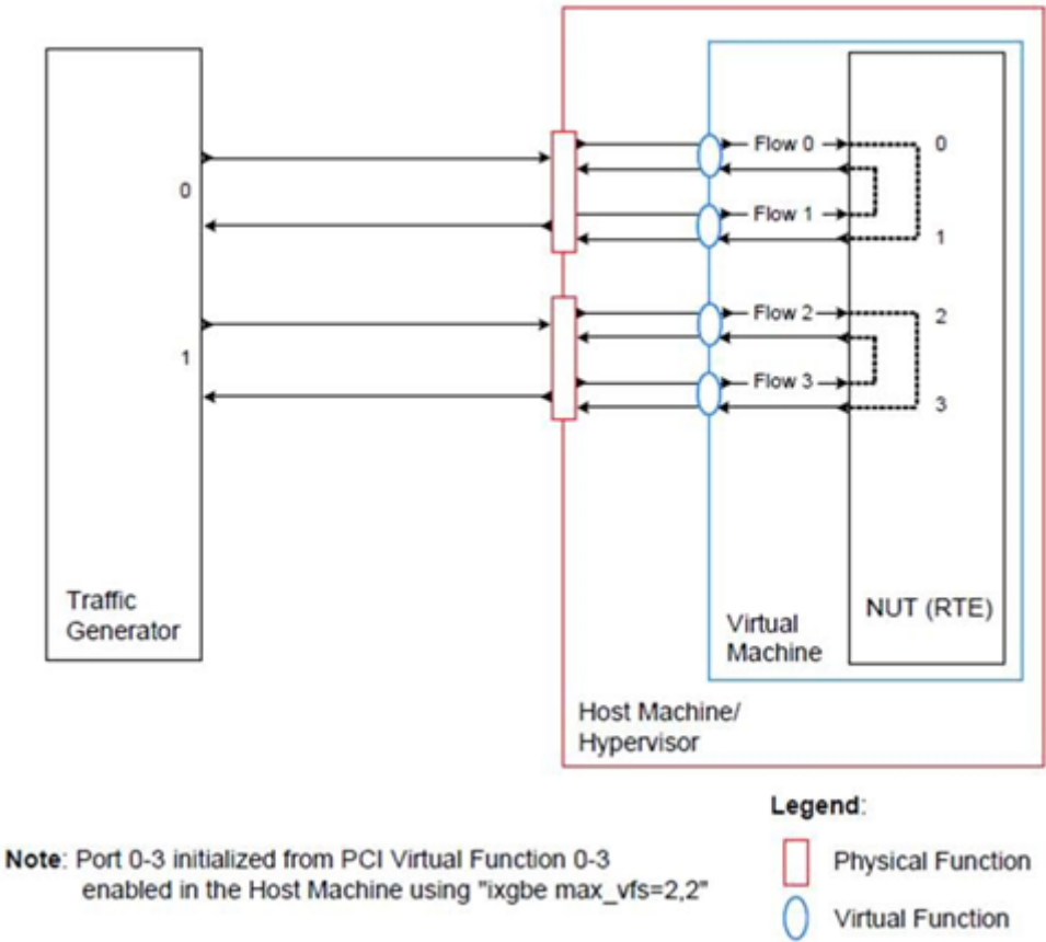
Fig. 12.2: Performance Benchmark Setup (Virtualized Environment)
