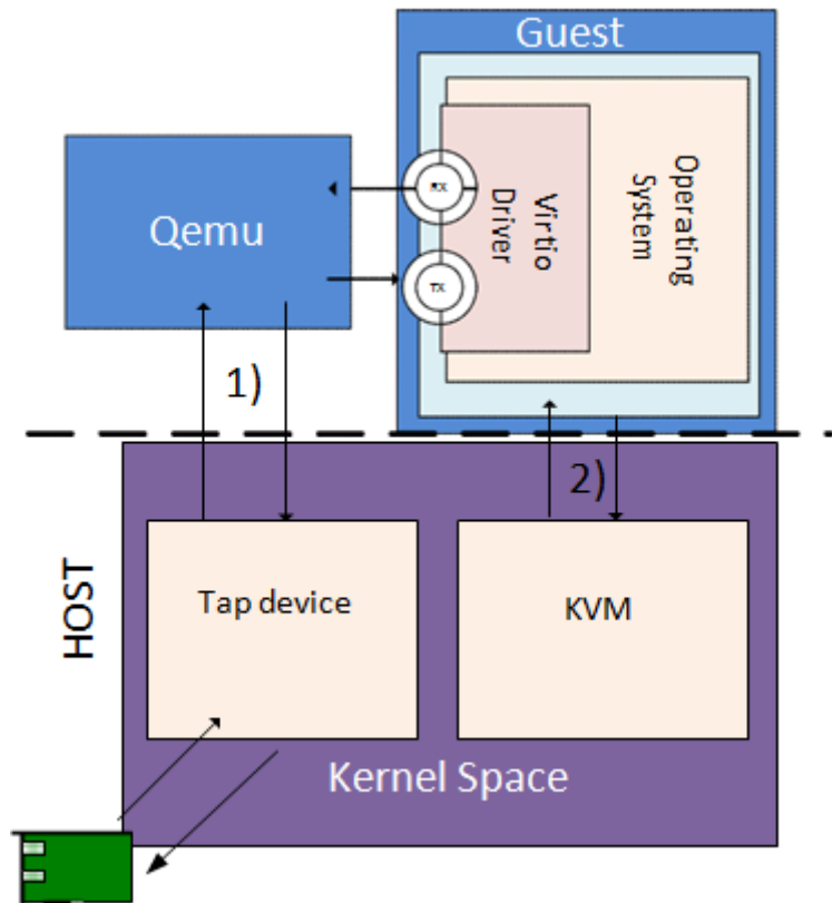
Fig. 27.1: System Architecture for Virtio-based Networking (virtio-net).
