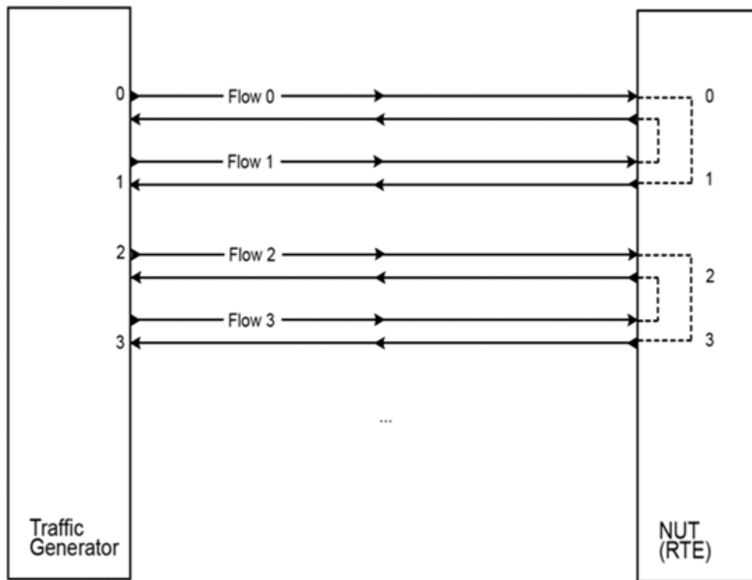
Fig. 23.2: Ring-based Processing Pipeline Performance Setup
