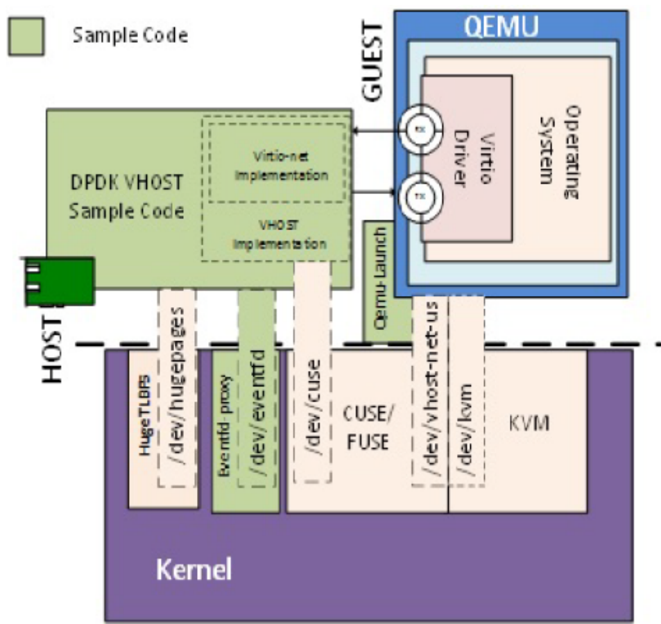
Fig. 27.3: Vhost-net Architectural Overview
