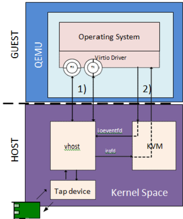
Fig. 27.2: Virtio with Linux
