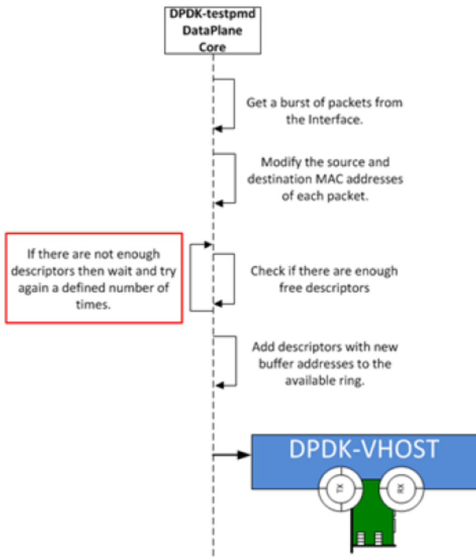
Fig. 27.5: Packet Flow on TX in DPDK-testpmd
