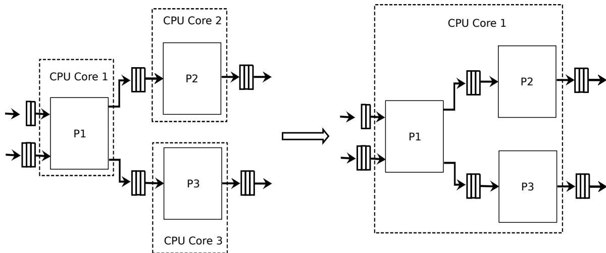
Fig. 29.1: Example of moving pipeline instances across different CPU cores
