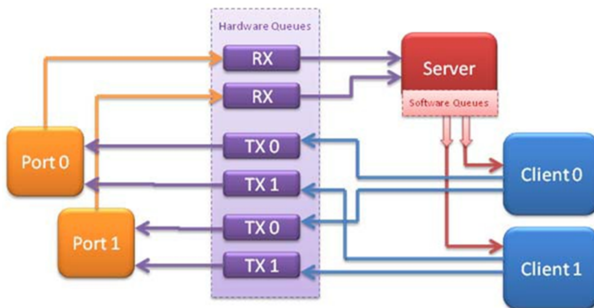
Fig. 19.2: Example Data Flow in a Client-Server Symmetric Multi-process Application
