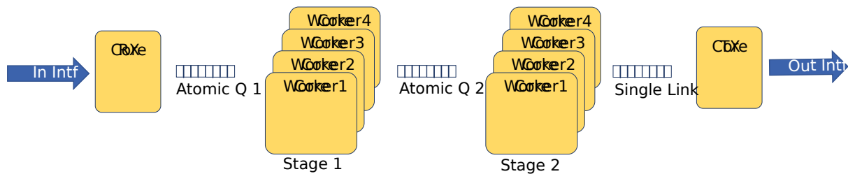
Fig. 38.1: Sample eventdev usage, with RX, two atomic stages and a single-link to TX.
