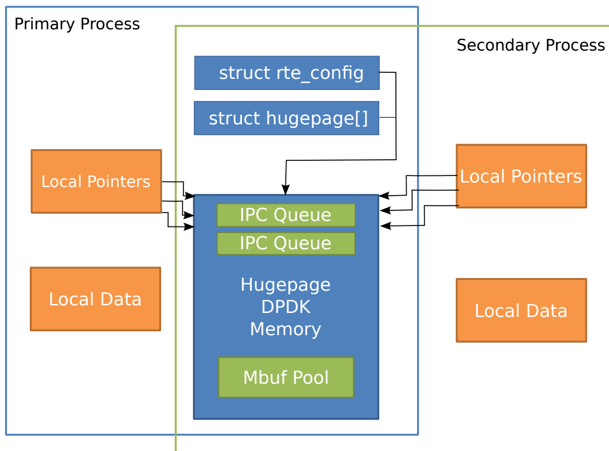
Fig. 35.1: Memory Sharing in the DPDK Multi-process Sample Application
