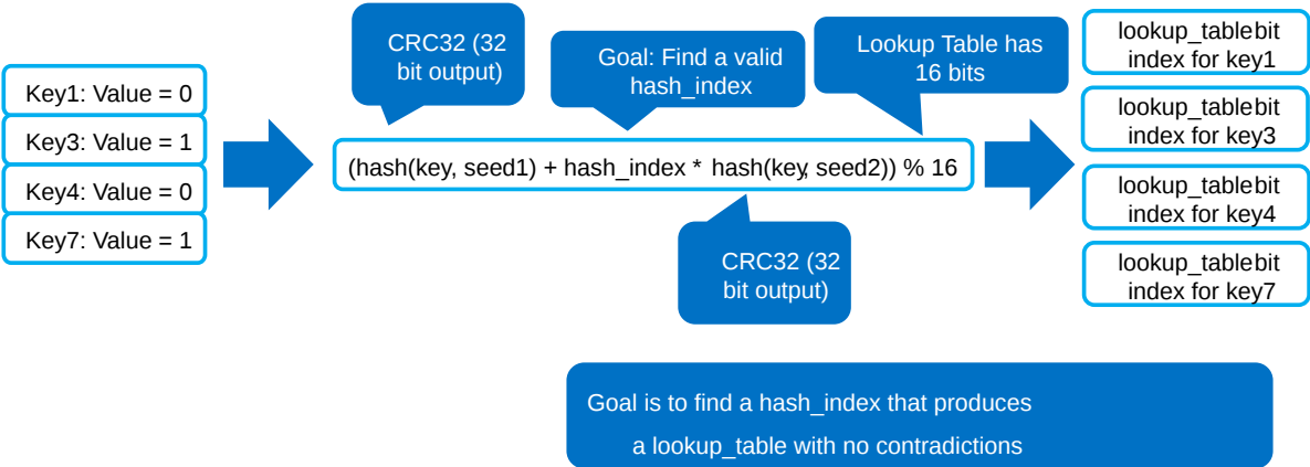
Fig. 24.9: Perfect Hash Search - Satisfy Target Values
