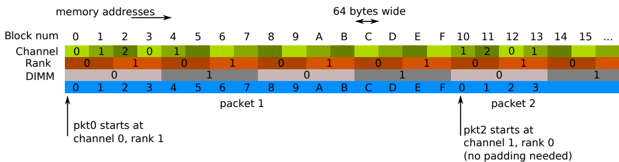
Fig. 9.2: Three Channels and Two Dual-ranked DIMM Example
