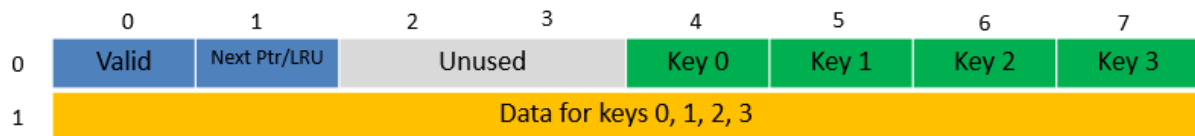
Fig. 46.5: Data Structures for 8-byte Key Hash Tables
