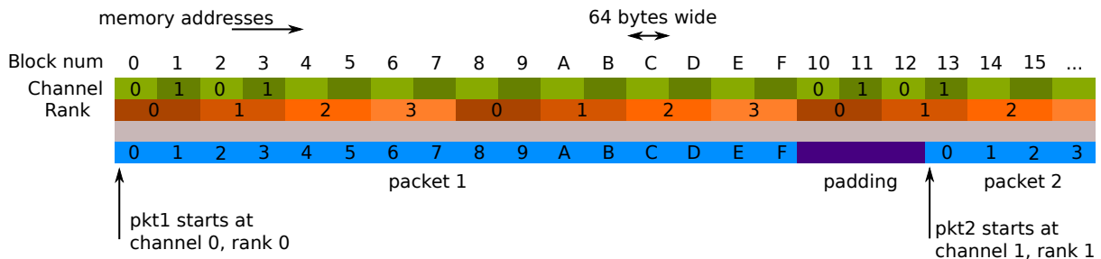
Fig. 9.1: Two Channels and Quad-ranked DIMM Example
