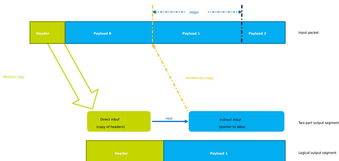
Fig. 33.1: Two-part GSO output segment
