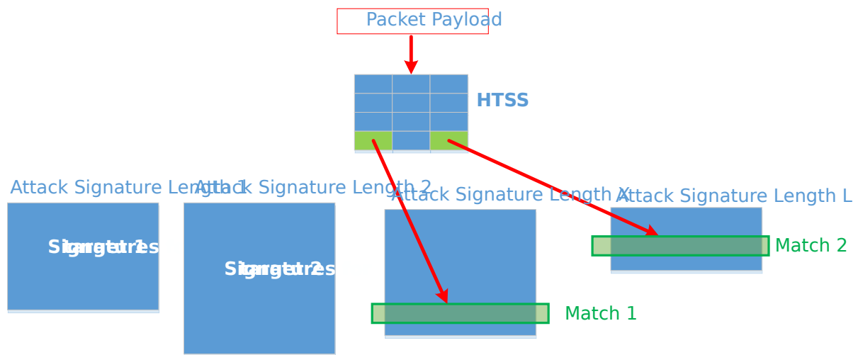
Fig. 25.6: Using HTSS for Attack Signature Matching
