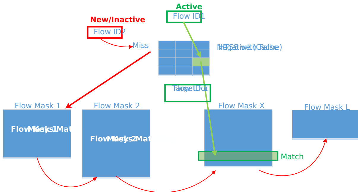
Fig. 25.7: Using HTSS with False Negatives for Wild Card Classification
