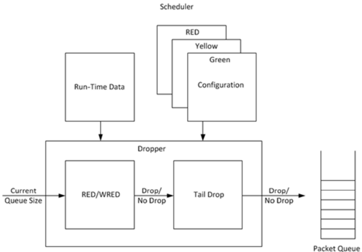
Fig. 43.7: High-level Block Diagram of the DPDK Dropper
