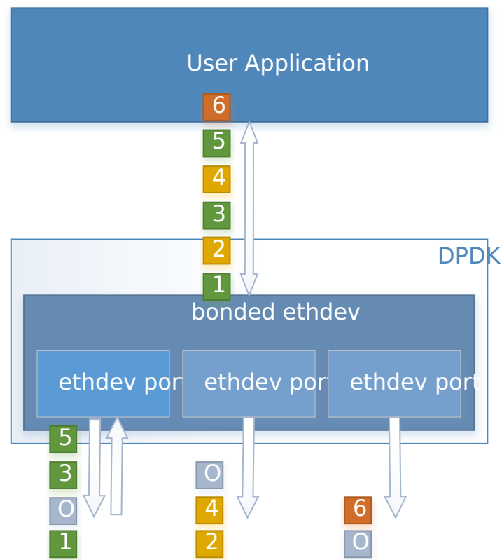
Fig. 21.6: Link Aggregation 802.3AD (Mode 4)
