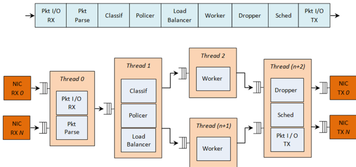
Fig. 43.1: Complex Packet Processing Pipeline with QoS Support
