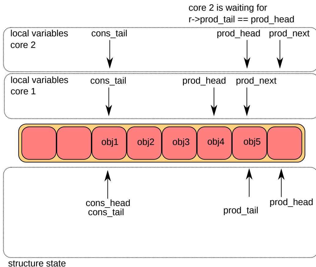
Fig. 7.11: Multiple producer enqueue fourth step
