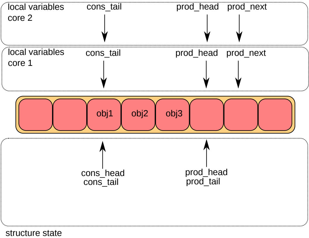
Fig. 7.8: Multiple producer enqueue first step
