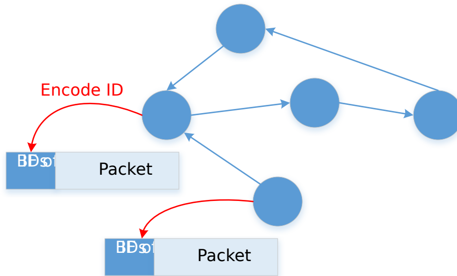
Fig. 25.3: Detecting Routing Loops Using BF
