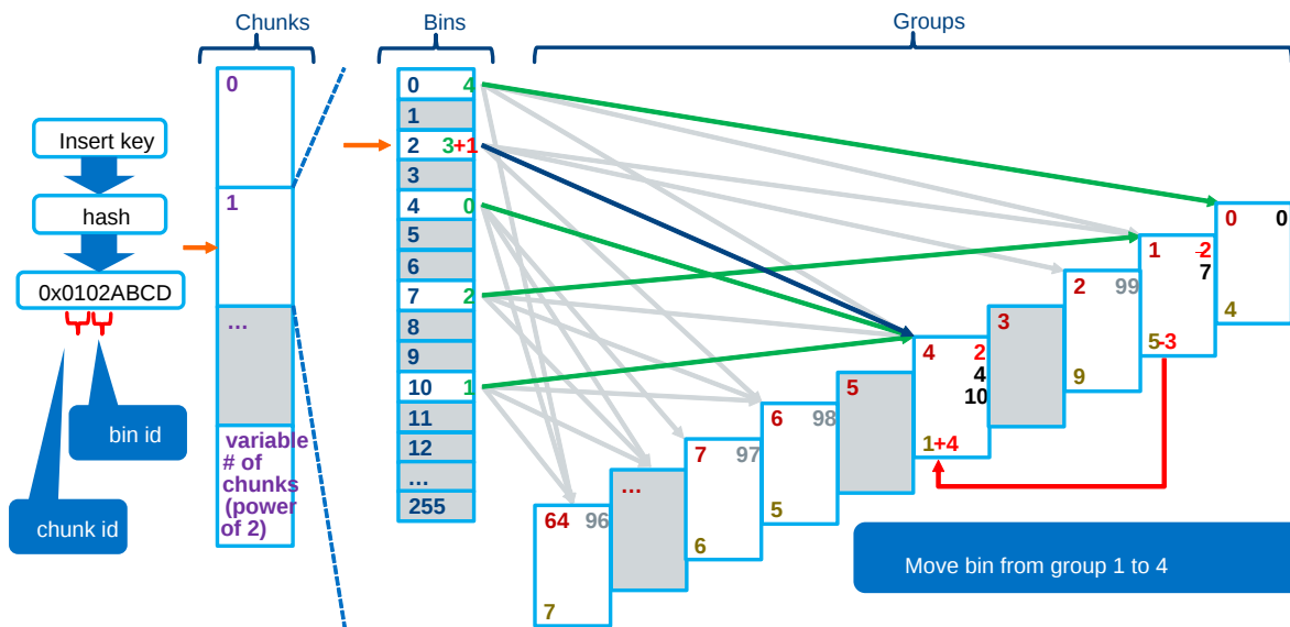
Fig. 24.12: Runtime Group Rebalancing
