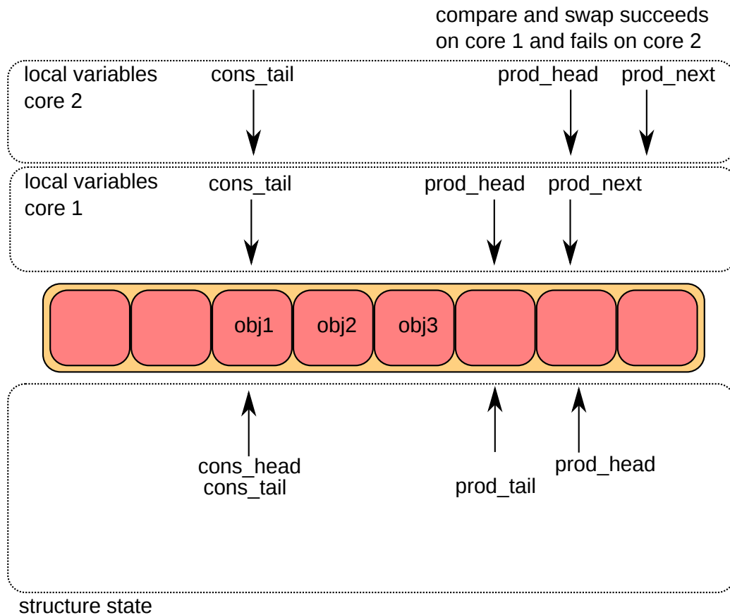
Fig. 7.9: Multiple producer enqueue second step
