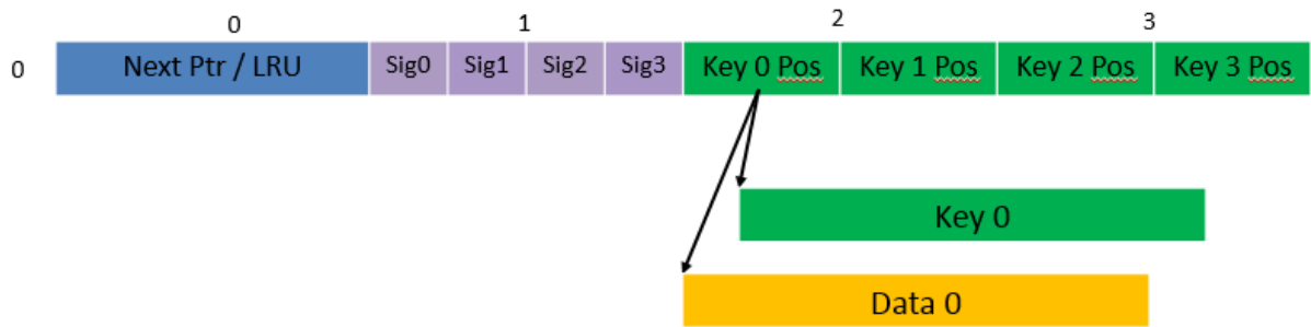
Fig. 46.3: Data Structures for Configurable Key Size Hash Tables
