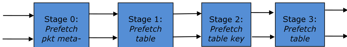
Fig. 46.4: Bucket Search Pipeline for Key Lookup Operation (Configurable Key Size Hash Tables)
