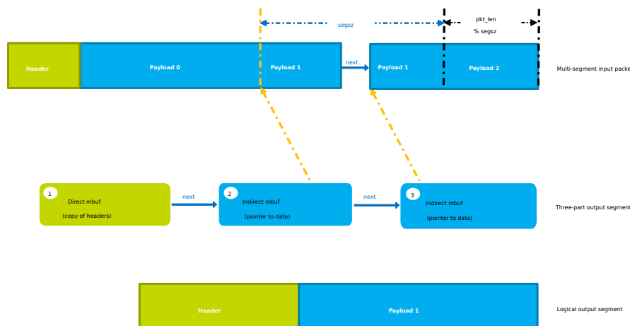
Fig. 33.2: Three-part GSO output segment
