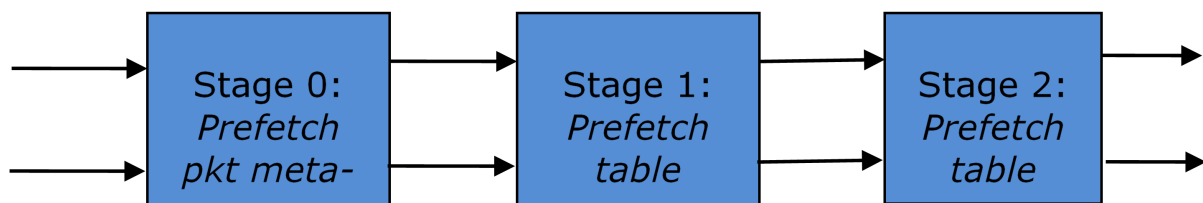
Fig. 46.7: Bucket Search Pipeline for Key Lookup Operation (Single Key Size Hash Tables)
