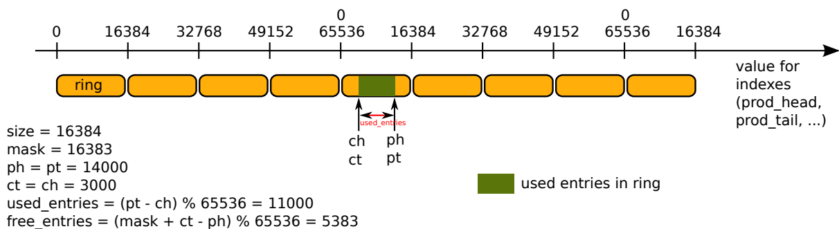
Fig. 7.13: Modulo 32-bit indexes - Example 1
