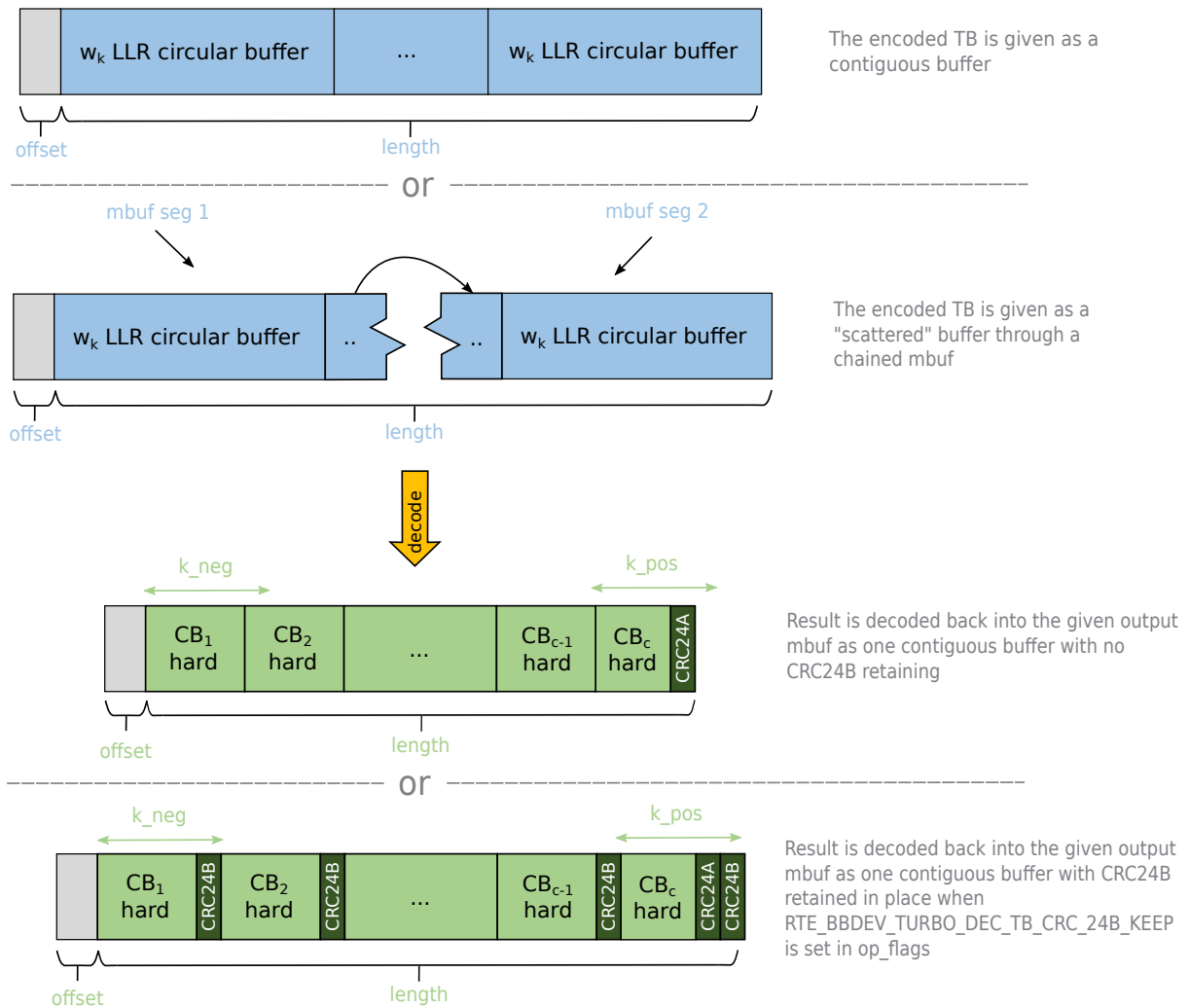
Fig. 16.2: Turbo decoding of Code Blocks in mbuf structure
