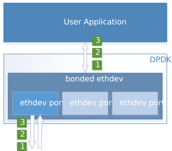
Fig. 21.3: Active Backup (Mode 1)
