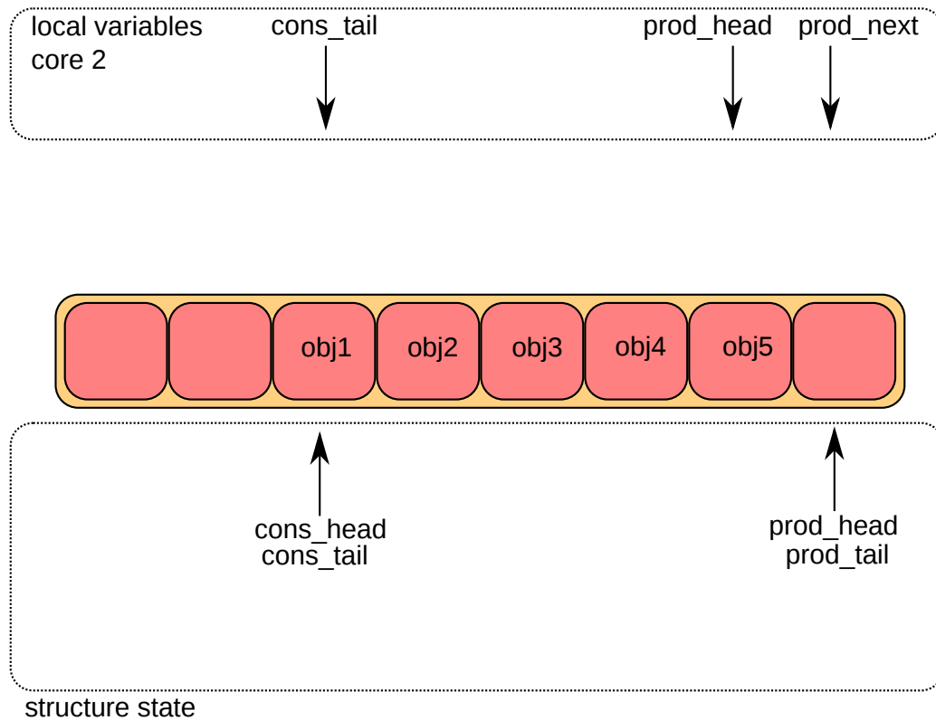
Fig. 7.12: Multiple producer enqueue last step
