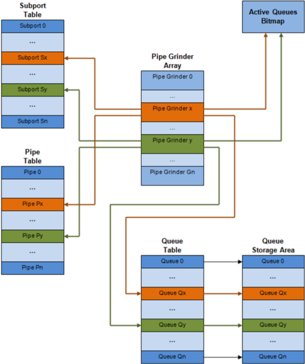
Fig. 43.4: Internal Data Structures per Port
