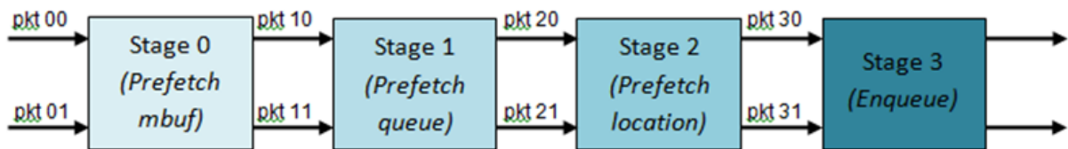
Fig. 43.5: Prefetch Pipeline for the Hierarchical Scheduler Enqueue Operation
