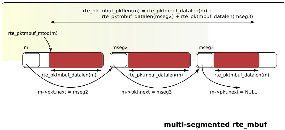
Fig. 10.2: An mbuf with Three Segments
