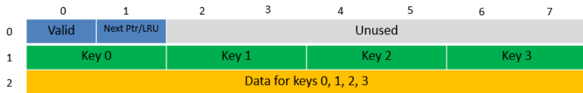
Fig. 46.6: Data Structures for 16-byte Key Hash Tables
