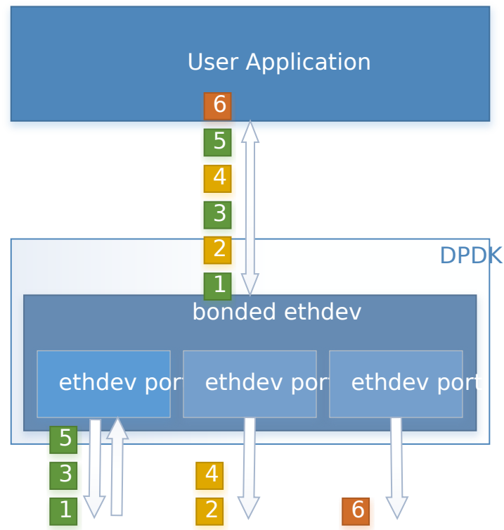
Fig. 21.4: Balance XOR (Mode 2)
