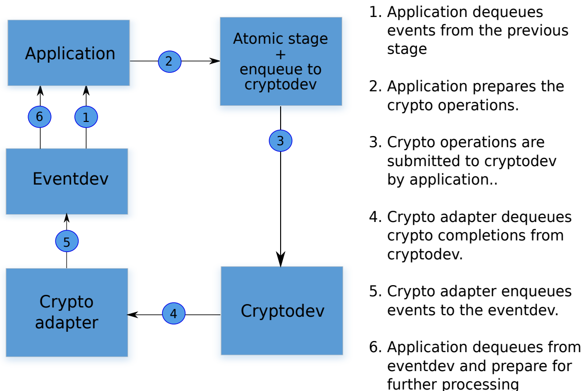
Fig. 42.1: Working model of RTE_EVENT_CRYPTOP_ADAPTER_OP_NEW mode
