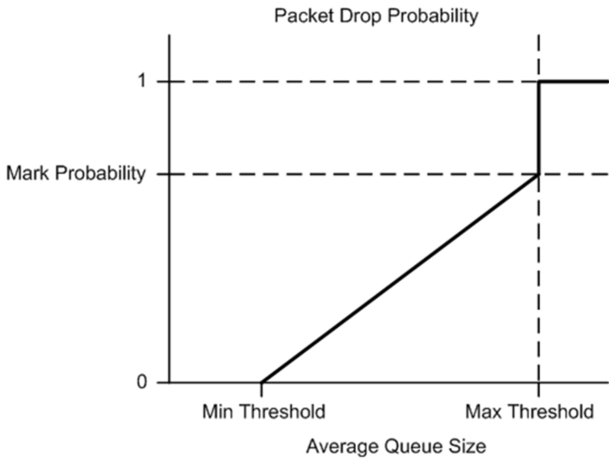
Fig. 43.10: Packet Drop Probability for a Given RED Configuration
