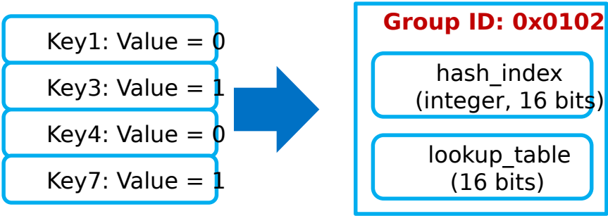
Fig. 24.8: Perfect Hash Search - Assigned Keys & Target Value
