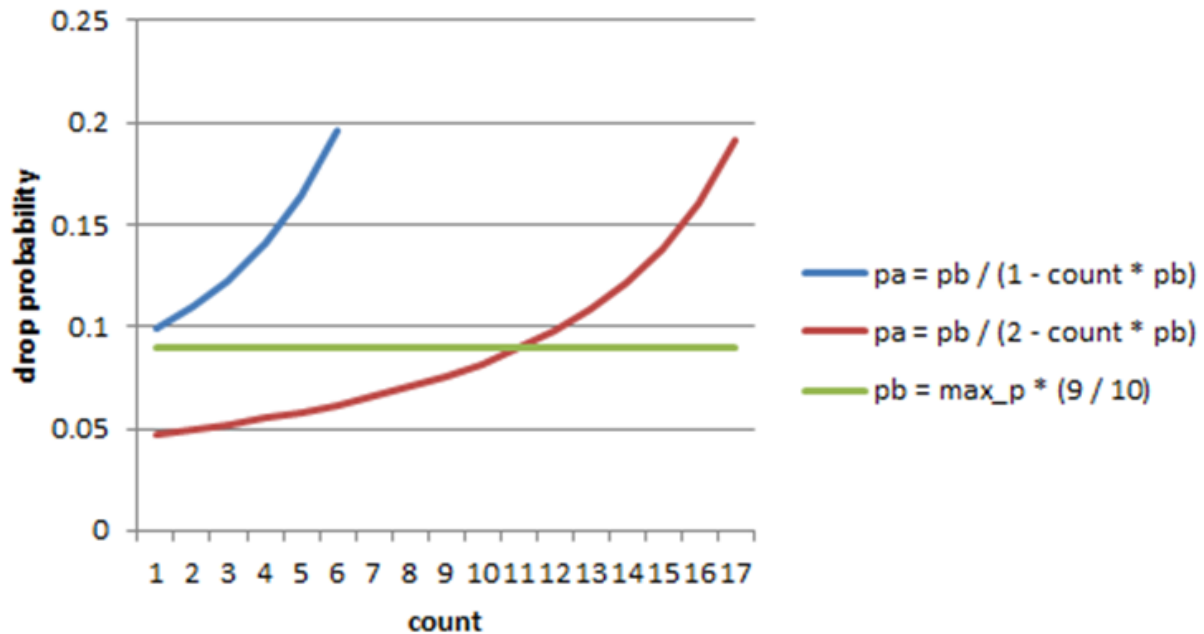
Fig. 43.11: Initial Drop Probability (pb), Actual Drop probability (pa) Computed Using a Factor 1 (Blue Curve) and a Factor 2 (Red Curve)
