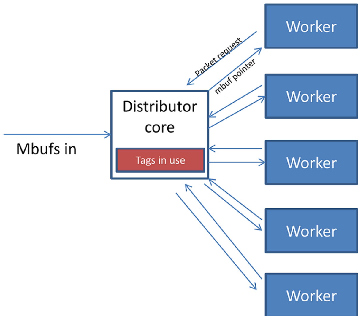
Fig. 29.1: Packet Distributor mode of operation
