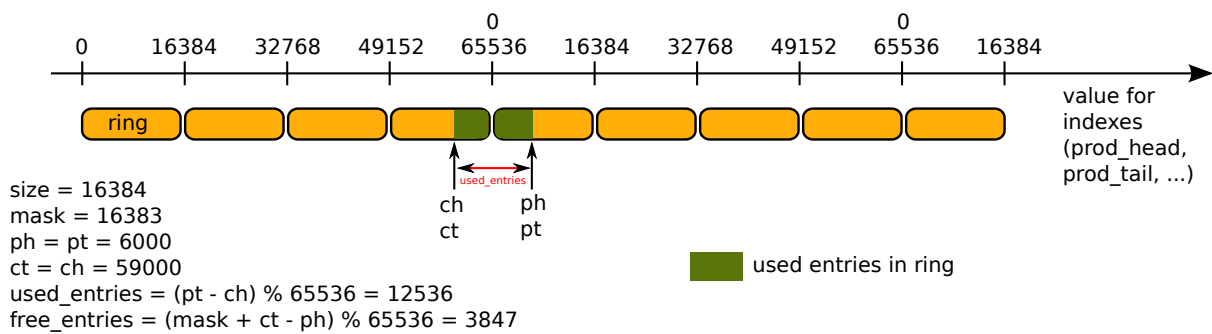
Fig. 7.14: Modulo 32-bit indexes - Example 2
