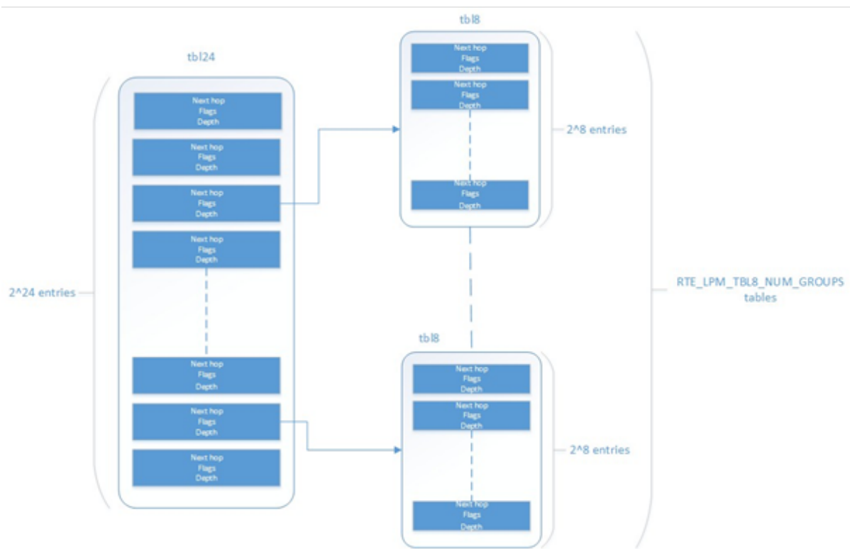
Fig. 26.1: Table split into different levels
