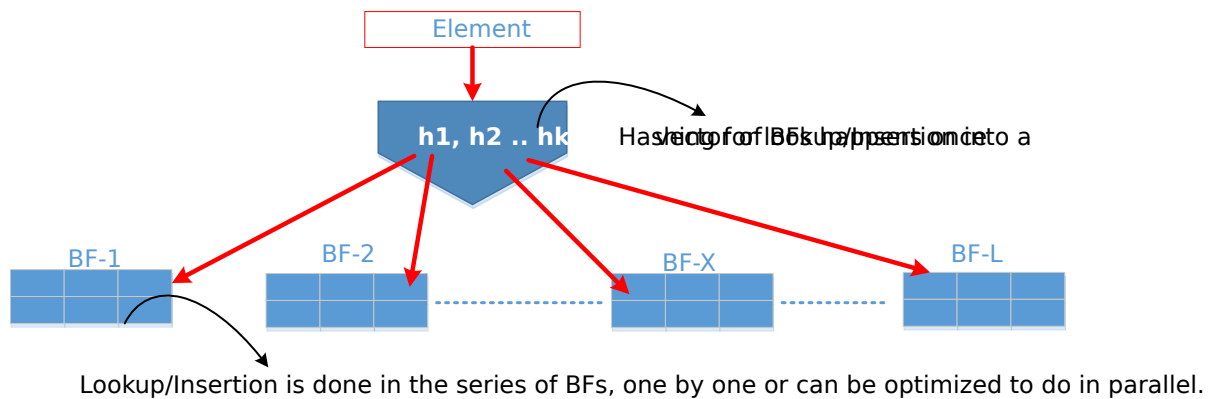
Fig. 25.4: Vector Bloom Filter (vBF) Overview
