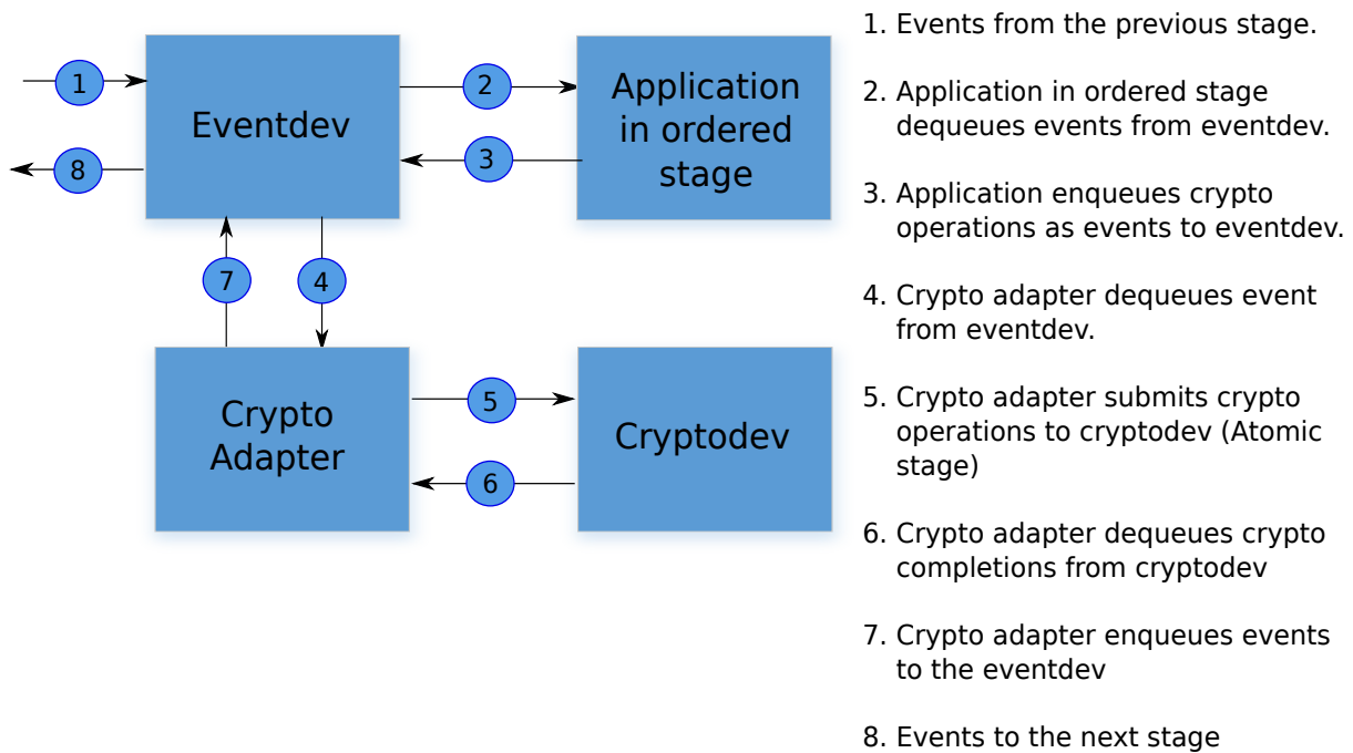
Fig. 42.2: Working model of RTE_EVENT_CRYPTOP_ADAPTER_OP_FORWARD mode
