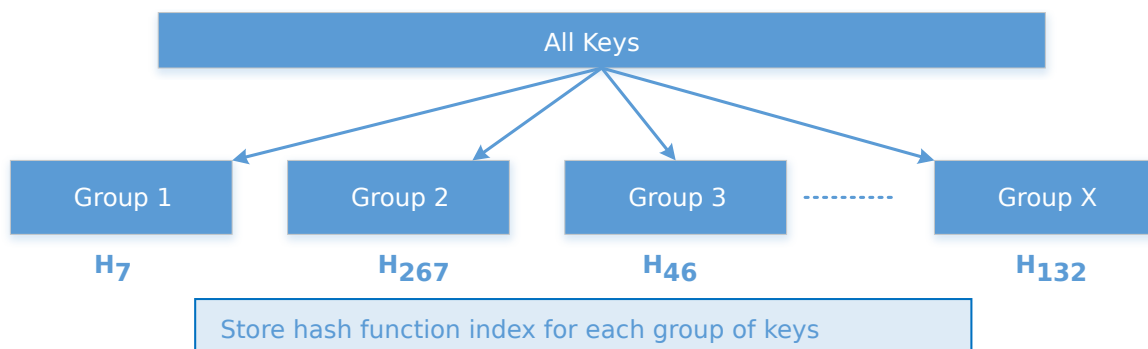
Fig. 24.5: Divide and Conquer for Millions of Keys
