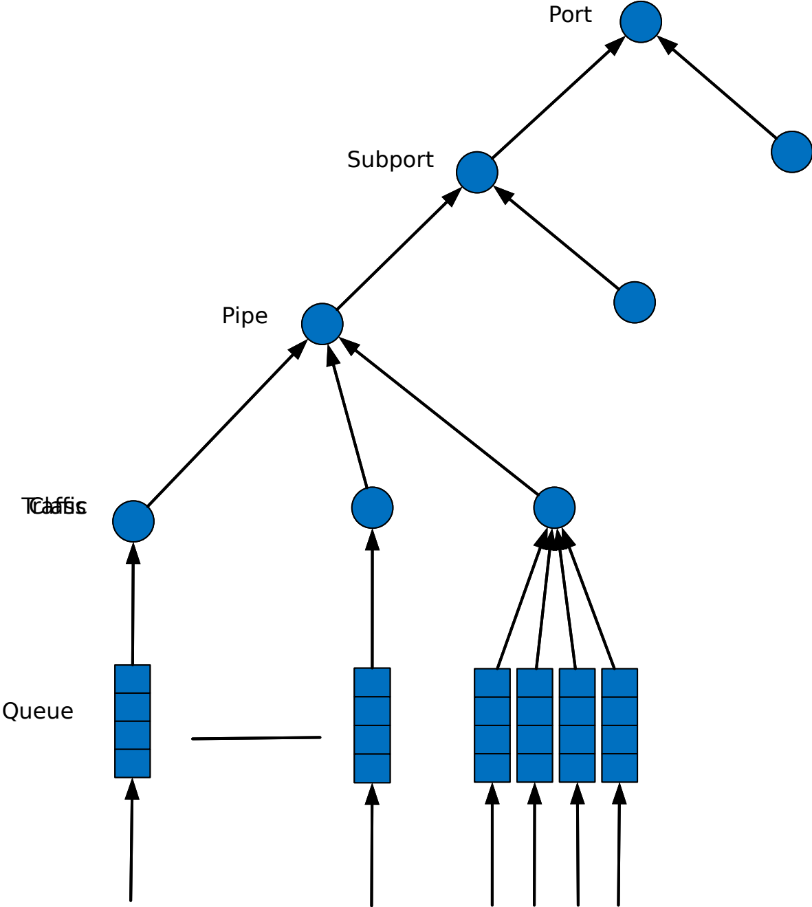
Fig. 43.3: Scheduling Hierarchy per Port
