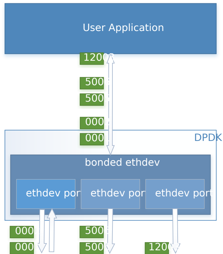
Fig. 21.7: Transmit Load Balancing (Mode 5)
