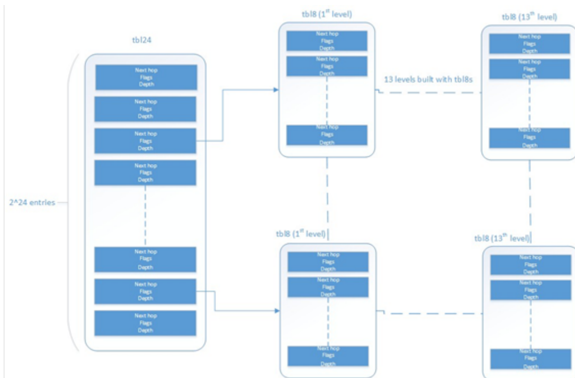
Fig. 27.1: Table split into different levels
