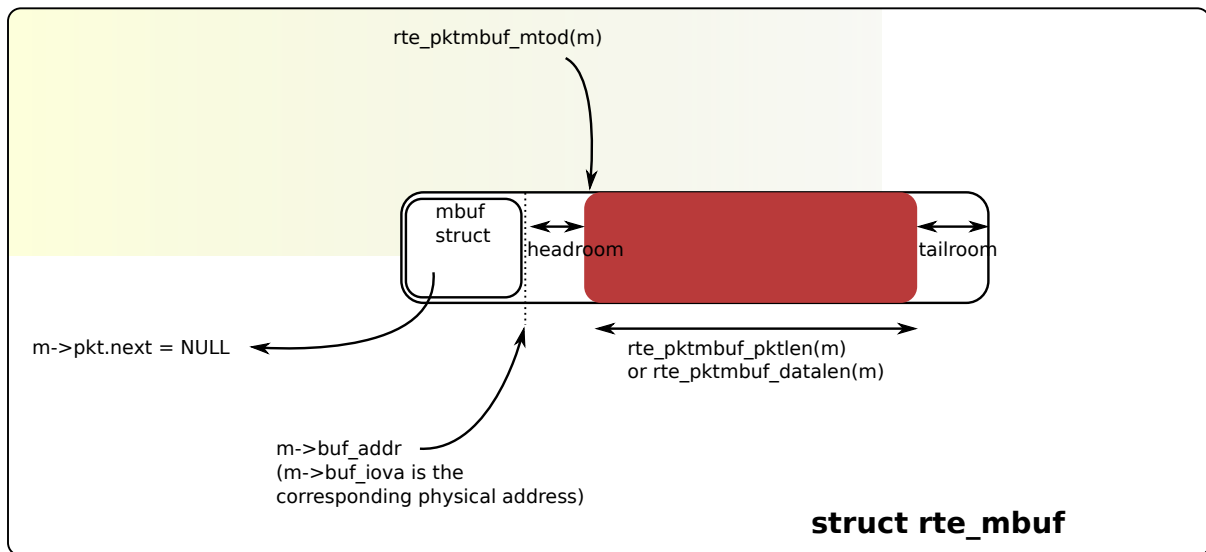
Fig. 10.1: An mbuf with One Segment
