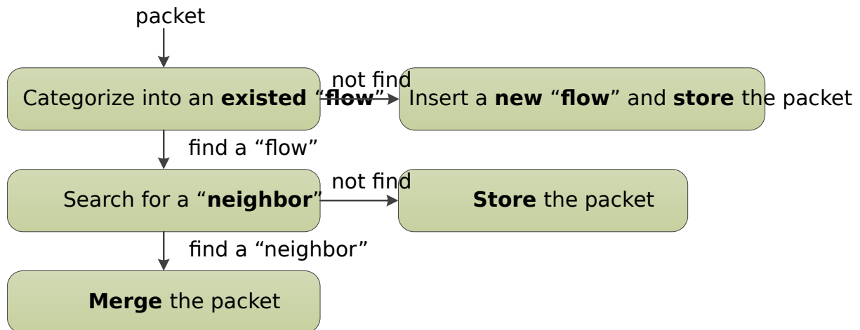
Fig. 32.1: Key-based Reassembly Algorithm
