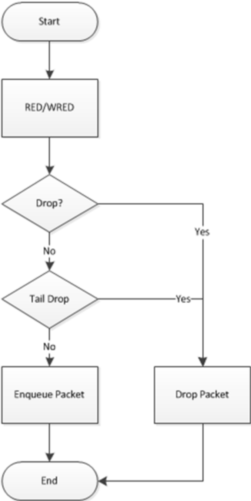
Fig. 43.8: Flow Through the Dropper
