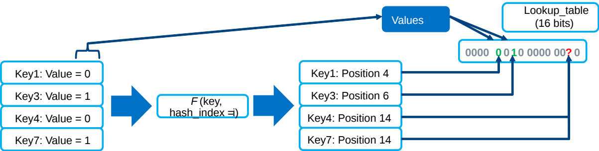
Fig. 24.10: Finding Hash Index for Conflict Free lookup_table
