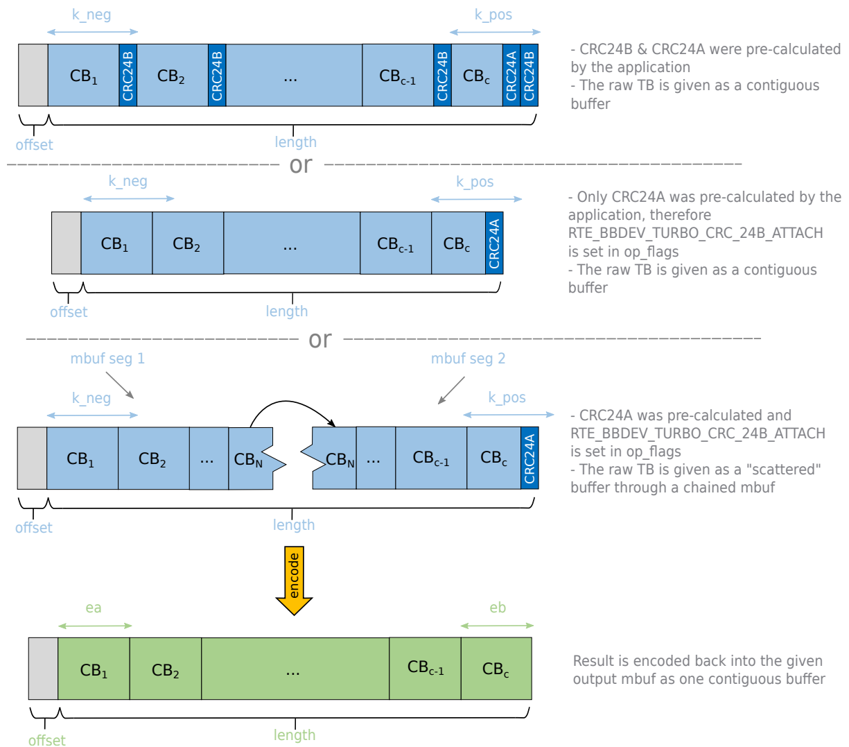
Fig. 16.1: Turbo encoding of Code Blocks in mbuf structure
