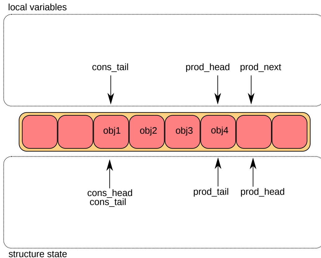
Fig. 7.3: Enqueue second step
