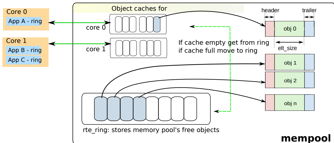
Fig. 9.3: A mempool in Memory with its Associated Ring
