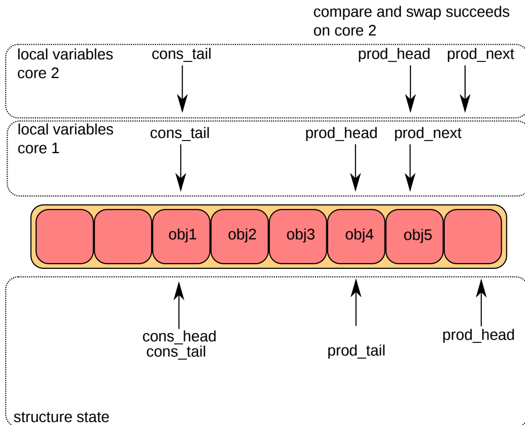
Fig. 7.10: Multiple producer enqueue third step
